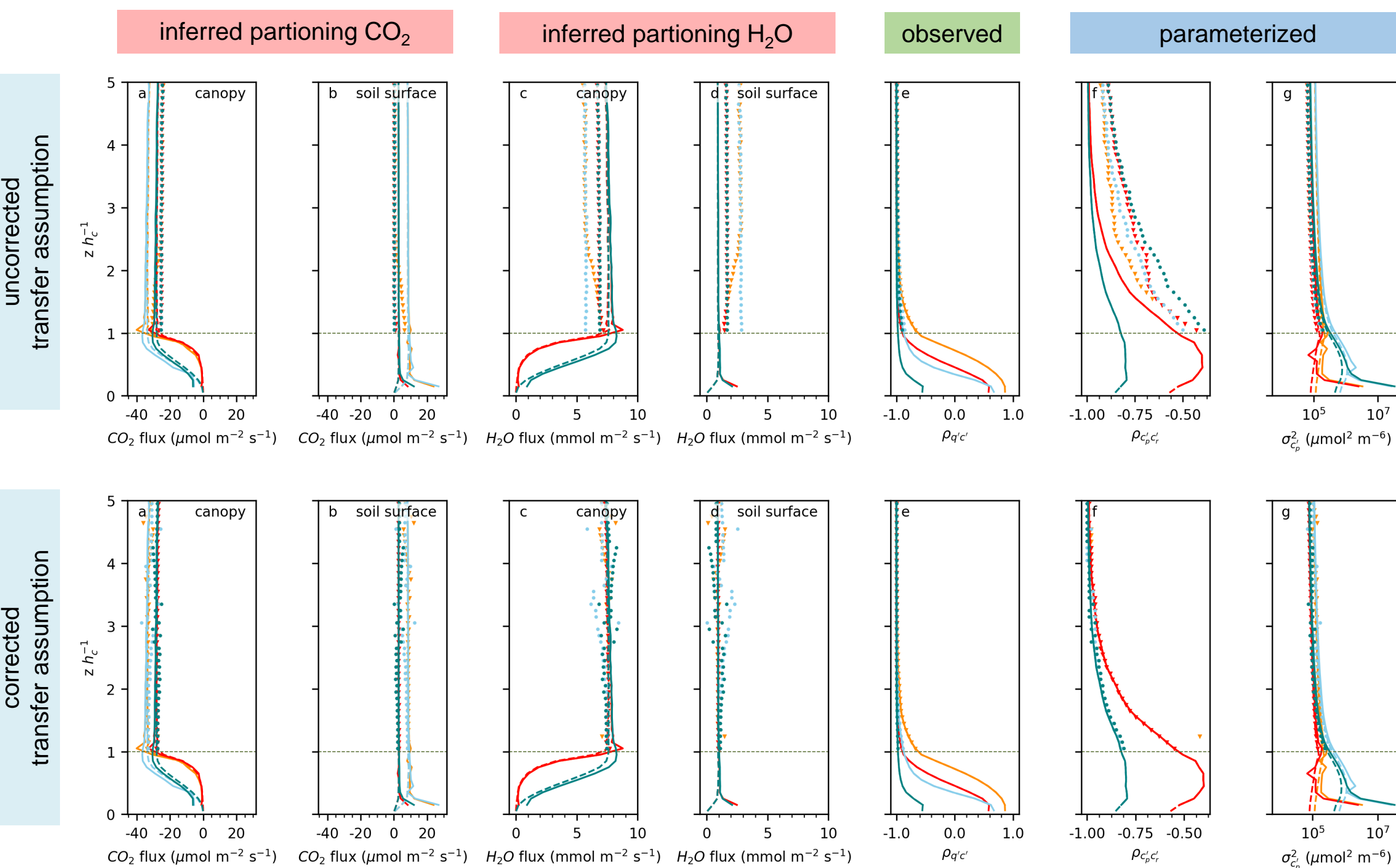
Fig.4: Vertical profiles of inferred H 2 O and CO 2 flux components, observed \rho_{q'c'} and \sigma_{c_p'}^2 for four sink-source-distributions (ModelIV or ModelB, low or high soil source). Top: the partitioning results of SK10 with the original parametrization for \rho_{c_p'c_r'} ; bottom: partitioning results with correction to the transfer assumption.
