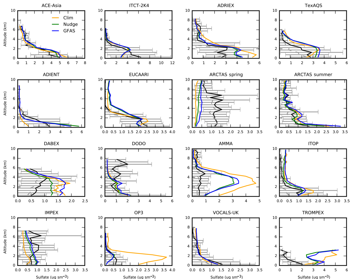
Figure 12. Vertical profiles of observed concentrations of sulfate (black) and simulated concentrations from the three simulations: CLIM (orange), NUDGE (green), and GFAS (blue). The observations are provided for 16 aircraft campaigns that investigated different regions of the world from 2001 to 2009 (Heald et al., 2011) (see also Fig. 2). The model is sampled along the flight tracks using a temporal average of the outputs over the duration of the campaign, and the error bars show the variabilities in the measurements. Simulated vertical profiles are shown as monthly and regional averages.
