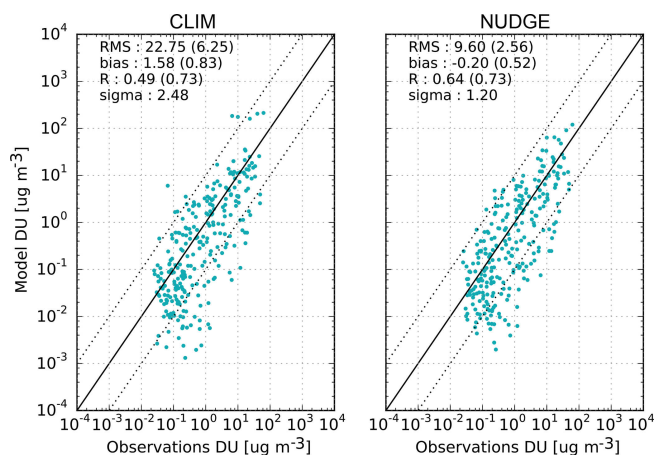
Figure 21. Scatterplot of observed versus simulated monthly mean dust surface concentrations at the AEROCE and SEAREX stations shown in Fig. 17. Simulated monthly means were constructed from the daily mean outputs sampled on the same days of the observations and collocated to the observation position for the time period 2003–2012.
