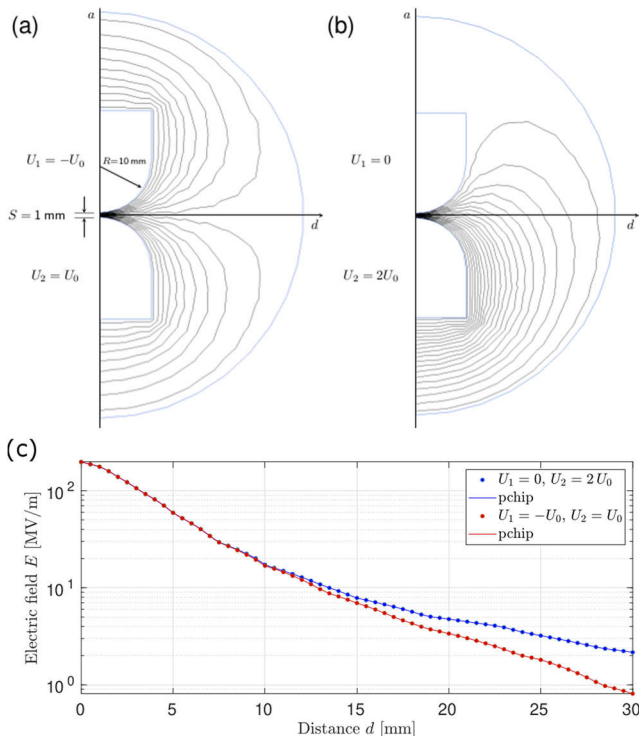
FIG. 1. Equipotential lines using QuickField 16 for the different potential configurations with R = 10\text{ mm} , S = 1\text{ mm} , and U_0 = 10\text{ kV} . The electrodes are rotationally symmetric around the axis a . Panel (a): the electrodes at the same but opposite potentials U_0 . Panel (b): one of the electrodes is grounded and another powered with twice the voltage U_0 . The electric field E as a function of distance d for both cases shown in panels (a) and (b) with a piecewise cubic hermite interpolating polynomial (pchip) is depicted in panel (c).
