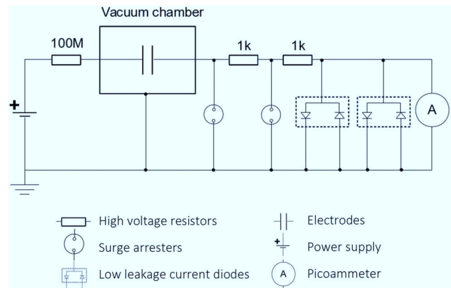
FIG. 2. Electrical schematic of the test apparatus used for the measurements. A 100\text{ M}\Omega resistor, two gas discharge boxes acting as surge arresters 18 , and two low-leakage diodes 19 are used to protect the power supply and the picoammeter during voltage breakdown in an electric discharge.
