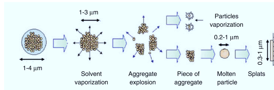
Fig. 2.27 Mechanism proposed for heat treatment of big agglomerates from liquid fragmentation to the splat formation [129].
