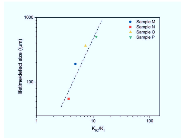
Fig. 4.14 Plot of lifetime t_f divided by initial defect size c as a function of the critical stress intensity factor divided by the apparent one (as shown in equation 4.3) for sample given in Table 4.3.
