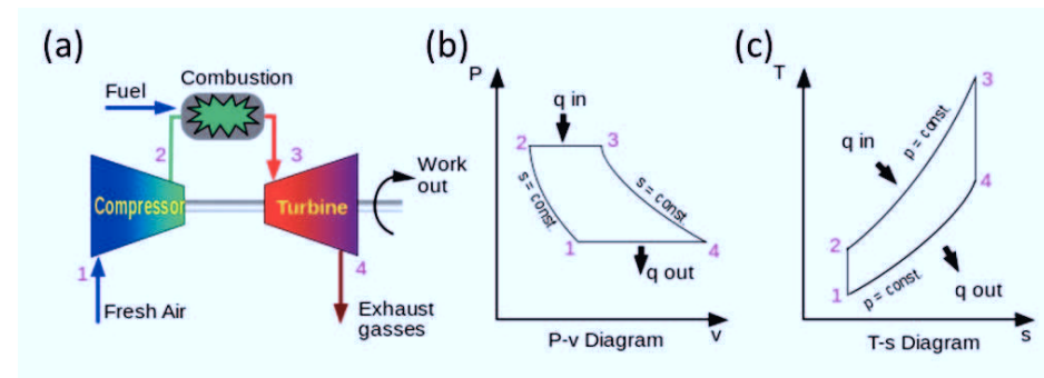
Fig. 2.2 Working mechanism for the ideal Brayton cycle (a); classical Pressure-Volume (P-V) diagram for the Brayton cycle (b); Temperature-Entropy (T-S) diagram [37].
