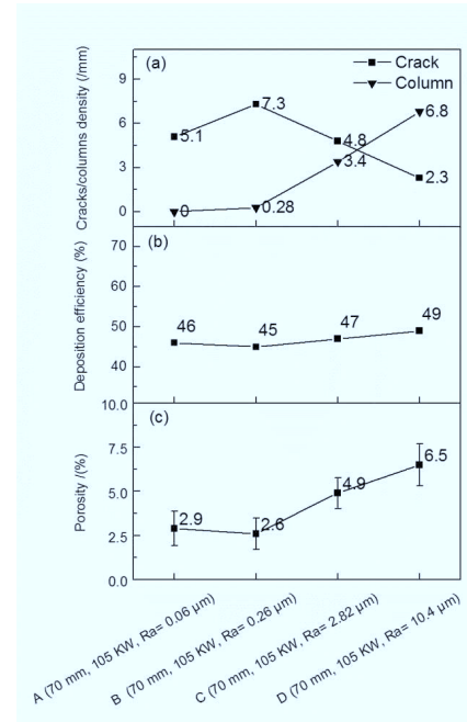
Fig. 4.2 Crack/column density (a), deposition efficiency (b) and porosity (c) for as-sprayed YSZ top coats deposited on bond coats with different surface roughness.
