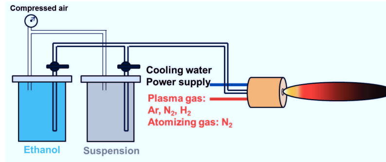
Fig. 3.3 Schematic of feeding system presented in Fig. 3.2.
