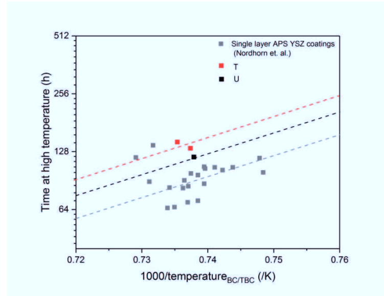
Fig. 7.5 Arrhenius plot of thermal cycling lifetime of multilayered APS/YSZ SPS/GZO sample T, U and single layered APS/YSZ samples.
