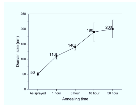
Fig. 6.6 Domain size of coatings after different annealing time at 1373 K.
