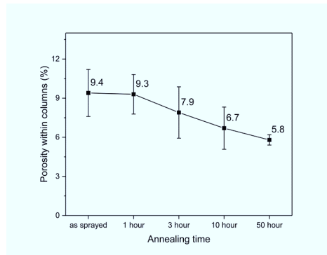
Fig. 6.7 Porosity of coating within columns after different annealing time at 1373 K.
