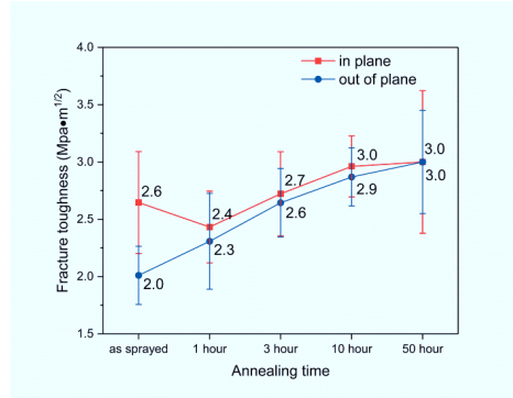
Fig. 6.10 Fracture toughness of coating after different annealing time at 1373 K.
