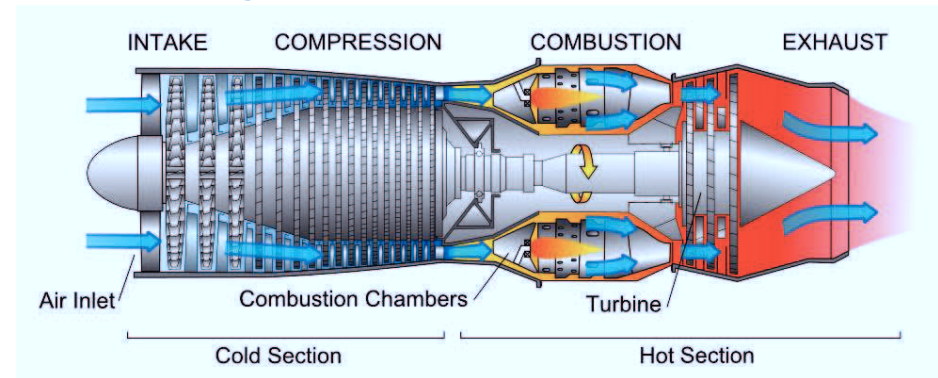
Fig. 2.1 Example of gas turbine (turbojet) configurations [34].
