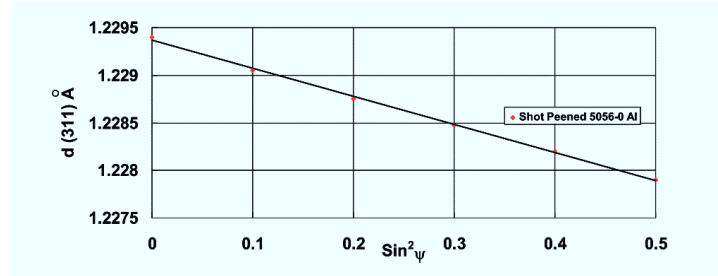
Fig. 3.6 Example of d-spacing versus \sin^2 \psi [147].
