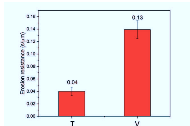
Fig.7.13 Erosion resistance of sample T and V.
