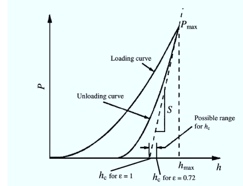
Fig. 3.7 Schematic of a typical indentation load-displacement curve [149].
