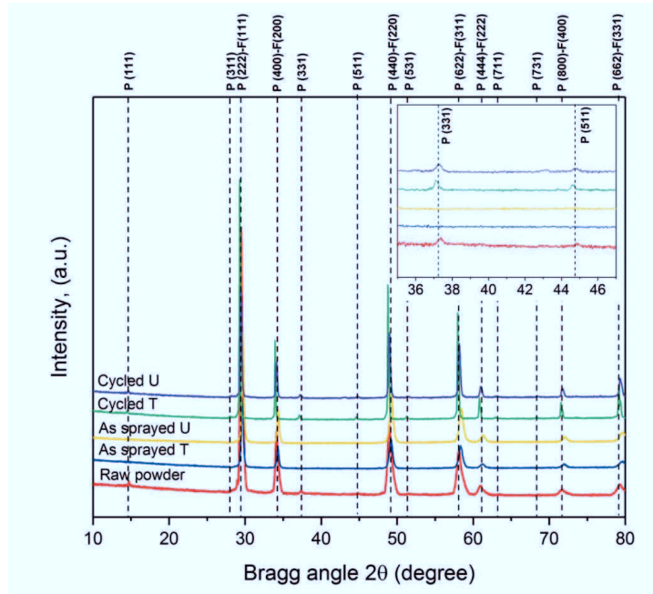
Fig.7.6 XRD pattern of raw powder, as-sprayed coatings and thermal cycled coatings.
