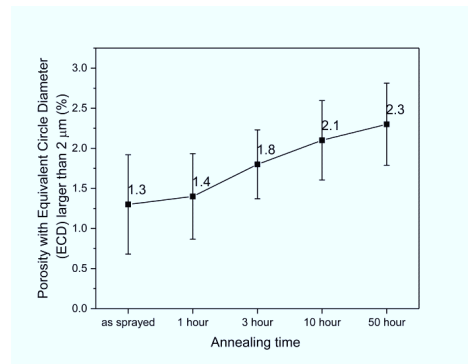
Fig. 6.4 Porosity with equivalent circle diameter larger than 2\ \mu\text{m} of coatings after different annealing time at 1373 K.
