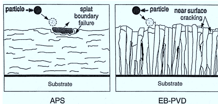
Fig. 2.12 A schematic diagram of the failure modes for APS and EB-PVD TBCs [71].
