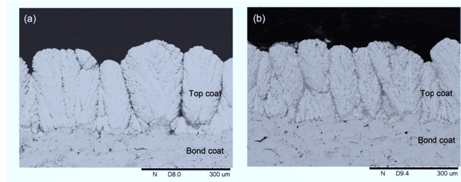
Fig. 4.6 Cross-section images of as-sprayed YSZ top coat (sample K (a) and L (b)) deposited with 5 wt.% solid content suspension on as-sprayed bond coats.
