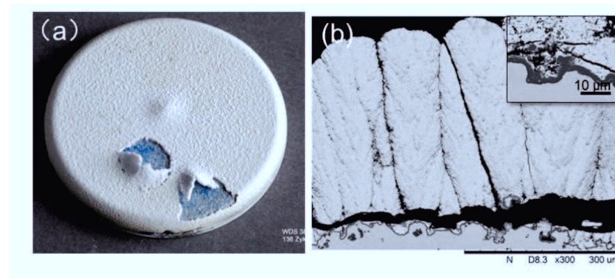
Fig. 4.13 Photograph (a) and cross-section microstructure SEM image (b) on thermal cycled sample P.
