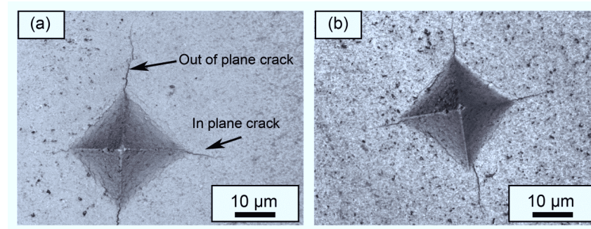
Fig. 6.9 Images of indentations imprinted on the cross-section of coatings. (a) as-sprayed, (b) annealed for 50 hours at 1373 K.
