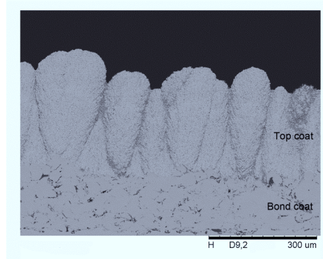
Fig. 4.5 Cross-section microstructure of as-sprayed YSZ top coat (sample J) deposited at 70 mm spraying distance with 84 kW input power on an as-sprayed bond coat.
