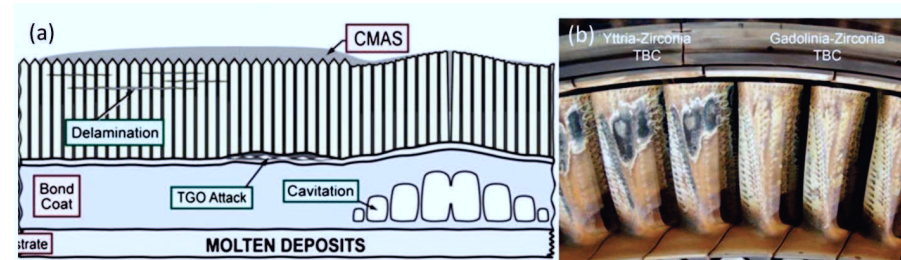
Fig. 2.13 (a) Identified TBCs failure mechanism attacked by CMAS and (b) example of CMAS attack on current airfoils (left part is coated with YSZ TBCs and the right part is coated with Gd_2Zr_2O_7 TBCs) [79, 80].
