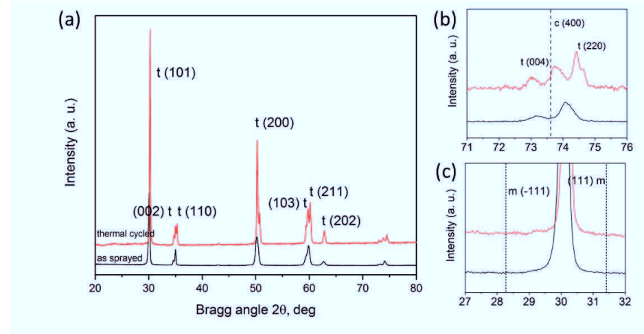
Fig. 5.5 XRD diagram of sample Q (a), diagrams zoomed in Bragg angle range of 70-76 ° (b) and 27-32 ° (c).
