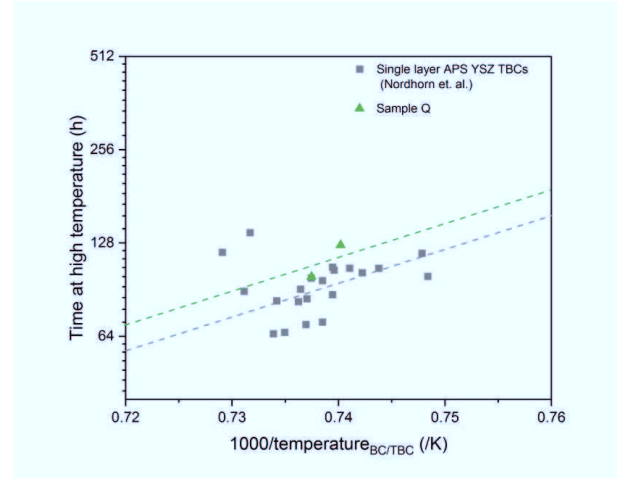
Fig. 5.6 Arrhenius plot on thermal cycling lifetime of samples Q and standard APS coatings.
