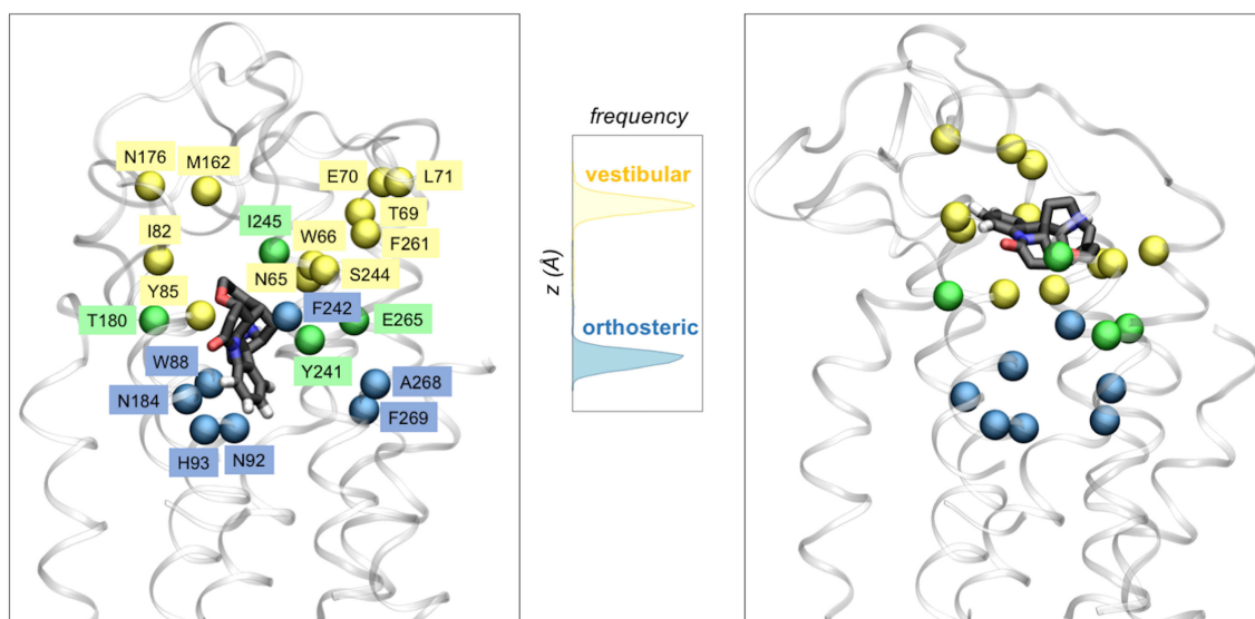
FIGURE 3 | Two binding site architecture of TAS2R46. The agonist strychnine (in licorice representation) can bind in either the orthosteric site (left panel) or the vestibular site (right panel). Receptor residues interacting with the ligand in the orthosteric site, the vestibular site or both sites are shown with blue, yellow or green spheres, respectively. The central panel displays the distribution of the ligand center-of-mass z coordinate for the two \sim 1 \mu\text{s} MM/CG simulations, showing that strychnine stabilized either in the orthosteric site or in a second (vestibular) site, located further toward the extracellular side.
