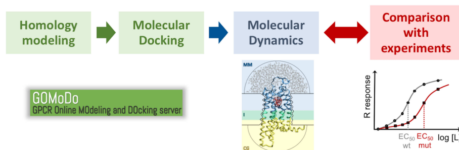
FIGURE 4 | Proposed protocol to study ligand binding in low resolution GPCR models. The initial model generated with homology modeling and molecular docking (e.g., using the GOMoDo webserver, Sandal et al., 2013) is further refined using molecular dynamics (e.g., using the molecular mechanics/coarse grained or MM/CG approach developed in our group, Leguèbe et al., 2012). The receptor/ligand interactions predicted by the simulations have to be validated by extensive comparison with experimental data (typically site-directed mutagenesis and dose-response functional assays).
