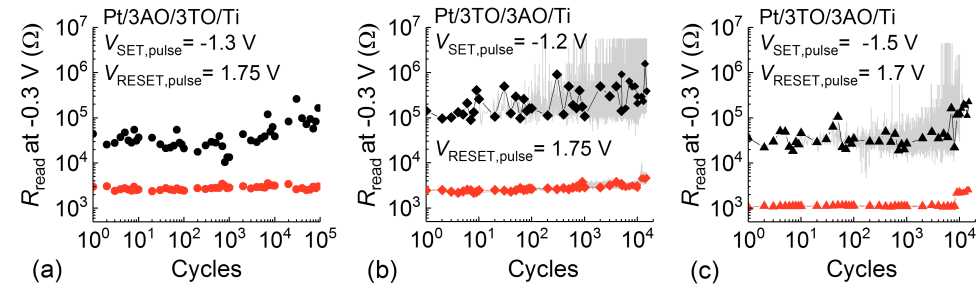
Figure 4.26: The endurance test was applied (a) in a Pt/3AO/3TO/Ti cell with pulse length t_{pulse} = 1 \mu s . (b) and (c) represent the endurance test in a Pt/3TO/3AO/Ti cell with t_{pulse} = 100 \mu s and t_{pulse} = 1 \mu s , respectively. The applied SET and RESET pulses are listed in each graph.
