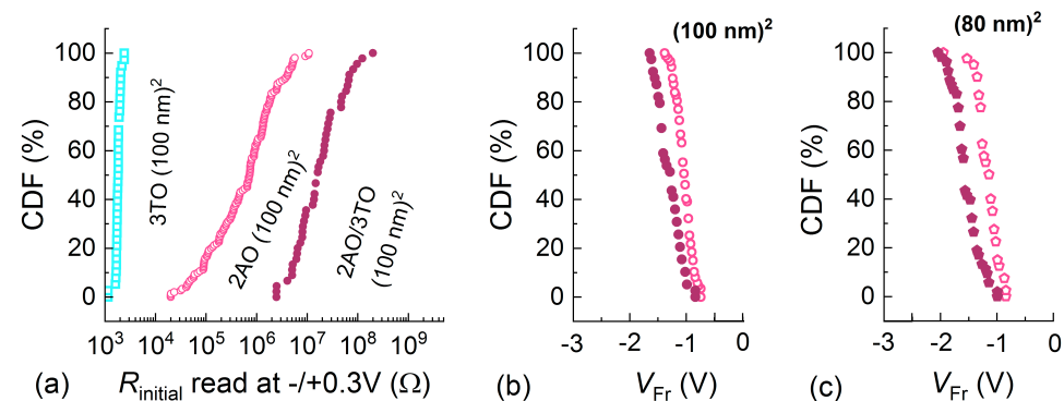
Figure 4.29: Comparison of the three Pt/oxide(s)/Ti stacks: 3 nm \text{TiO}_2 (blue open square), 2 nm \text{Al}_2\text{O}_3 with (claret-red solid circle) and without (pink open circle) an additional 3 nm \text{TiO}_2 artificial layer. (a) The read-out initial resistance ( R_{\text{initial}} ) of the pristine cells measured at \pm 0.3 \text{ V} , (b) V_{\text{Fr}} of cells from (a). The CDF plots comprise measurements of 38, 45 and 88 cells with (100 \text{ nm})^2 cells, respectively. (c) CDF plots of V_{\text{Fr}} for about 50 cells with (80 \text{ nm})^2 size for each stack. Solid and open pentagon stand for 2 nm \text{Al}_2\text{O}_3 -based cells with and without 3 nm \text{TiO}_2 artificial layer, respectively.
