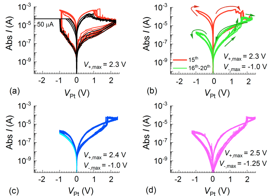
Figure 8.11: (a-b) Transition from c8w to 8w BRS is observed in a (100 \text{ nm})^2 Pt/3 nm \text{TiO}_2 /3 nm \text{Al}_2\text{O}_3 /Ti cell by |I_{CC}| increased to 600 \mu\text{A} . (c-d) Stable 8w BRS with switching parameters listed in the lower-right corner of each graph. The switching direction is depicted by arrows. For each parameter variation at least 20 cycles were performed.
