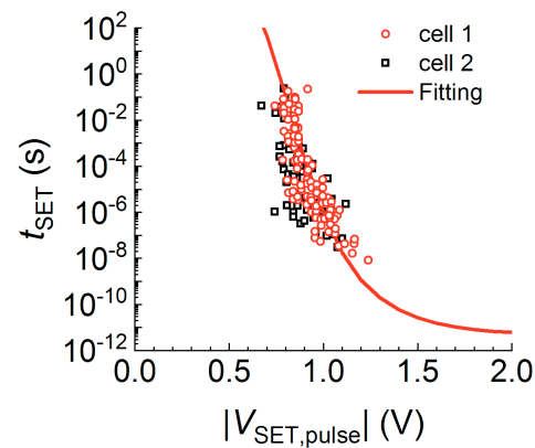
Figure 5.6: SET time as a function of the applied SET pulse amplitude in two Pt/5 nm \text{Al}_2\text{O}_3/\text{Ti} cells from Fig. 5.5. The experimental data are depicted as dots and the model calculation as the red line. The resistance range for dots and the best simulation parameters are summarized in Tab. 5.1
