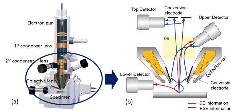
Figure 3.11: Schematic of (a) section view of Hitachi SU8000 setup and (b) its detection systems. The figures are redrawn from [191, 192].
