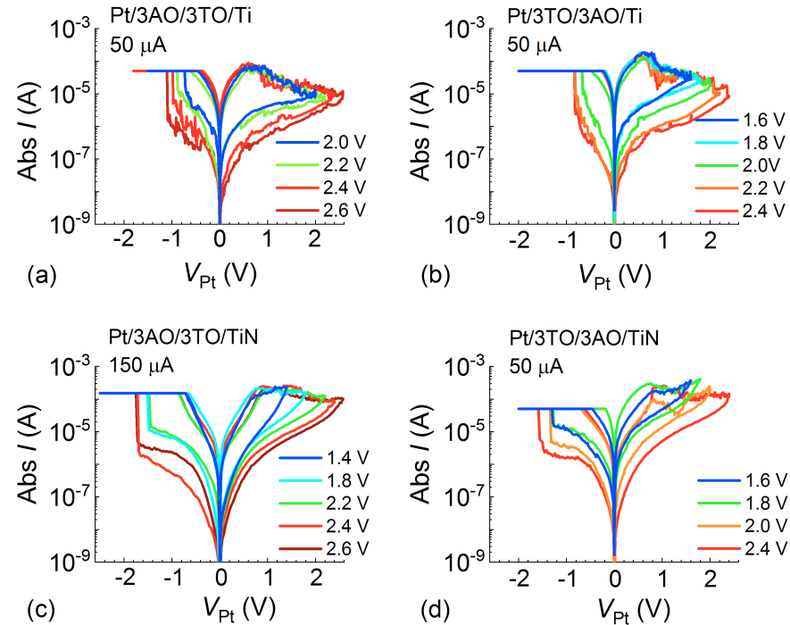
Figure 4.20: V_{+,max} influence on the c8w BRS in (a) Pt/3AO/3TO/Ti, (b) Pt/3TO/3AO/Ti, (c) Pt/3AO/3TO/TiN, (d) Pt/3TO/3AO/TiN stacks. The applied |I_{CC}| are given under the stack and the V_{+,max} variation are listed in the lower-right corner of each graph.
