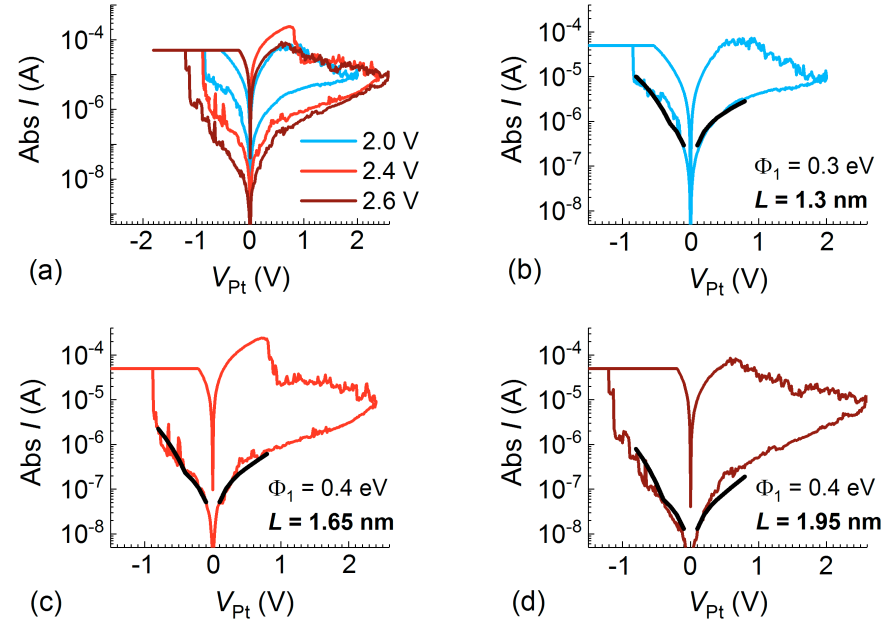
Figure 7.15: (a) Comparison of one typical I(V) curve with different V_{+, \text{max}} values in a Pt/3AO/3TO/Ti cell. The best simulation result on I(V) characteristics with V_{+, \text{max}} of (b) 2.0 V, (c) 2.4 V, (d) 2.6 V. The simulation parameters are listed in each graph, whereas m^* = 0.23 \cdot m_0 , A = 100 \text{ nm}^2 and \Phi_2 = 1.1 eV are kept constant.
