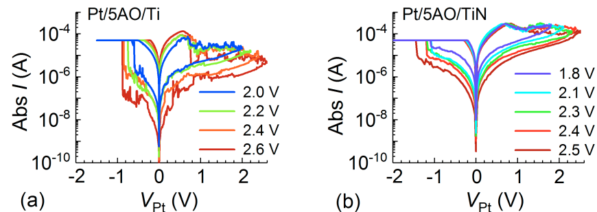
Figure 4.10: V_{+,max} influence on the c8w BRS in Pt/5AO/TE cells with different top electrodes: (a) evaporated Ti and (b) sputtered TiN. |I_{CC}| is kept as 50 \mu A .
