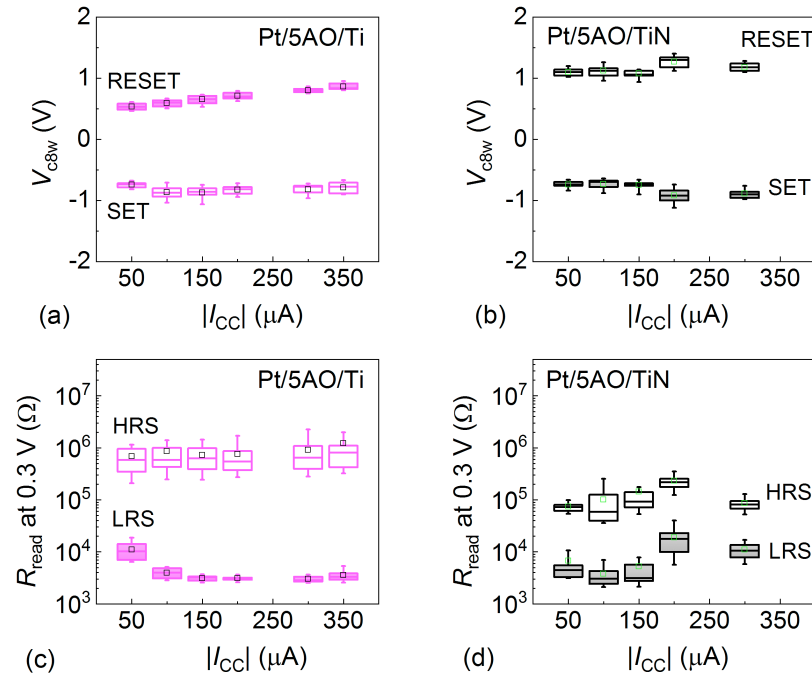
Figure 4.13: Dependency of the characteristic switching parameters from the |I_{CC}| variation in the form of box plots for V_{c8w,SET} , V_{c8w,RESET} and for R_{c8w,ON} , R_{c8w,OFF} in Pt/5AO/TE cells with Ti (a,c) and TiN (b,d) electrode, respectively. The data for each varied parameter is taken from Fig. 4.12 for 20 cycles.
