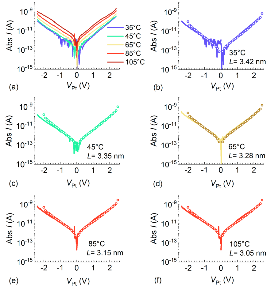
Figure 7.7: (a) The temperature dependent I(V) characteristics of initial state in a Pt/3TO/3AO/Ti cell. (b) to (f) are experimental curves (colored lines) and the corresponding best simulation result (dots). Some parameters are kept constant: \Phi_1 = 1.9 eV, \Phi_2 = 2.4 eV, m^* = 0.24 \cdot m_0 , tunneling area A = (100 \text{ nm})^2 , the tunneling length L and the substrate temperature are listed in the lower-right corner of (b-f).
