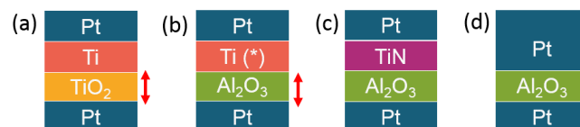
Figure 4.1: Stacks of oxide single-layers with varied layer thickness in nano-crossbar structures: (a) Pt/3 nm to 11 nm TiO 2 /evaporated Ti, (b) Pt/2 nm or 5 nm Al 2 O 3 /evaporated Ti or sputtered Ti*, (c) Pt/5 nm Al 2 O 3 /sputtered TiN, (d) Pt/5 nm Al 2 O 3 /10 nm evaporated Pt. The bottom electrode for all stacks was 30 nm sputtered Pt and all 10 nm top electrodes linked with 20 nm Pt capping layer that was deposited by the same system without breaking the vacuum.
