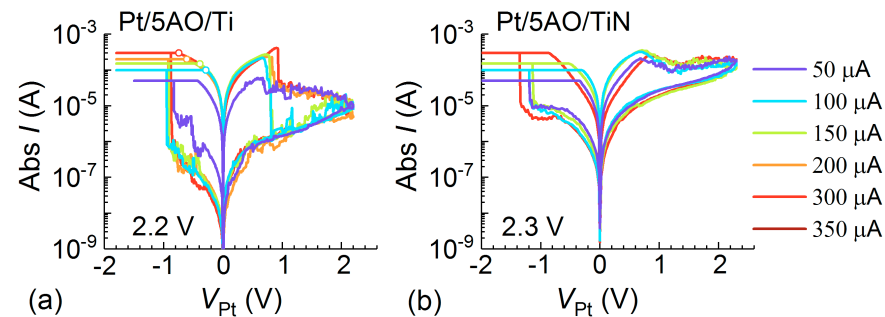
Figure 4.12: Current compliance influence on the c8w BRS in Pt/5AO/TE cells with (a) evaporated Ti and with (b) sputtered TiN. The tested |I_{CC}| values are listed on the right and the applied V_{+,max} are given in the lower-left corner of each graph.
