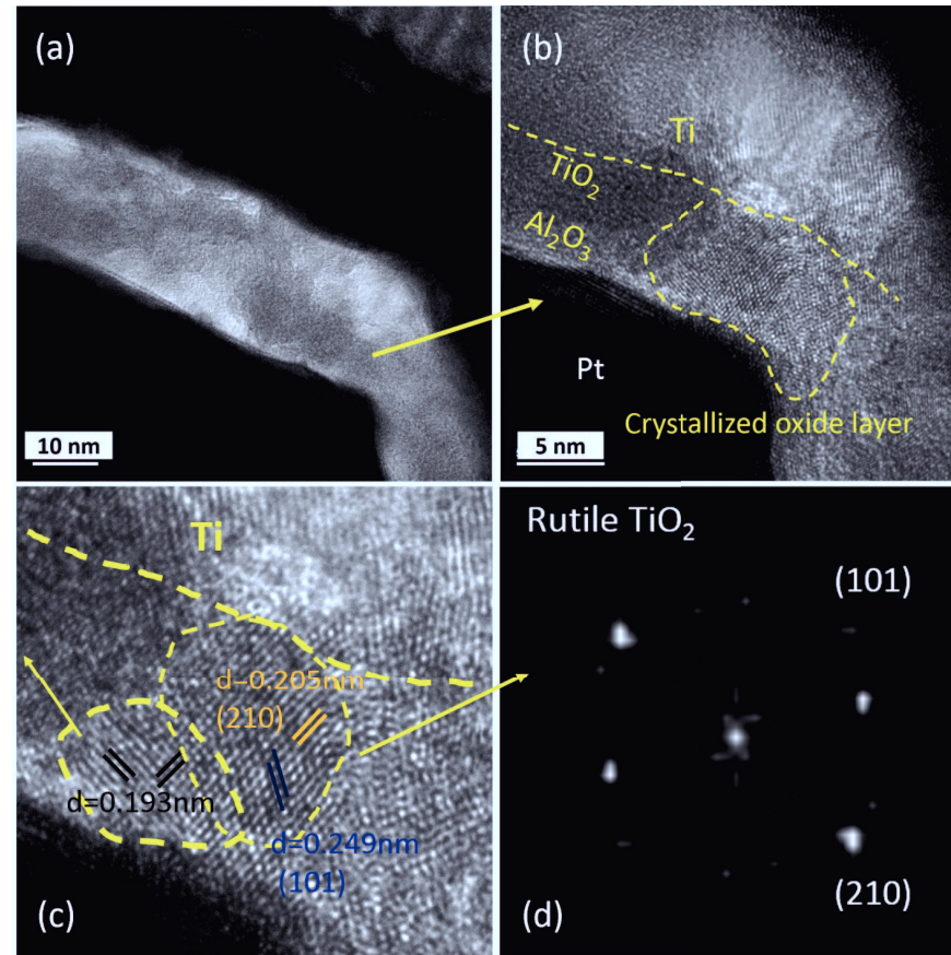
Figure 6.3: The TEM analysis of the filament region in an active switched Pt/3 nm Al 2 O 3 /3 nm TiO 2 /Ti/Pt ReRAM cell: (a) overview of the cross-section with the active region for resistive switching, (b) region with the crystallized filament, (c) high-resolution TEM of the two marked crystallized regions with atomic resolution, (d) the fast Fourier transform (FFT) of the upper selected region in (c), which shows a rutile structure.
