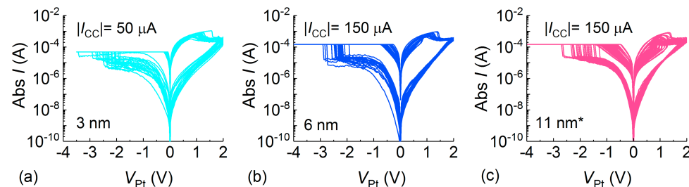
Figure 4.4: Overview of I(V) characteristics during c8w BRS cycles of Pt/ TiO_2 /Ti stacks for (a) 3 nm TiO_2 , (b) 6 nm TiO_2 and (c) 11 nm* TiO_2 . The I(V) curves are given for (a) 20 cycles, (b) 20 cycles and (c) 42 cycles.
