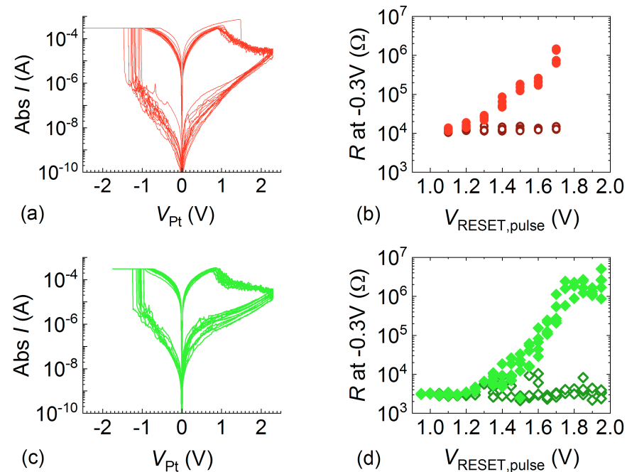
Figure 5.7: Typical I(V) curves obtained from V_{+,max} = 2.3 V and |I_{CC}| = 300 \mu A for (a) one Pt/5 nm Al_2O_3 /Ti cell with (80\text{ nm})^2 cell size and (c) one Pt/3 nm Al_2O_3 /3 nm TiO_2 /Ti cell with (100\text{ nm})^2 cell size. (b) and (d) show the V_{RESET,pulse} dependent R_{read} for HRS (solid dots) and LRS (open dots) in two (80\text{ nm})^2 single-layer and bilayer cells, respectively. The RESET pulse length is kept as 1 \mu s.
