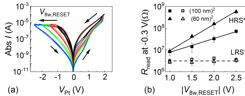
Figure 8.6: (a) The I(V) characteristics for increased |V_{8w, \text{RESET}}| obtained in a (60 \text{ nm})^2 Pt/3 nm \text{TiO}_2 /Ti cell. (b) The readouts for \text{HRS}^* (solid) and \text{LRS}^* (open) as a function of |V_{8w, \text{RESET}}| for the cell size of (60 \text{ nm})^2 (triangle) and (100 \text{ nm})^2 (square).
