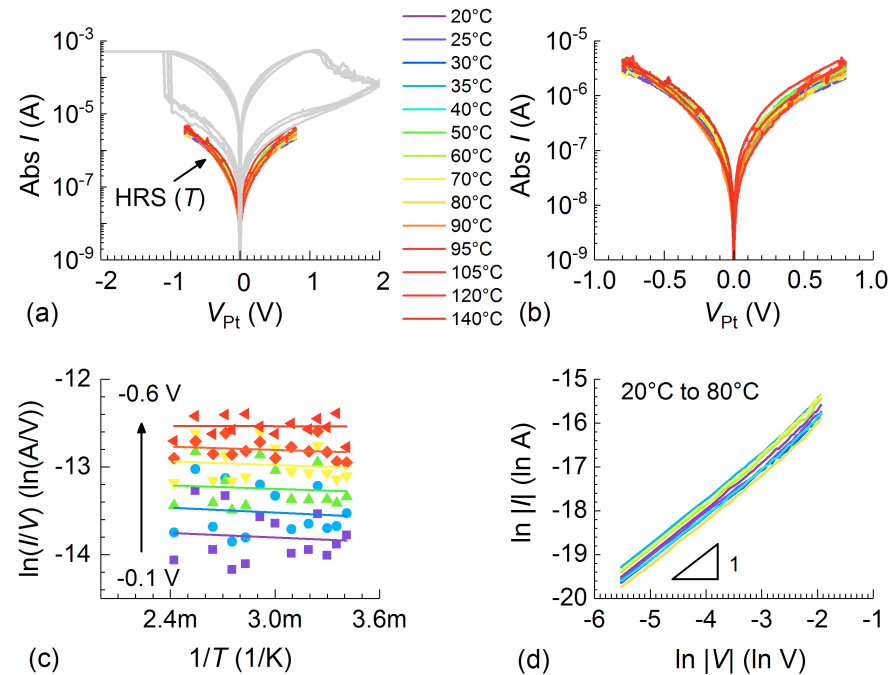
Figure 7.8: (a) The I(V) characteristics of a Pt/2AO/Ti cell in 20 cycles (grey curves) measured at room temperature with V_{+,max} = 2.0\ V and |I_{CC}| = 150\ \mu A . The read-out I(V) loops for HRS were measured from 20°C to 140°C as rainbow lines. (b) The zoomed I(V, T) curves. (c) The plots of \ln(I/V) vs. 1/T and (d) of \ln|I| vs. \ln|V| from (b) for the negative voltage branch.
