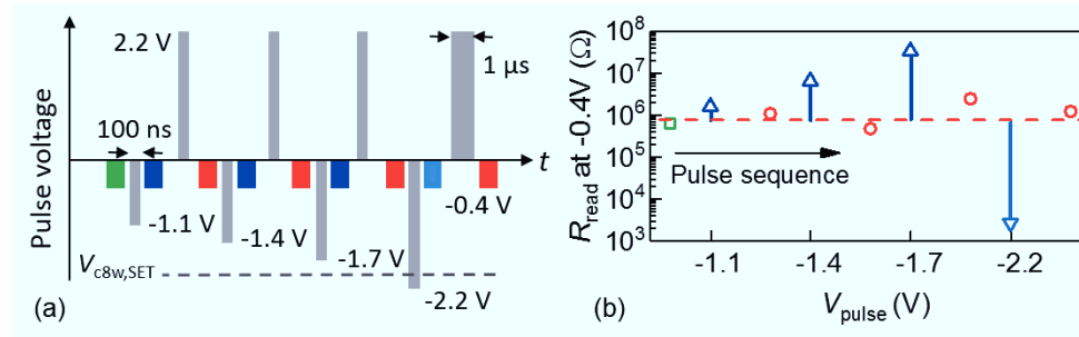
Figure 8.8: Pulsed switching behavior in the 8w BRS mode. (a) A schematic diagram of pulse procedure carried out in a (100 \text{ nm})^2 Pt/3 nm \text{TiO}_2/\text{Ti} cell. (b) The read-out resistances measured at -0.4 V after each write pulse. The red circles represent the read-out values of LRS* programmed with a signal of 2.2 V. The green square is the initial read-out value recorded after the last DC sweep loop. The triangles mark the read-out values after applying a negative pulse starting at -1.1 V and ending at -2.2 V, which exceeds the threshold voltage for c8w SET. The figure is redrawn from [261].
