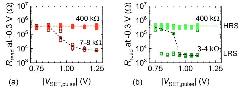
Figure 5.2: The SET behavior obtained for SET pulses length of 1 \mu s of (a) a Pt/5 nm \text{Al}_2\text{O}_3/\text{Ti} cell with (80 \text{ nm})^2 cell size and (b) a Pt/3 nm \text{Al}_2\text{O}_3/3 \text{ nm TiO}_2/\text{Ti} cell with (100 \text{ nm})^2 cell size. The values for HRS (solid dots) and for LRS (open dots) are read out before and after SET pulse, respectively. The colored dash lines represent the almost constant HRS of \approx 400 \text{ k}\Omega . The black dash lines link the median value of LRS.
