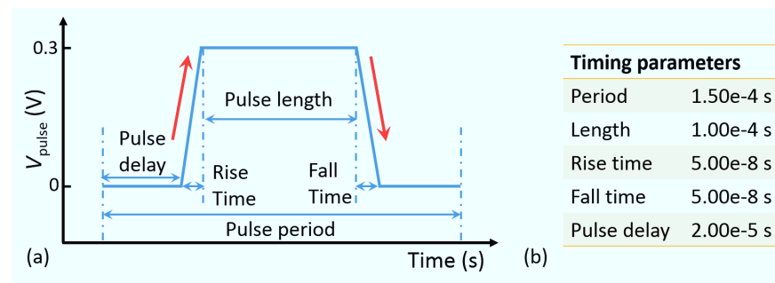
Figure 3.16: (a) Illustration of the pulse signal and (b) its timing parameters for a read step applied in the Keithley 4200 SCS setup.
