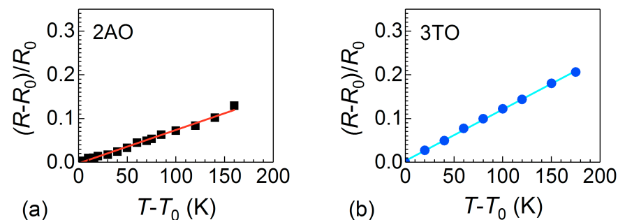
Figure 7.20: Temperature dependency of the resistance of (a) one Pt/2AO/Ti cell and of (b) one Pt/3TO/Ti cell set into the c8w LRS normalized to the resistance value R_0 at T_0 = 298 \text{ K} . The TCR values of (0.76 \pm 0.02) \cdot 10^{-3} \text{K}^{-1} and of (1.18 \pm 0.01) \cdot 10^{-3} \text{K}^{-1} are obtained from the linear fitting in (a) and (b), respectively.
