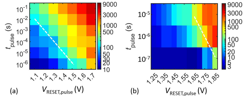
Figure 5.8: Illustration of the read-out resistance against pulse length and RESET pulse voltage in (a) one Pt/5 nm \text{Al}_2\text{O}_3/\text{Ti} cell and in (b) one Pt/3 nm \text{Al}_2\text{O}_3/3 nm \text{TiO}_2/\text{Ti} cell with the same (80 \text{ nm})^2 cell size. The white dash lines mark the boundary for the read-out resistance of \approx 100 \text{ k}\Omega .
