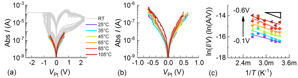
Figure 7.16: (a) The I(V) characteristics of a Pt/3TO/3AO/Ti cell in 20 cycles (grey curves) measured at room temperature with V_{+,max} = 2.3 V and |I_{CC}| = 150 \mu A. The read-out I(V) loops for HRS measured from 25°C to 105°C as rainbow lines. (b) The zoomed I(V, T) curves. (c) The plots of \ln(I/V) vs. 1/T from (b) for the negative voltage branch.
