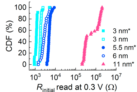
Figure 4.3: CDF plots of the read-out initial resistance ( R_{initial} ) in Pt/ TiO_2 /Ti cells with XRR fitting thickness ranging from 3 nm* to 11 nm*. The star ("*") marks the TiO_2 layers deposited in the FlexAL ALD system (see "Appendix C"), while others were fabricated by the standard ALD process with AIXTRON® reactor (see Tab. 3.1). The statistics are gathered from 23, 38, 26, 31, 36 cells (from left to right), respectively.
