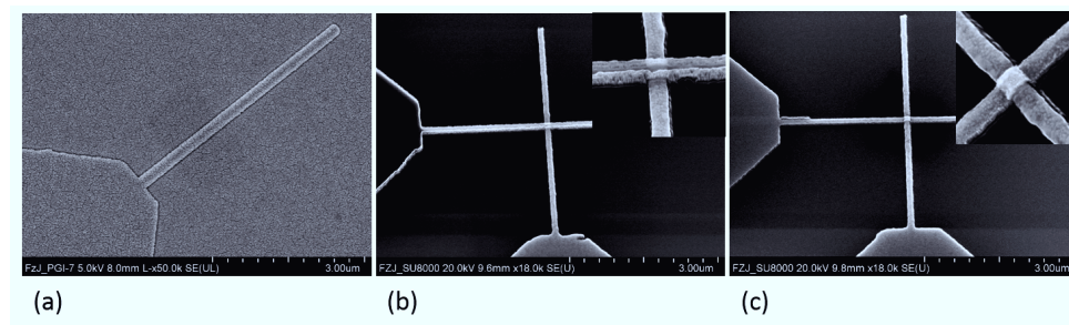
Figure 3.14: SEM images for nano-crossbar devices (a) after oxide layer and top electrode deposition, (b) after development, (c) after removing residual resist.
