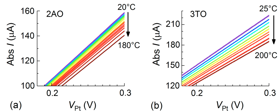
Figure 7.19: The temperature dependent I(V) behavior in LRS for two single-layer devices, namely, (a) Pt/2 nm \text{Al}_2\text{O}_3/\text{Ti} , (b) Pt/3 nm \text{TiO}_2/\text{Ti} .
