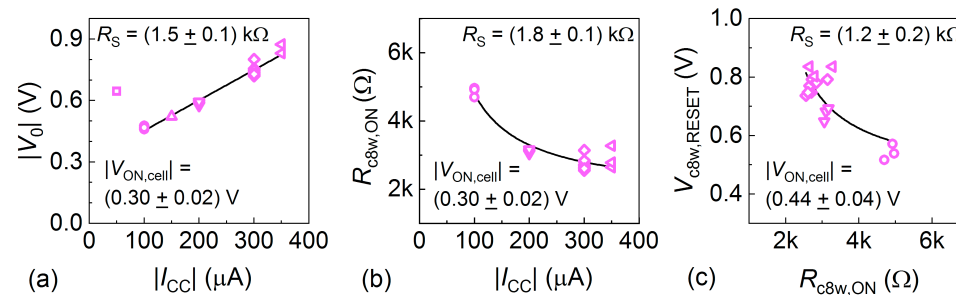
Figure 4.14: (a) The filtered value of |V_0| extracted from the I(V) curves as the function of |I_{CC}| for a Pt/5AO/Ti cell from Fig. 4.12 (a). The data point for |I_{CC}| = 50 \mu\text{A} is excluded from the linear fitting. (b) The filtered value of R_{c8w,ON} as the function of |I_{CC}| from Fig. 4.13 (a). (c) The filtered value of V_{c8w,RESET} as the function of R_{c8w,ON} . The R_{c8w,ON} value is read out at 0.3 V.
