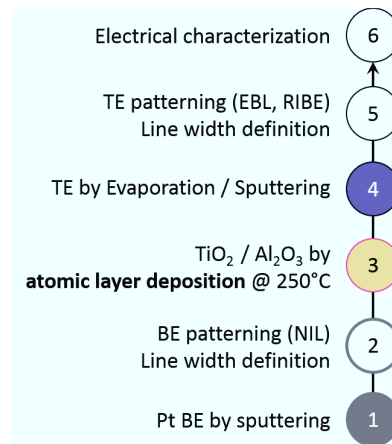
Figure 3.12: Fabrication procedure of nano-crossbar devices
