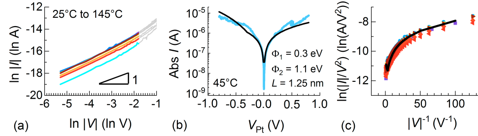
Figure 7.14: (a) The plots of \ln|I| vs. \ln|V| from Fig. 7.13 (b) for negative bias. (b) The read-out I(V) curve (blue line) for HRS measured at 45°C from Fig. 7.13 (b). The best simulation result is drawn in black with m^* = 0.23 \cdot m_0 and A = 100 \text{ nm}^2 , whereas the changeable parameters are listed in the lower-right corner. (c) The read-out I(V, T) curves from Fig. 7.13 (b) and the simulation result from (b) are plotted into \ln(|I|/V^2) vs. |V|^{-1} as color dots and as black line, respectively.
