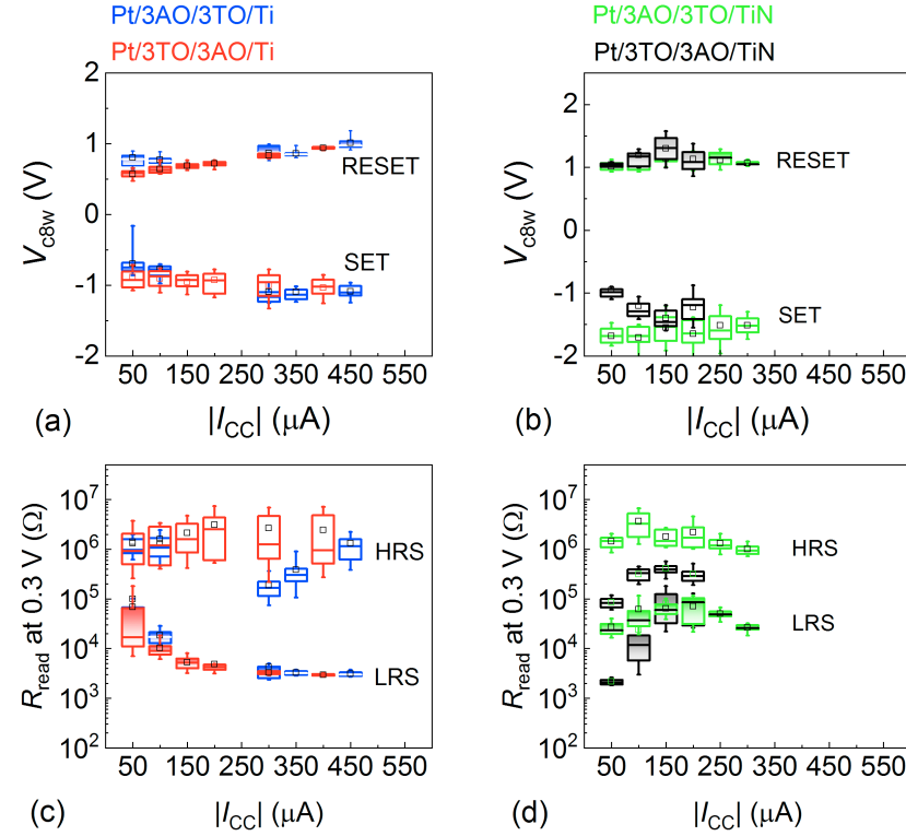
Figure 4.24: (a,b) Box plots of V_{c8w,SET} and of V_{c8w,RESET} from Fig. 4.23 in Pt/3AO/3TO/Ti (blue), Pt/3TO/3AO/Ti (red), Pt/3AO/3TO/TiN (green), Pt/3TO/3AO/TiN (black) stacks. (c,d) The corresponding box plots of R_{c8w,OFF} and of R_{c8w,ON} for these four stacks.
