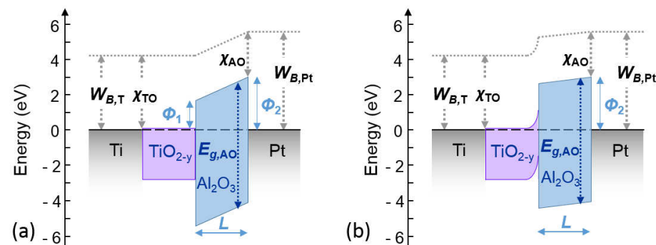
Figure 7.6: The suggested band diagram for initial state in the \text{Pt}/3\text{AO}/3\text{TO}/\text{Ti} cell based on (a) the Simmons' tunneling model with trapezoidal barrier and (b) Schottky tunneling through an extra \text{TiO}_2 depletion region and insulating \text{Al}_2\text{O}_3 layer.
