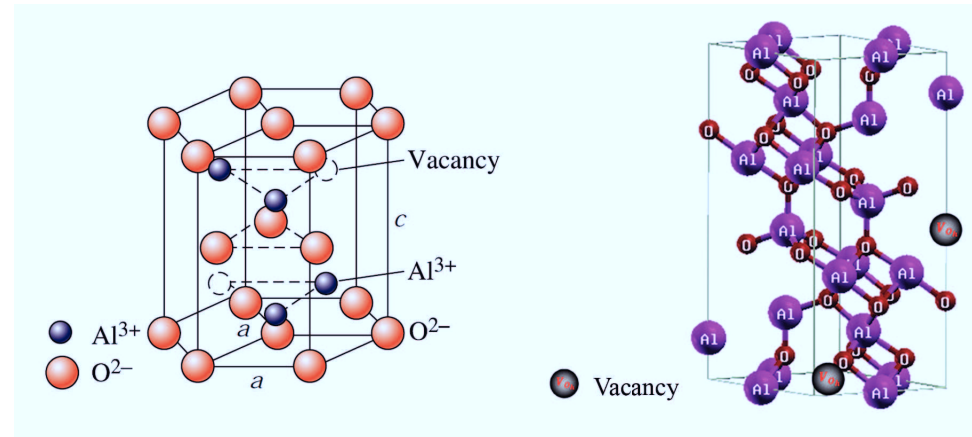
Figure 2.14: Schematic structures of a unit cell of (a) \alpha -alumina ( \alpha -Al 2 O 3 ) and (b) \gamma -alumina ( \gamma -Al 2 O 3 ). Images are taken from [139,140].
