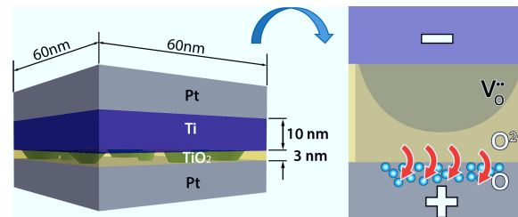
Figure 8.18: (a) An asymmetric \text{Pt}/3\text{ nm TiO}_2/\text{Ti} structure in initially conductive state. (b) Zoomed into the switching regime during the 1 st c8w-type RESET.
