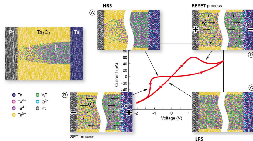
Figure 2.5: Schematic illustration of the filamentary-type VCM switching model. The switching hysteresis follows the c8w orientation by starting from (a) HRS, undergoing (b) a SET process into (c) LRS and a closing of the loop by (d) a RESET process. The Image is redrawn from [86].
