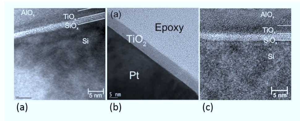
Figure 2.13: Transmission electron microscopy images of (a) a 3 nm amorphous \text{TiO}_x film on Si(100) substrate grown at 200°C, (b) a 6 nm amorphous \text{TiO}_2 film on Pt substrate grown at 260°C, (c) a 3 nm amorphous \text{TiO}_x film on Si(100) substrate grown at 300°C. Images are taken from [114, 115].
