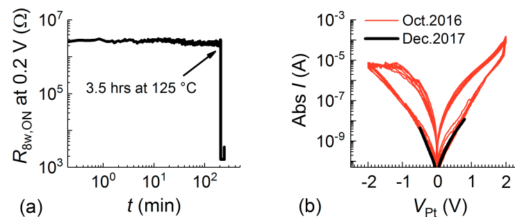
Figure 8.3: The stability of 8w resistance states in different Pt/3 nm \text{TiO}_2 /Ti cells: (a) retention test for 8w LRS* performed at 125°C in a (100 \text{ nm})^2 cell; (b) 8w BRS in red performed in a (80 \text{ nm})^2 cell at room temperature in October 2016. The 8w HRS* was written by -2.0 V in the last red RESET loop. The black lines are the read-out loop measured at room temperature after more than one year storage under nitrogen condition.
