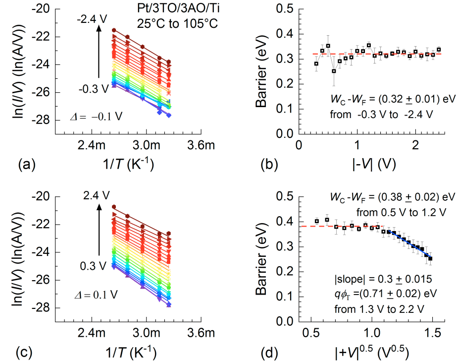
Figure A.3: (a) \ln(I/V) vs. 1/T plots from Fig. 7.7 (a) for negative bias and (c) for positive bias. (b) and (d) are the voltage dependent slopes from (a) and (c).
