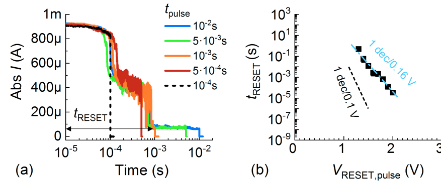
Figure 5.9: (a) The transient current response with the applied V_{\text{RESET,pulse}} of 1.8 V in one (100 \text{ nm})^2 Pt/5 nm \text{Al}_2\text{O}_3/\text{Ti} cell with R_{\text{pre,ON}} \approx 2 \text{ k}\Omega for LRS. The tested pulse lengths were listed as legend. (b) The plot of t_{\text{RESET}} against V_{\text{RESET,pulse}} for two Pt/5 nm \text{Al}_2\text{O}_3/\text{Ti} cells. The black dash line is taken from cell with R_{\text{pre,ON}} = 10\text{-}17 \text{ k}\Omega . The cyan dash line is the slope of the black square obtained from cells with R_{\text{pre,ON}} of around 2 k \Omega .
