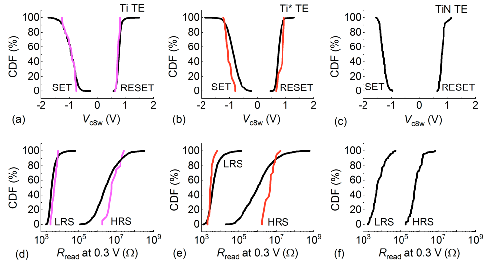
Figure 4.9: CDF plots of V_{c8w,SET} and of V_{c8w,RESET} in a Pt/5AO/TE stack with (a) evaporated Ti for 70 cells, (b) sputtered Ti^* for 48 cells, (c) sputtered TiN for 5 cells. The corresponding CDF plots of read-out resistance for HRS and LRS are shown in (d) to (f). The black lines are the statistics in all tested cells, colored lines represent the 20 cycles in the representative cell from Fig. 4.8.
