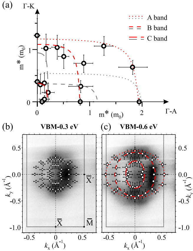
FIG. 5. (a) Polar plot of the effective masses for the bulk valence bands along different directions in k_{\parallel} space obtained from a fit to the experimentally observed bands. The red lines show our assignment to the different bands, while the gray lines correspond better to an assignment in agreement with theory. (b),(c) Comparison between the measured energy surfaces at (b) 0.3 eV and (c) 0.6 eV below VBM, as already shown in Figs. 3(b) and 3(c), and those calculated from the effective masses. The red curves show the suggested shapes of the energy surfaces for the three bands.
