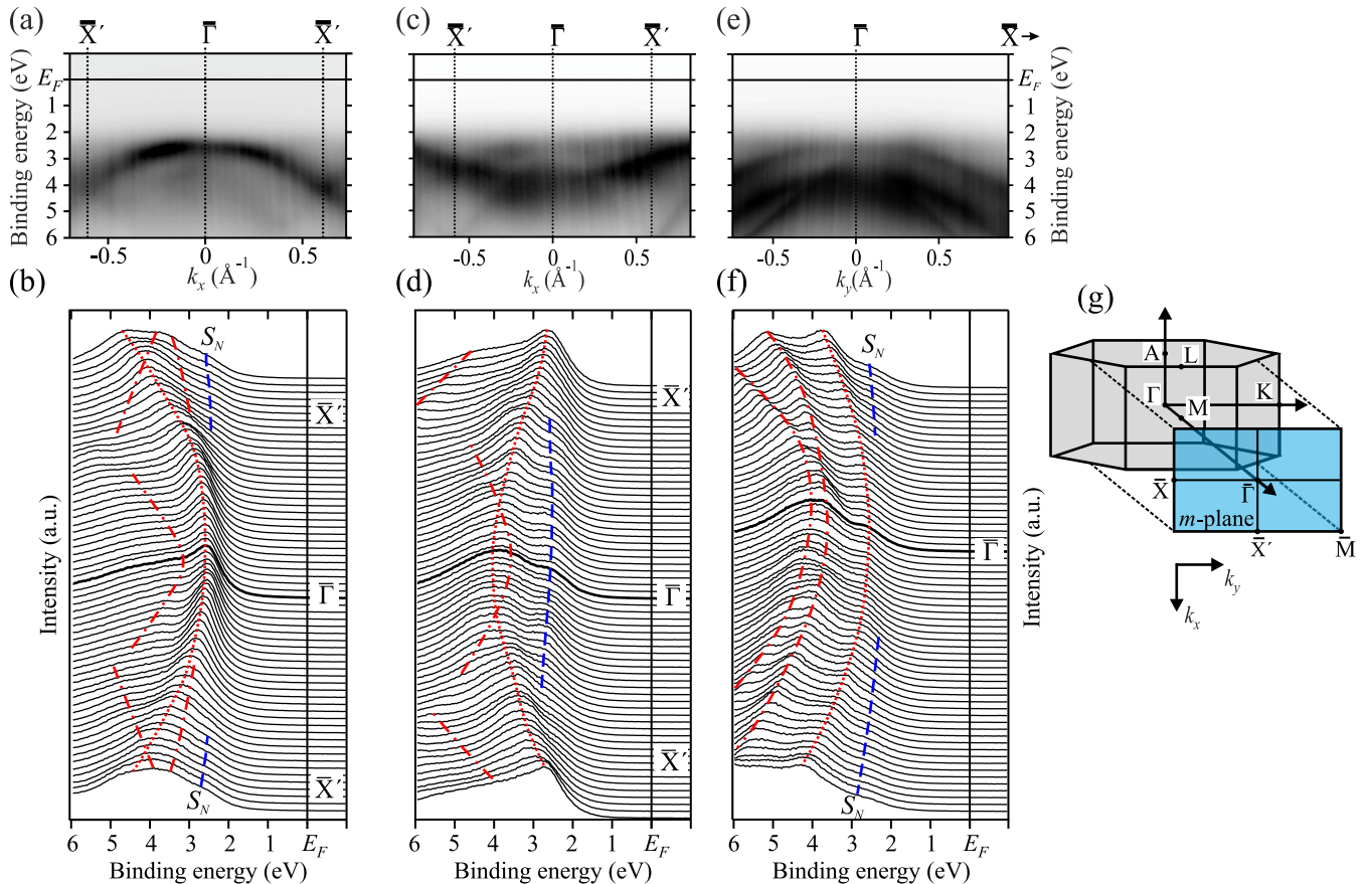
FIG. 2. ARPES results for (a),(b) h\nu = 62 eV and (c)–(f) h\nu = 80 eV measured along (a)–(d) the \bar{\Gamma} - \bar{X}' and (e),(f) the \bar{\Gamma} - \bar{X} directions. The blue lines indicate the dispersion of the surface state band S_N , while the red lines indicate bulk bands. (g) Relation between the wurtzite bulk Brillouin zone (gray) and the SBZ of the (10 \bar{1} 0) surface ( m -plane, blue).
