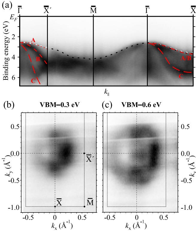
FIG. 3. (a) Bulk dispersion along the \bar{\Gamma}-\bar{X}'-\bar{M}-\bar{\Gamma}-\bar{X} path ( h\nu = 62 eV). The red dashed and dotted lines indicate the bulk bands analyzed in this work. The black and white dashed lines show the calculated projection of the upper valence band edge taken from Refs. [39] and [40], respectively. (b),(c) Energy surfaces at (b) 0.3 eV and (c) 0.6 eV below the VBM. The asymmetry of the intensity distribution is related to matrix element effects.
