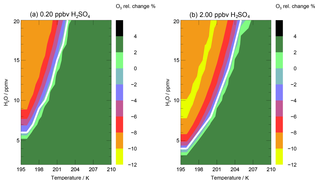
Figure 9. Relative ozone change during the 7 d simulation along the standard trajectory dependent on temperature and H_2O ratio for climatological non-enhanced (a) and enhanced (b) sulfate conditions. The white line corresponds to the water- and temperature-dependent chlorine activation threshold.
