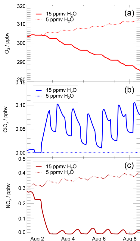
Figure 2. Volume mixing ratio of \text{O}_3 (a), \text{ClO}_x (b) and \text{NO}_x (c) during a simulation with 15 ppmv \text{H}_2\text{O} and 5 ppmv \text{H}_2\text{O} . These water vapour mixing ratios are chosen because they are clearly in the regime of low (5 ppmv) and elevated (15 ppmv) water vapour. The x axis marks refer to 00:00 local time (06:00 UTC).
