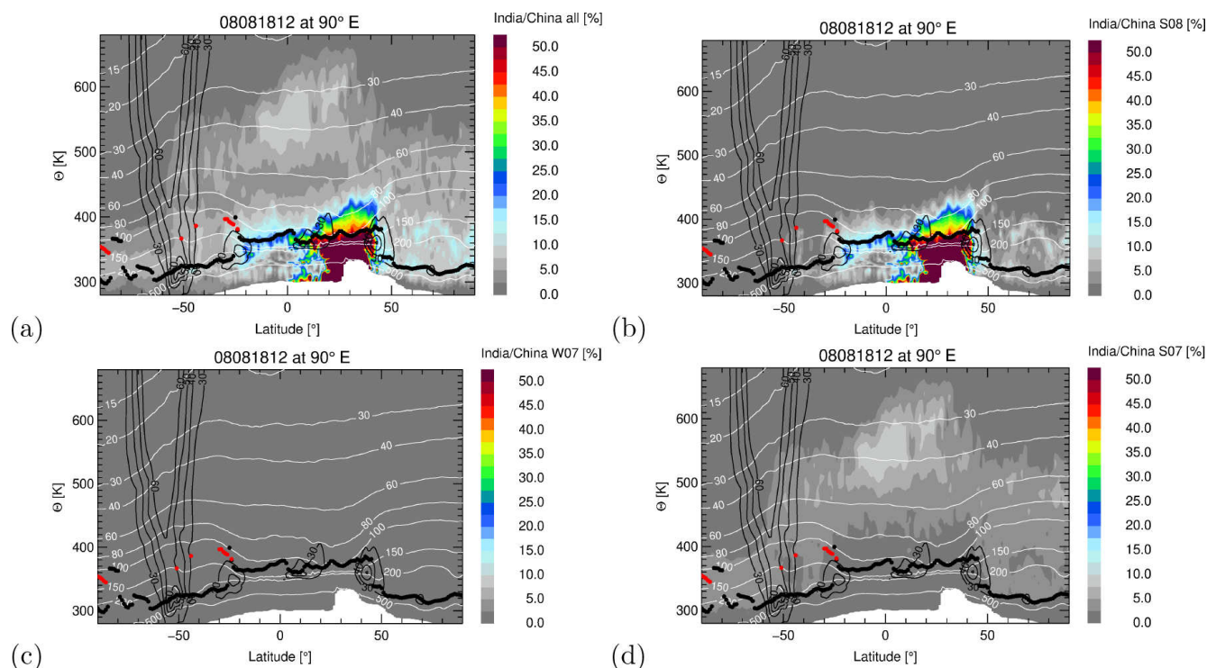
Figure 9. Latitude–theta cross sections at 90° E for the fraction of the India/China tracer for the simulation period (1 May 2007–18 August 2008 labelled as “all”) (a), for the summer 2008 (S08) pulse (b), for the winter 2007–2008 (W07) pulse (c), and for the summer 2007 (S07) pulse (d) on 18 August 2008. The thermal tropopause (primary in black dots and secondary in red dots) and absolute horizontal winds (black lines for 30, 40, 50, and 60 m s −1 ) are shown. The levels of pressure are marked by thin white lines. Note that the maximum value for the winter 2007–2008 (W07) pulse (c) is 2.4 %.
