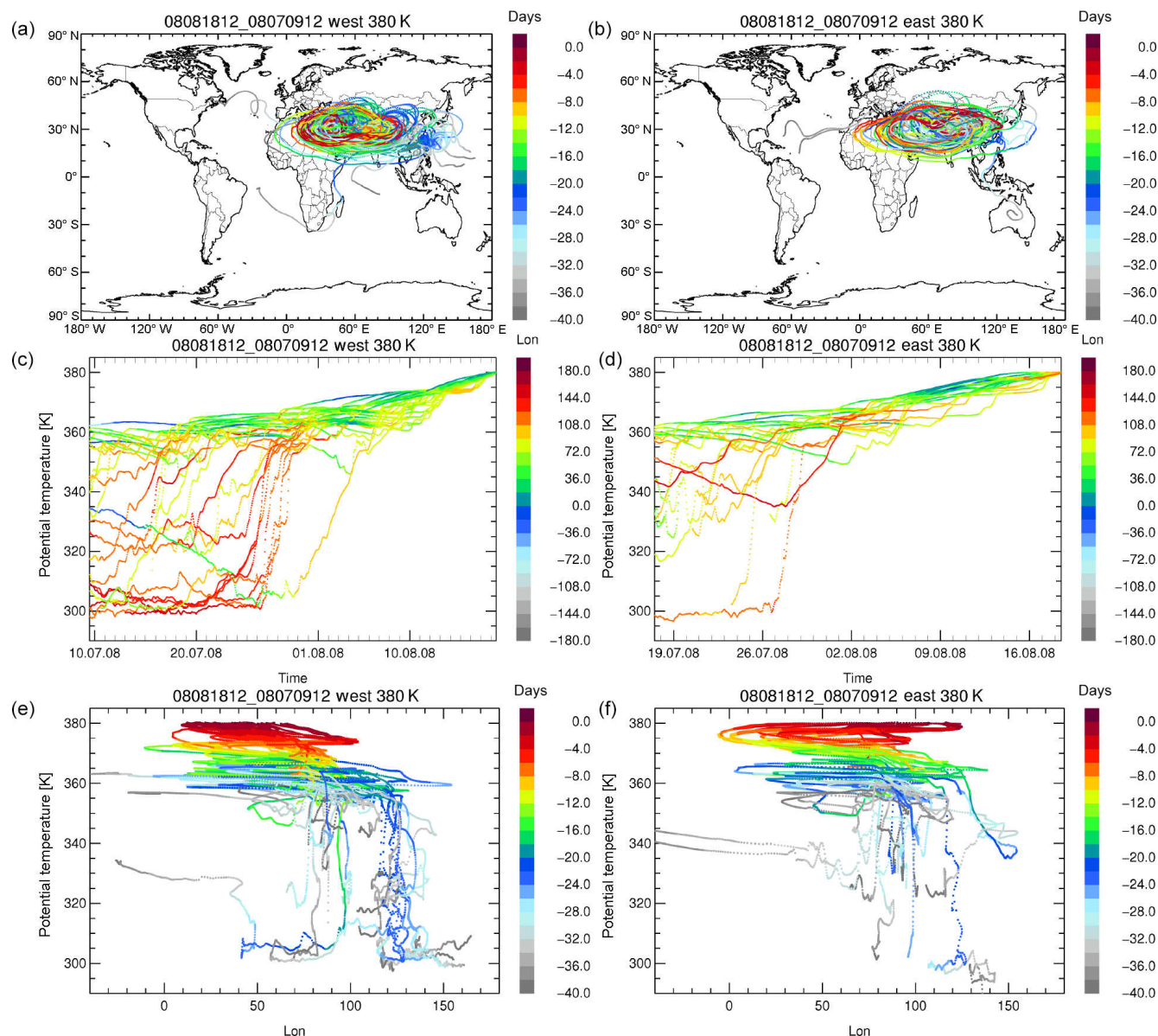
Figure 6. Different 40-day backward trajectories started at 380 K in the western ( a , c , e ) and eastern ( b , d , f ) mode of the Asian monsoon anticyclone are shown colour-coded by days back from 18 August 2008 ( a , b ). Further, potential temperature versus time (in UTC) along 40-day backward trajectories colour-coded by longitude ( c , d ) and potential temperature versus longitude, colour-coded by days back from 18 August 2008 ( e , f ) are shown. The trajectory positions are plotted every hour (coloured dots). Large distances between successive positions indicate rapid uplift.
