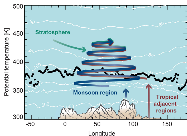
Figure 15. Longitude–theta cross section at about 30° N. At the top of the Asian monsoon anticyclone (above \sim 360 K) air masses circulate around the anticyclone in a large-scale upward spiral extending from northern Africa to the western Pacific. In the upward spiralling range air masses from inside the Asian monsoon anticyclone (shown in blue) are mixed with air masses convectively uplifted outside the core of the Asian monsoon anticyclone in the tropical adjacent regions, e.g. uplifted by tropical cyclones in the western Pacific ocean (shown in red). The higher the air masses are above the thermal tropopause, the larger the contribution of air masses is from outside the Asian monsoon anticyclone from the stratospheric background coming into the upward spiralling flow (shown in green). The levels of pressure are marked by thin white lines and the thermal tropopause is shown by black dots.
