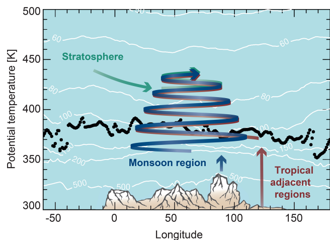
Figure 15. Longitude–theta cross section at about 30^{\circ} N. At the top of the Asian monsoon anticyclone (above \sim 360 K) air masses circulate around the anticyclone in a large-scale upward spiral extending from northern Africa to the western Pacific. In the upward spiralling range air masses from inside the Asian monsoon anticyclone (shown in blue) are mixed with air masses convectively uplifted outside the core of the Asian monsoon anticyclone in the tropical adjacent regions, e.g. uplifted by tropical cyclones in the western Pacific ocean (shown in red). The higher the air masses are above the thermal tropopause, the larger the contribution of air masses is from outside the Asian monsoon anticyclone from the stratospheric background coming into the upward spiralling flow (shown in green). The levels of pressure are marked by thin white lines and the thermal tropopause is shown by black dots.
