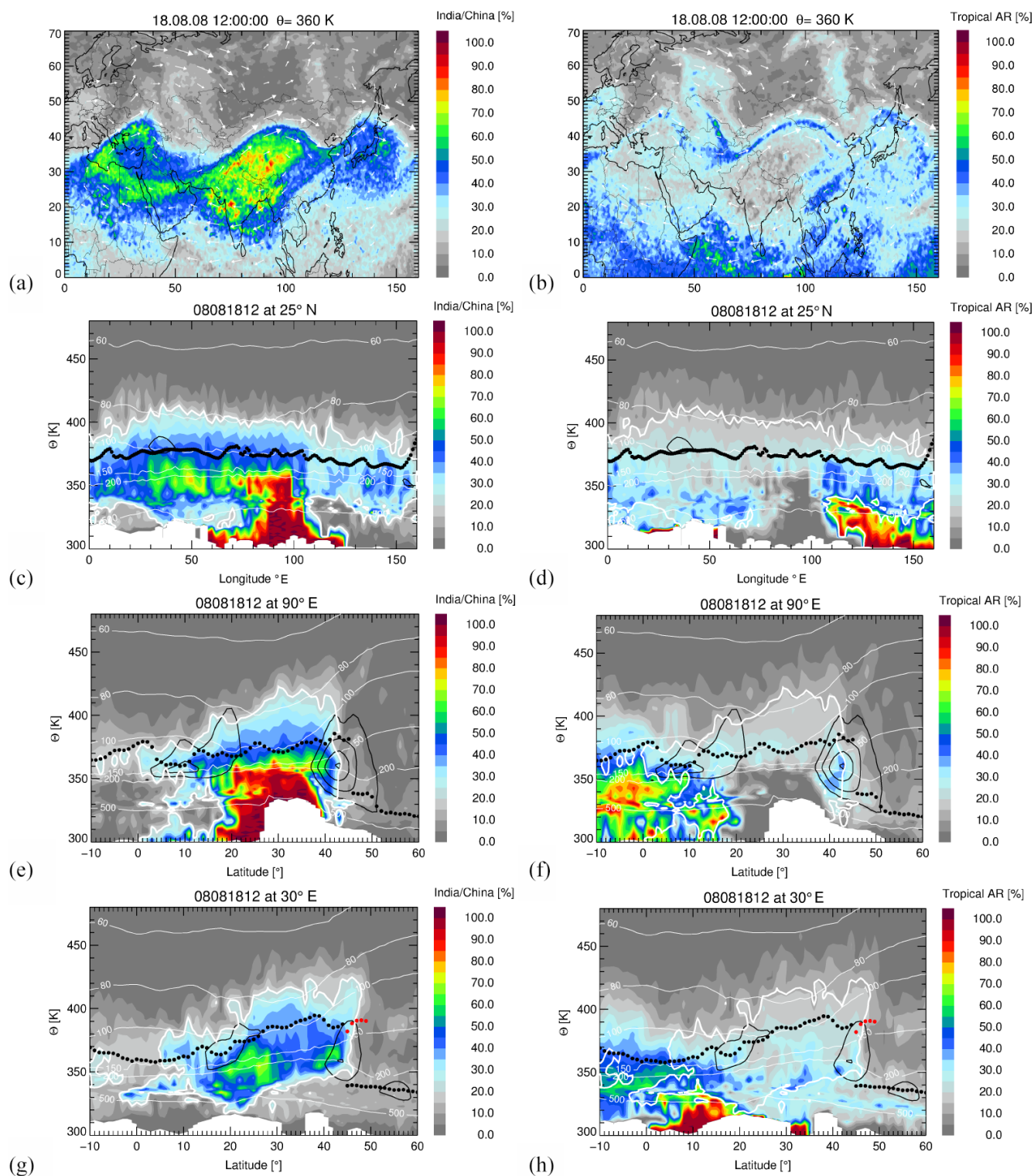
Figure 2. Horizontal distribution of the fraction of air originating in India/China (a, c, e, g) and in tropical adjacent regions (b, d, f, h) at 360 K potential temperature, longitude–theta cross sections at 25° N and latitude–theta cross sections at 90° E (eastern part of the anticyclone) and 30° E (western part of the anticyclone) on 18 August 2008. The horizontal winds are indicated by white arrows (maps) or by black thin lines (cross sections) (shown are 30, 40, 50, and 60 m s -1 ). The primary thermal tropopause is marked by black dots, the secondary thermal tropopause by red dots, and the levels of pressure are marked by thin white lines. The contour line of 20 % of the India/China tracer is shown by thick white lines (cross sections).
