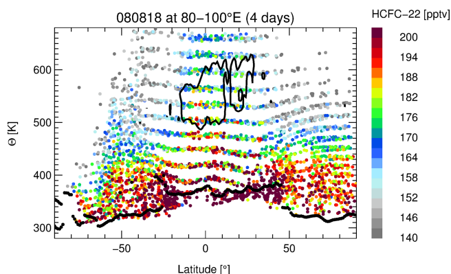
Figure 12. Latitude–theta cross sections of MIPAS HCFC-22 measurements crossing the eastern (80–100° E) mode of the anticyclone up to 680 K potential temperature on 18 August 2008. The thermal tropopause is indicated by black dots. The contour line of 6% of the India/China tracer for the summer 2007 pulse is shown by thick black lines as shown in Fig. 9. To highlight the MIPAS HCFC-22 signal within the tropical pipe the plot range of the data is up to 200 pptv. Note that the maximum values of MIPAS HCFC-22 in the troposphere are higher than 200 pptv.
