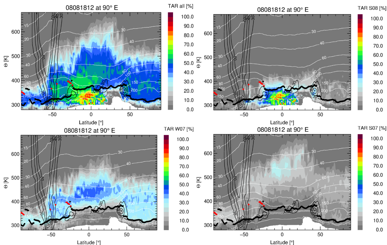
Figure 10. As Fig. 9 but for the fraction of the tracer for tropical adjacent regions (TAR).
