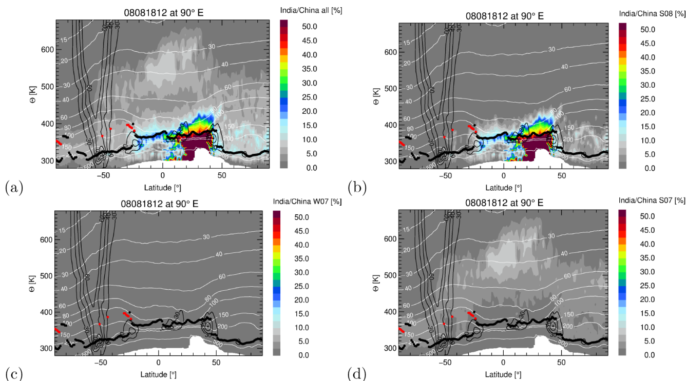
Figure 9. Latitude–theta cross sections at 90^\circ E for the fraction of the India/China tracer for the simulation period (1 May 2007–18 August 2008 labelled as “all”) (a), for the summer 2008 (S08) pulse (b), for the winter 2007–2008 (W07) pulse (c), and for the summer 2007 (S07) pulse (d) on 18 August 2008. The thermal tropopause (primary in black dots and secondary in red dots) and absolute horizontal winds (black lines for 30, 40, 50, and 60 \text{ m s}^{-1} ) are shown. The levels of pressure are marked by thin white lines. Note that the maximum value for the winter 2007–2008 (W07) pulse (c) is 2.4 %.
