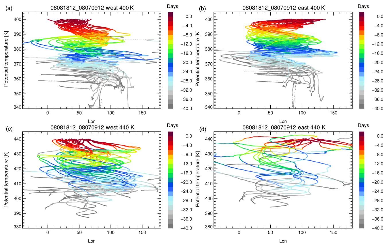
Figure 7. Potential temperature of different 40-day backward trajectories started at 400 K (a, b) and 440 K (c, d) in the western (a, c) and eastern (b, d) mode of the Asian monsoon anticyclone are shown versus longitude, colour-coded by days back from 18 August 2008.
