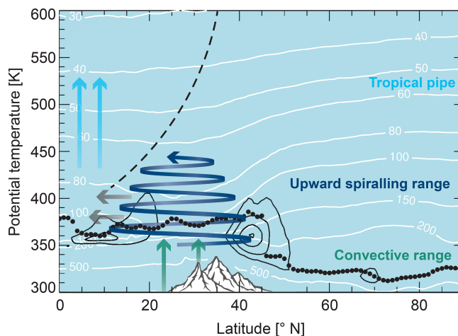
Figure 14. Latitude–theta cross section at about 90° E. The transport of air masses from the region of the Asian monsoon into the tropical pipe occurs in three distinct steps: first, very fast uplift within the convective range up to \sim 360 K within the Asian monsoon anticyclone and outside in the tropical adjacent regions (within a few days); second, uplift above 360 K (up to \sim 460 K) within the upward spiralling range (within a few months); and third, transport within the tropical pipe to altitudes higher than 460 K associated with the large-scale Brewer–Dobson circulation (within \sim 1 year). The thermal tropopause (black dots) and horizontal winds (black lines) are shown. The horizontal winds mark the edge of the anticyclone at its northern and southern flank. The levels of pressure are marked by thin white lines. Large grey arrows indicate isentropic transport from the Asian monsoon anticyclone into the tropics. The dashed line marks the tropical pipe, which largely isolates tropical air masses from isentropic mixing with mid-latitude air (e.g. Plumb, 1996; Volk et al., 1996).
