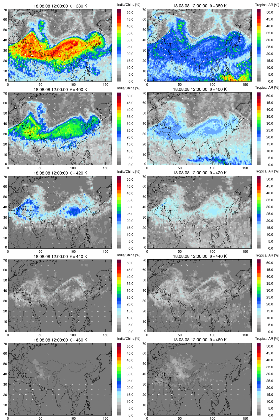
Figure 5. Horizontal distribution of the fraction of air originating in India/China (left) and in tropical adjacent regions (right) at 380, 400, 420, 440, and 460 K potential temperature.
