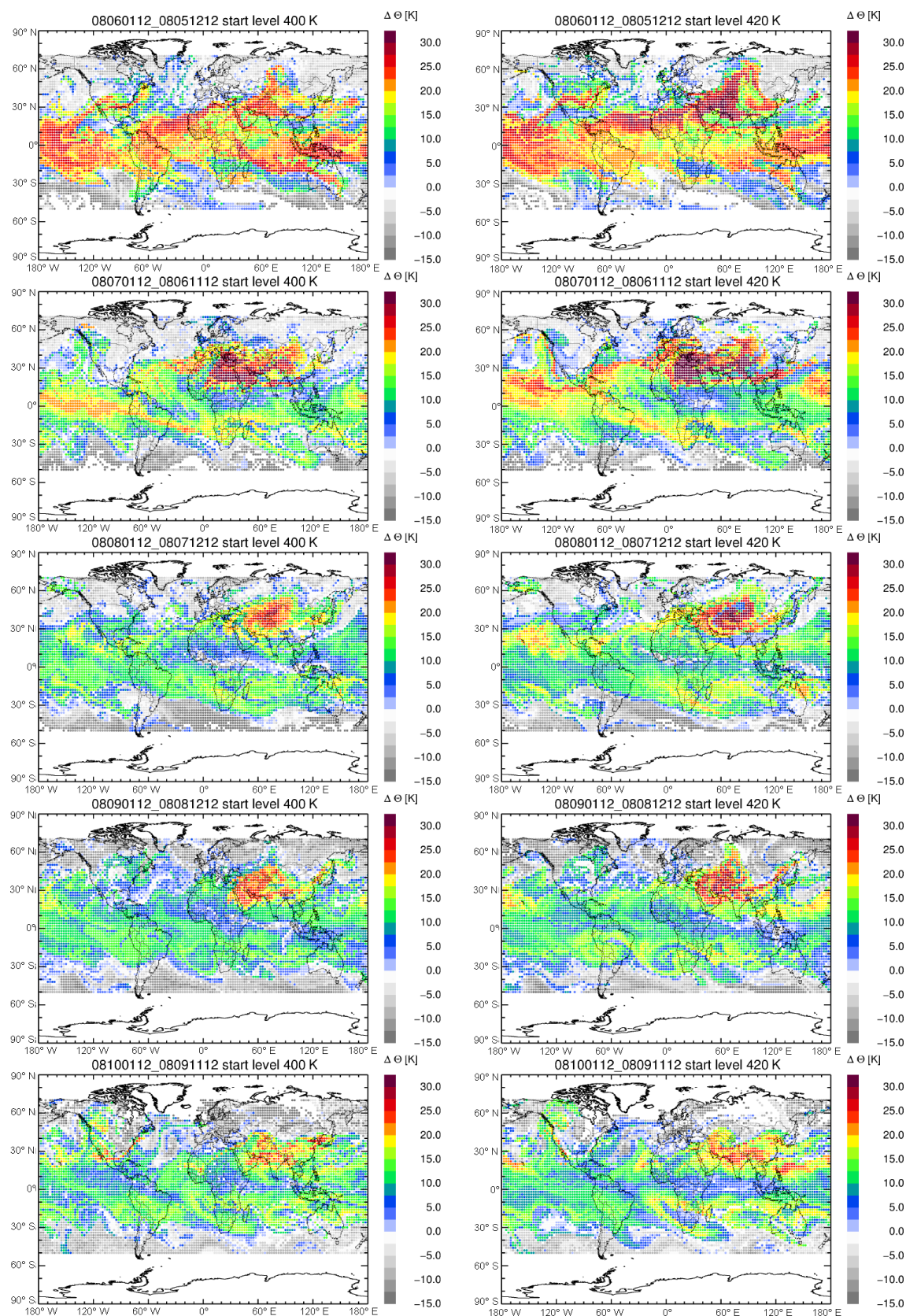
Figure A1. The change in potential temperature ( \Delta\Theta ) along 20-day backward trajectories are shown for different levels of potential temperature (400 and 420 K) for different days from monsoon onset until post-monsoon (1 June, 1 July, 1 August, 1 September, and 1 October 2008).
