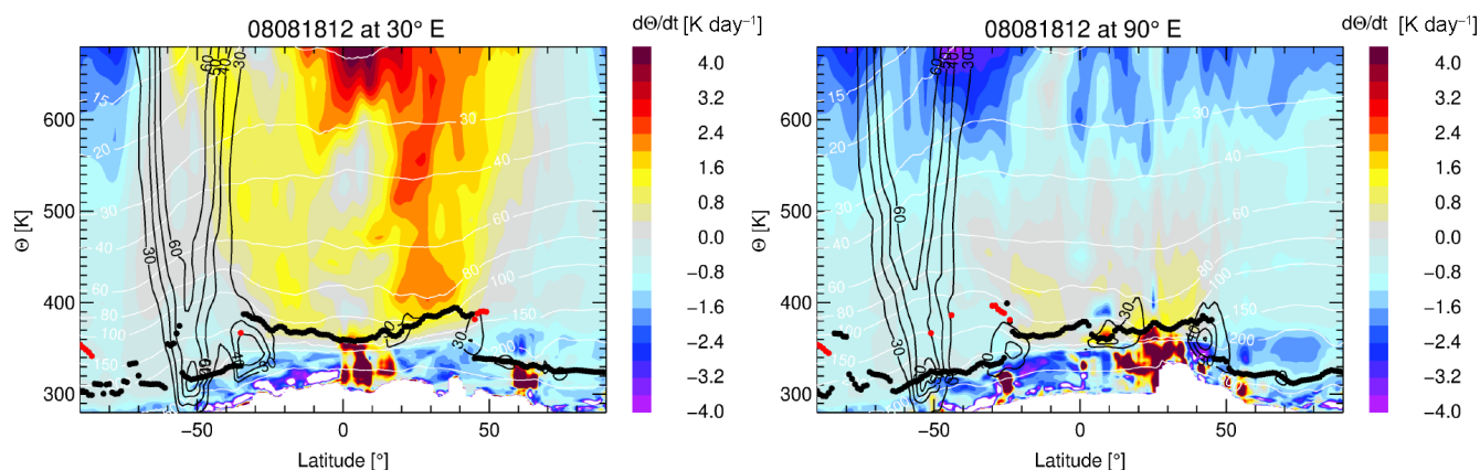
Figure 11. Latitude–theta cross section of d\Theta/dt showing the radiative heating above the Asian monsoon anticyclone for the western ( 30^\circ E) and eastern mode ( 90^\circ E) of the anticyclone on 18 August 2008. The thermal tropopause (primary in black dots and secondary in red dots) and absolute horizontal winds (black lines for 30, 40, 50, and 60 \text{ m s}^{-1} ) are shown. The pressure levels are marked by thin white lines.
