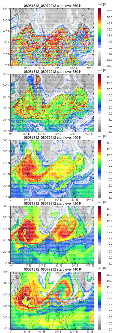
Figure 8. The change in potential temperature ( \Delta\Theta ) along 20-day backward trajectories initialised on 18 August 2008 is shown for different levels of potential temperature (360, 380, 400, 420, and 440 K). Note that the range of the colour bar in the first panel is much larger than in the other panels. At the lower potential temperature levels (360, 380 K), some 20-day backward trajectories exist that reach the model boundary layer within a time period shorter than 20 days (in cases of very strong uplift by convection). For these trajectories \Delta\Theta is shown for the shorter time period.
