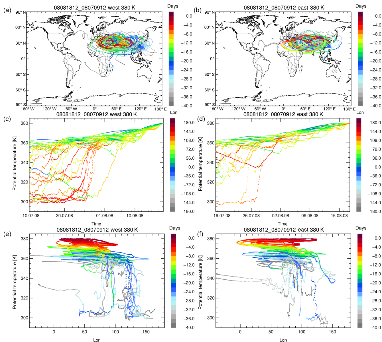
Figure 6. Different 40-day backward trajectories started at 380 K in the western (a, c, e) and eastern (b, d, f) mode of the Asian monsoon anticyclone are shown colour-coded by days back from 18 August 2008 (a, b). Further, potential temperature versus time (in UTC) along 40-day backward trajectories colour-coded by longitude (c, d) and potential temperature versus longitude, colour-coded by days back from 18 August 2008 (e, f) are shown. The trajectory positions are plotted every hour (coloured dots). Large distances between successive positions indicate rapid uplift.
