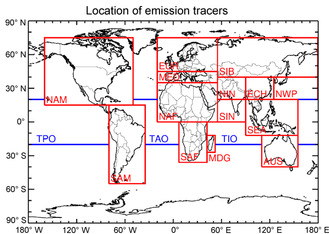
Figure 1. Global geographical location of artificial boundary layer source regions in the CLaMS model, also referred to as “emission tracers”, adapted from Vogel et al. (2015). The latitude and longitude range for each emission tracer is listed in Table 1.
