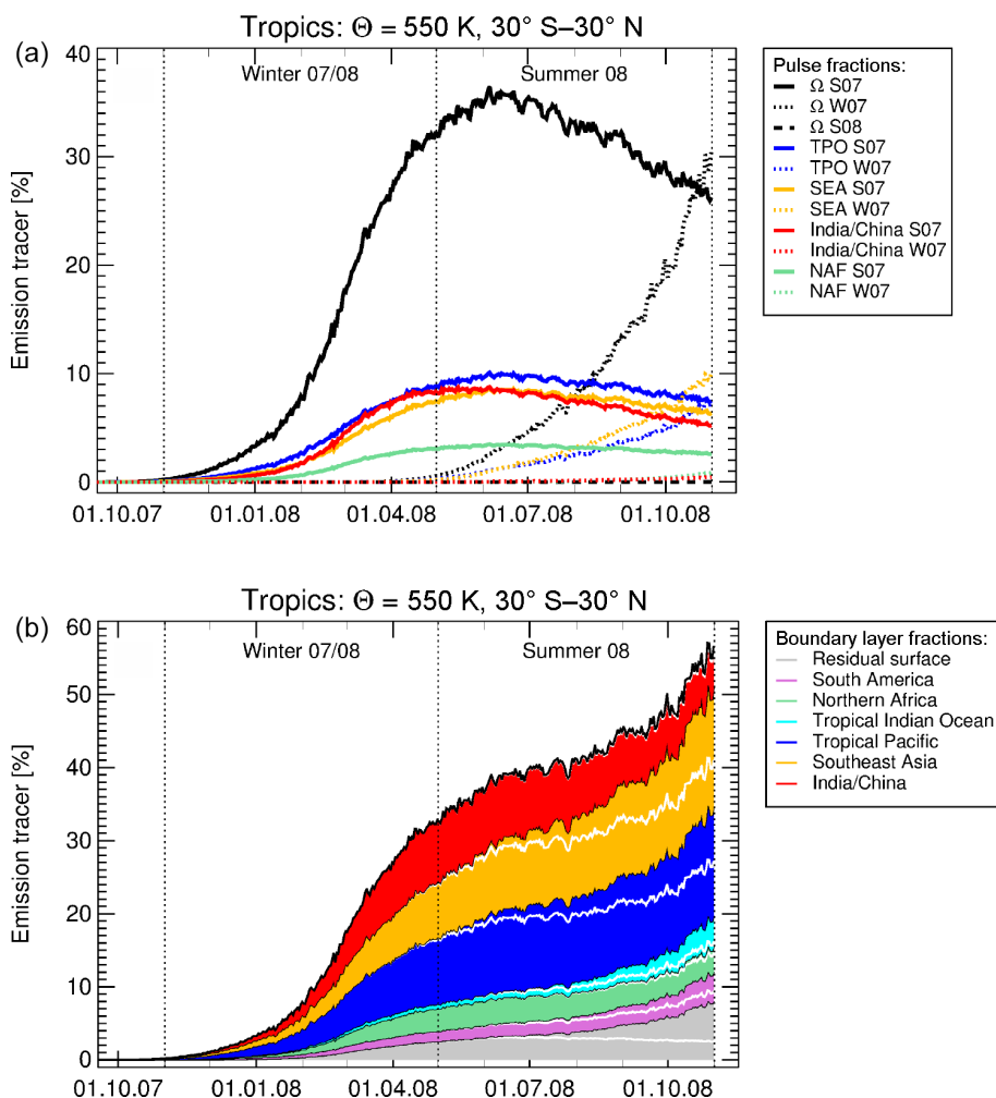
Figure 13. (a) The contribution of the three different time pulses S07, W07, and S08 (each set for a time period of 6 months marked by the vertical dotted lines) for the entire Earth's surface ( \Omega_{S07} , \Omega_{W07} , \Omega_{S08} ) to the tropical pipe between 30° S and 30° N at 550 K potential temperature from 1 October 2007 until the end of the simulation period (31 October 2008) (black lines). Emission tracers released during S08 have no contribution to the tropical pipe at 550 K by October 2008. The contribution of several tracers of air mass origin to the individual pulses are shown by coloured lines. (b) Contribution of different emission tracers for the tropical Pacific Ocean, Southeast Asia, India/China, South America, northern Africa, tropical Indian Ocean, and the residual surface (all other regions of the Earth's surface) to the tropical pipe between 30° S and 30° N at 550 K potential temperature from 1 October 2007 until the end of the simulation period. The contribution of the time pulses for the different emission tracers are marked by thin white lines for S07 and by thin black lines for W07.
