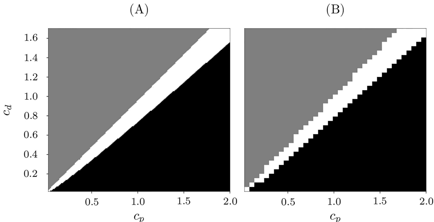
Fig 13. Parameter (c_p, c_d) -plane of the plasticity function. Panel (A): system (10)–(11). White region: stable periodic solution coexisting with a stable fixed point, case II. Black region: globally stable fixed point, case I. Grey region: globally stable periodic solution with \sigma = 0 . Panel (B): original system (1)–(3). White: stable two-clusters (white); black: stable synchrony and no stable clusters; grey: decoupling of all neurons. Other parameters \tau_p = 2 , \tau_d = 5 , N = 50 , N_s = 7 , and \kappa_{\max} = 1 .
