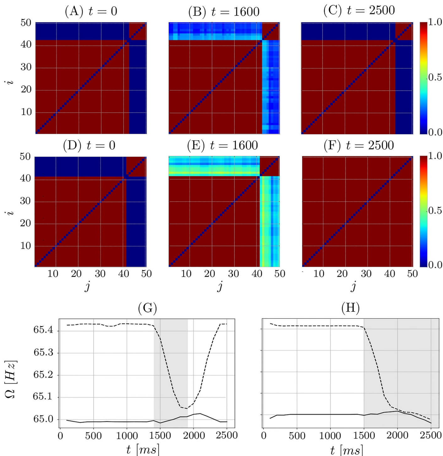
Fig 8. Two cases: Fusion and stable clusters. Evolution of the coupling matrix for N = 50 and the number of neurons N_s = 8 (A)-(C) and N_s = 9 (D)-(F) in the small cluster. In panels (A)-(C) the clusters are stable, while in (D)-(F) they are merging to one synchronous cluster. (G, H) Time courses of the spiking synchronization frequencies of small ( N_s neurons) and large ( N_b neurons) clusters depicted by dashed and solid curves, respectively, for (G) N_s = 8 and N_b = 42 and (H) N_s = 9 and N_b = 41 . Parameter \kappa_{max} = 1.0 .
