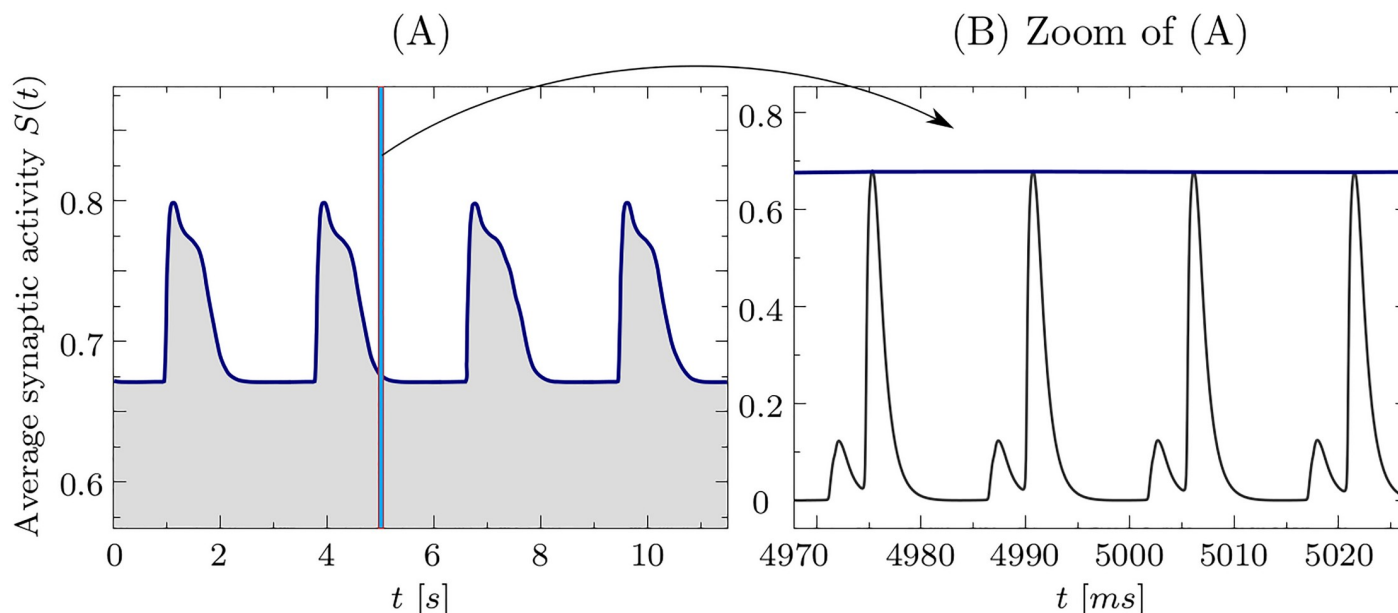
Fig 9. Mean synaptic activity. Mean synaptic activity S(t) of the neural population in the case of stable two cluster state. Panel (A) shows the dynamics of S(t) on the time interval of 12 s, where modulation of the amplitude (blue line) is visible, while the fast oscillations are not recognized on this timescale. The maximum amplitude corresponds to the two clusters being synchronised, while the low amplitude corresponds to the clusters being out of phase. Panel (B) shows the zoom of a small time interval. The modulation takes place on the timescale which is two orders of magnitude larger than the individual spikes of S(t) as well as individual neural spikes in both clusters. Cluster frequencies \omega_1 = 0.065012 kHz and \omega_2 = 0.065416 kHz. The corresponding period of modulation is T \approx 2.5 s.
