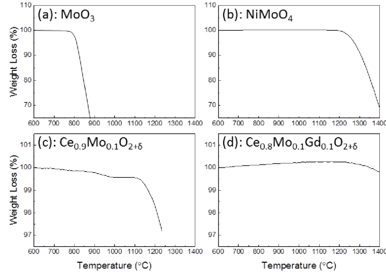
Figure 5.14: TGA result of Mo precursor: MoO 3 (a), NiMoO 4 (b), Ce 0.9 Mo 0.1 O 2+δ (c), and Ce 0.8 Mo 0.1 Gd 0.1 O 2+δ (d)
