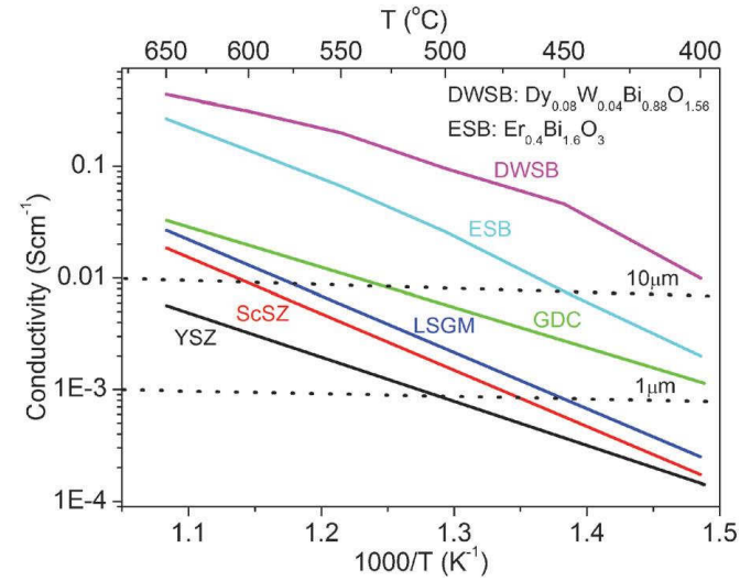
Figure 2.4: Specific ionic conductivity of various SOFC electrolyte materials [31]
