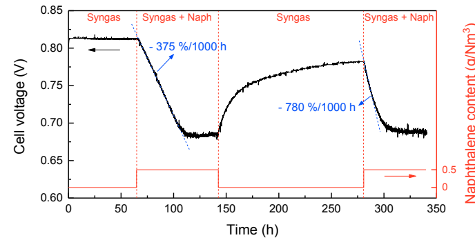
Figure 4.8: Voltage-time plot of syngas + naphthalene test (NAPH) at 700 °C, 0.34 A/cm 2
