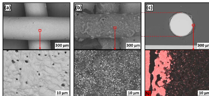
Figure 4.22: SEM images of contacting Ni mesh on the interconnect with low (upper images) and high (bottom images) magnification, the clean Ni mesh image of (a) was achieved from the area 4 and carbon covered mesh images of (b) and (c) were achieved from area 5 in Figure 4.19
