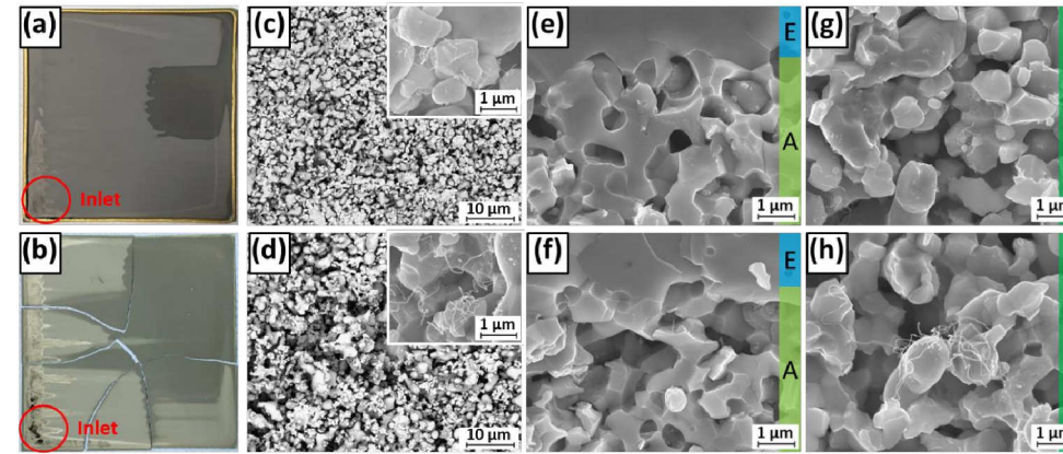
Figure 5.11: Support photo, surface, and fractured cross-section SEM images of the support inlet after the 2g/Nm 3 phenol test (a-d) and the 1-8 g/Nm 3 phenol test (e-h)
