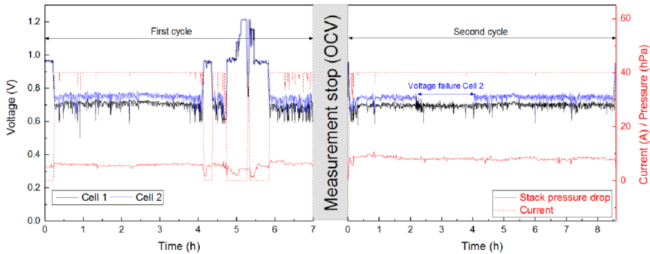
Figure 4.17: Stack test result with clean-syngas at 715 °C, 0.5 A/cm 2
