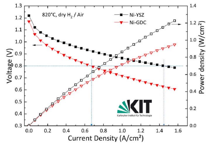
Figure 5.9: Single cell measurement result of the Ni/GDC anode cell (Measured at KIT IAM-WET by N. Russner) [150]
