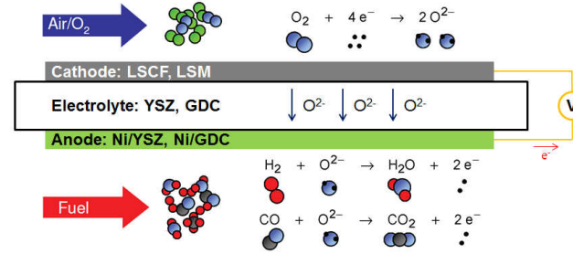
Figure 2.2: Schematic illustration of structure and working principle of SOFCs
