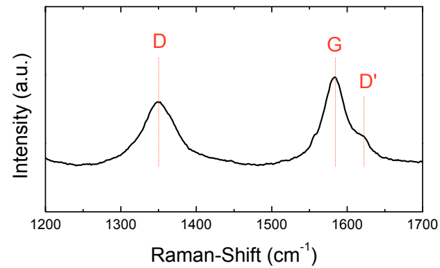
Figure 4.11: Raman spectra of the cell support inlet surface after the NAPH test
