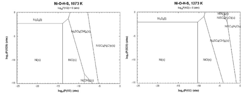
Figure 2.9: Ni–O–H–S diagrams in thermodynamic equilibrium at (a) 800 and (b) 1000 °C [15]
