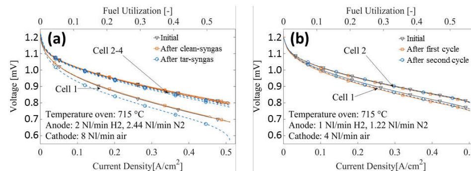
Figure 4.18: I-V characterization before, intermediate, and after stack test with clean- and tar-syngas (a, correspond to Figure 4.16) and clean-syngas (b, correspond to Figure 4.17)
