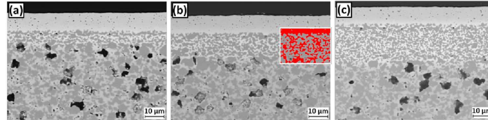
Figure 5.1: The cross-section SEM image of Ni/GDC anode half-cells with different numbers of screen printing: (a) single, (b) double, and (c) triple layer (NiO to GDC ratio: 60/40 wt%)
