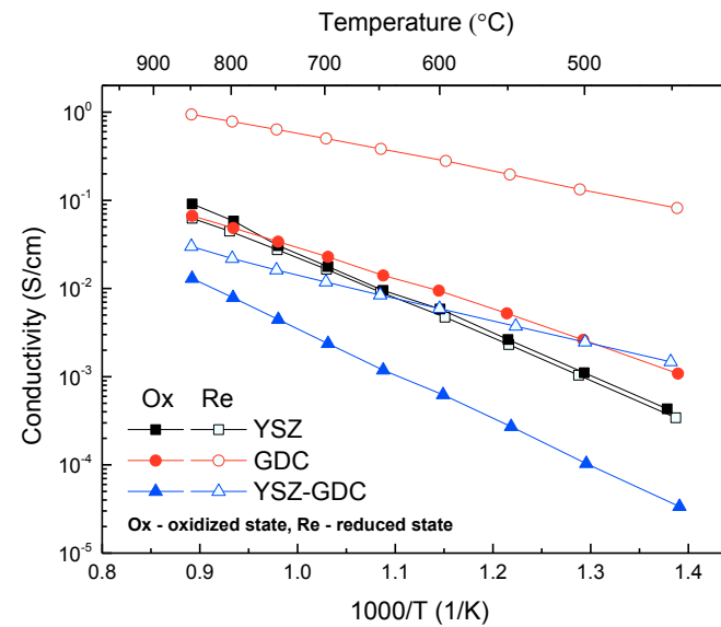
Figure 5.7: Temperature-conductivity plot of YSZ (black), GDC (red), and YSZ-GDC (blue) phases; the conductivities were measured in both oxidized (closed symbol) and reduced (open symbol) state [150]
