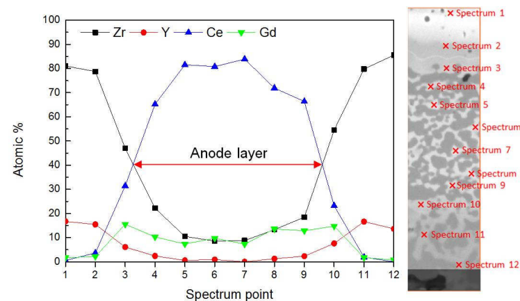
Figure 5.4: Point EDX result of the Ni/GDC half-cell after sintering and SEM image with different measurement position
