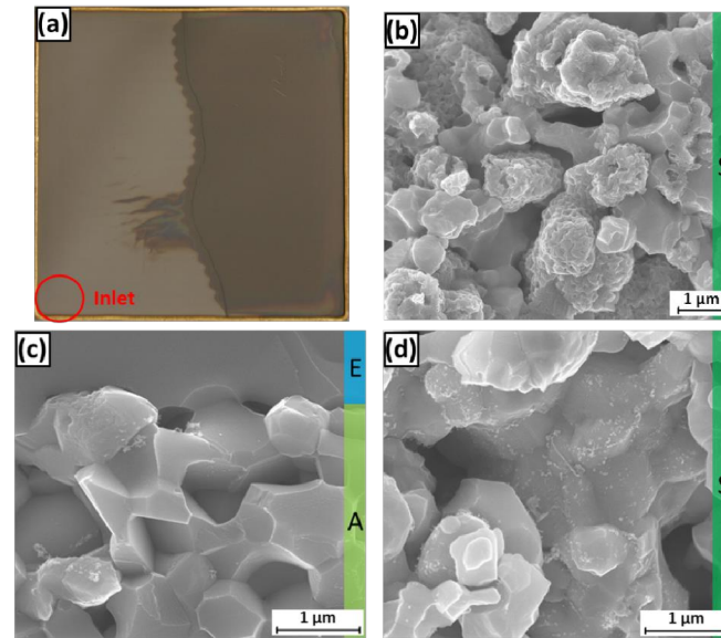
Figure 4.9: Cell photo (a) and fractured cross-sectional SEM images of outlet support (b), inlet electrolyte and anode (c), and inlet support (d) after the NAPH test
