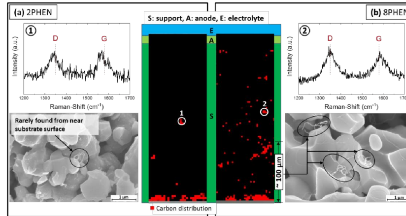
Figure 4.7: Carbon deposition analysis of fractured cell cross-section after 2PHEN and 8PHEN test; carbon distribution mapping by Raman with example spectra and carbon fibers observation by SEM
