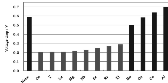
Figure 2.11: Cell voltage drop with various additives impregnated in porous anode layers at 200 \text{mA}/\text{cm}^2 800 ^\circ\text{C} , \text{H}_2\text{S} conc. = 20 ppm, \text{H}_2/\text{CO} = 100:0 , electrolyte/ScSZ, anode/Ni-YSZ + additives [15]
