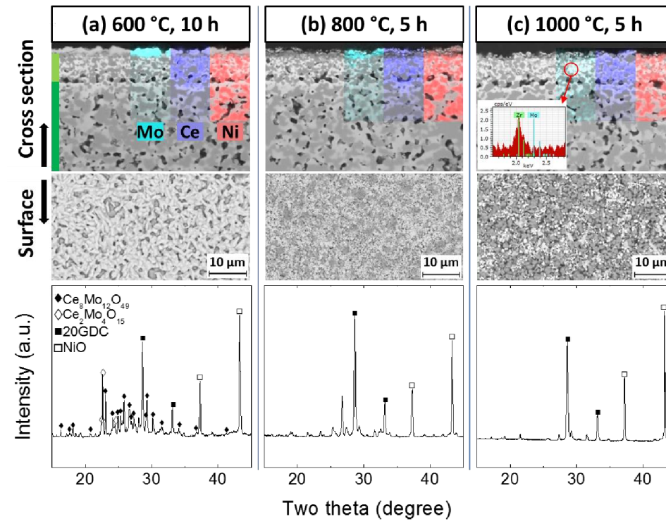
Figure 5.19: The microstructure and phase analysis result of Ni/GDC anode after \text{MoO}_3 treatment with different heat treatment 600 °C, 10 h (a), 800 °C, 5 h (b), and 1000 °C, 5 h (c)
