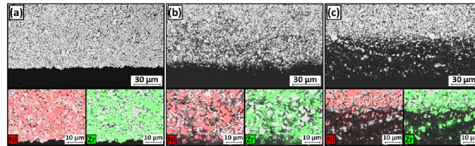
Figure 4.21: Polished cross sectional SEM images and EDX element mapping results of the cell supports, the figure labels (a), (b), and (c) are correspond with the area of 1, 2, and 3 in Figure 4.19
