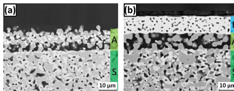
Figure 5.15: SEM images of half-cell after sintering with anode composition of \text{Ni/Ce}_{0.8}\text{Mo}_{0.1}\text{Gd}_{0.1}\text{O}_{2+\delta} (a) and \text{Ni/Ce}_{0.85}\text{Mo}_{0.05}\text{Gd}_{0.1}\text{O}_{2+\delta} (b)
