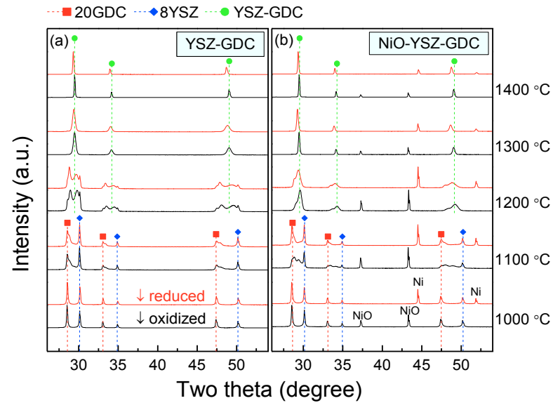
Figure 5.5: XRD result of the YSZ-GDC (a) and NiO-YSZ-GDC (b) powder mixtures after sintering at different temperatures of 1000, 1100, 1200, 1300, and 1400 °C; the red line shows the XRD result after reducing at 900 °C for 5 h in 2.9 % H 2 /Ar
