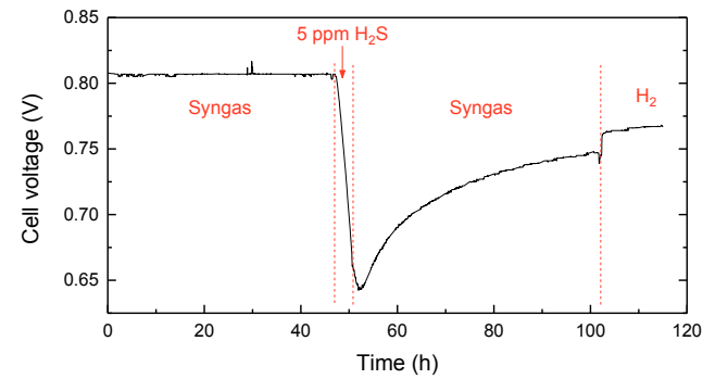
Figure 4.12: Voltage-time plot of syngas + H 2 S test at 700 °C, 0.34 A/cm 2
