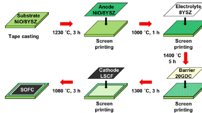
Figure 3.1: Manufacturing process of JÜLICH standard anode-supported cell
