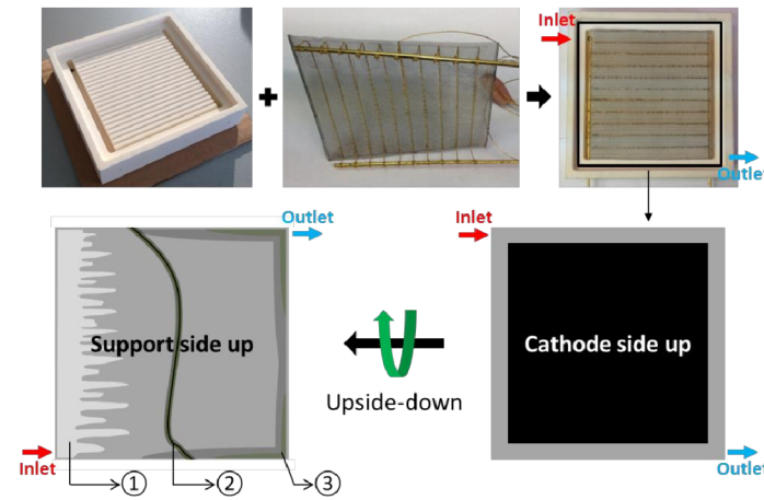
Figure 3.6: Photos of the alumina housing, contact material, and the schematic diagram of the cell after testing
