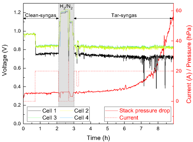
Figure 4.16: Stack test result with cleaned syngas (tar, sulfur, and chlorine removed) and tar-syngas (sulfur and chlorine removed) at 715 °C, 0.25 A/cm 2 . Note: the voltage curves of cell 2 to 4 (yellow, green, and blue) overlap completely
