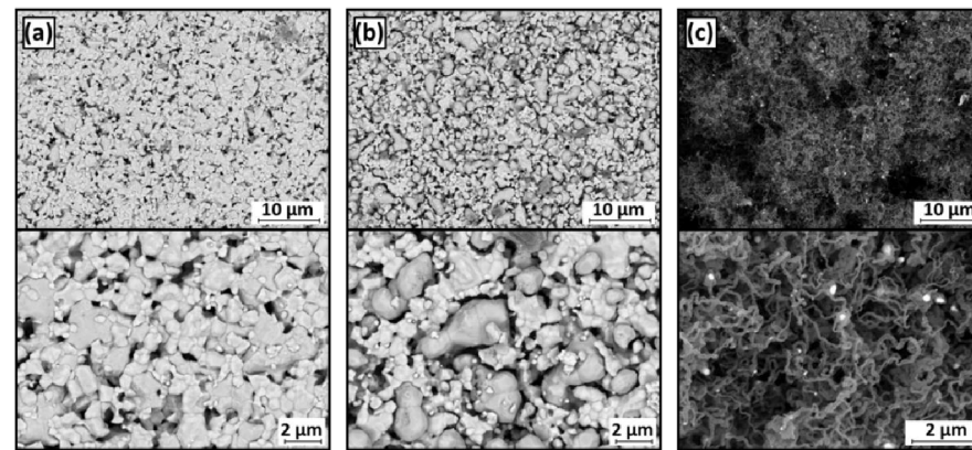
Figure 4.20: Surface SEM images of anode support with low (upper images) and high (below images) magnification from different positions, the figure labels (a), (b), and (c) are correspond with the area of 1, 2, and 3 in Figure 4.19
