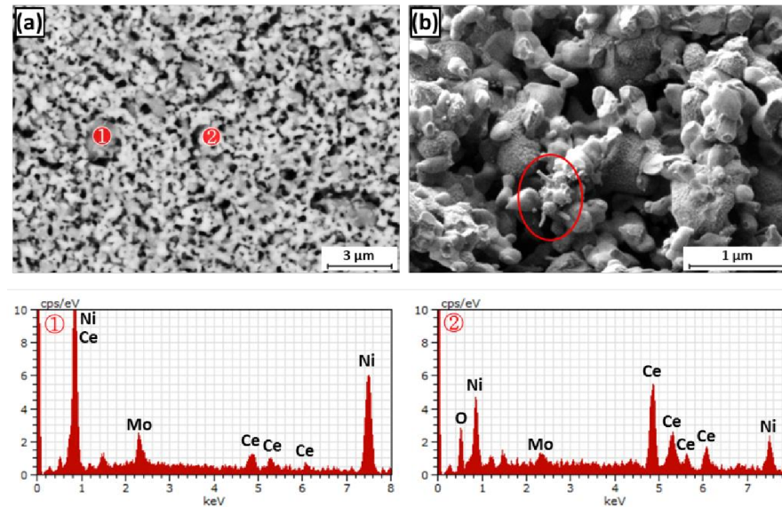
Figure 5.21: SEM images of Ni/GDC anode with Mo infiltration and the point EDX result of Ni (1) and GDC (2) particles
