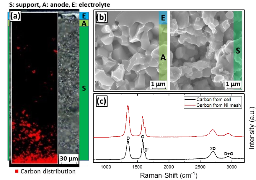
Figure 4.23: Carbon distribution mapping result of fractured cell cross-section by Raman spectroscopy (a), SEM images of fractured cell cross-section (b), and Raman shift result of carbon from cell surface and contacting Ni mesh (c)
