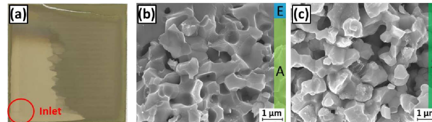
Figure 5.12: Support photo and fractured cross-section SEM images after of support inlet 0.5 g/Nm 3 naphthalene test
