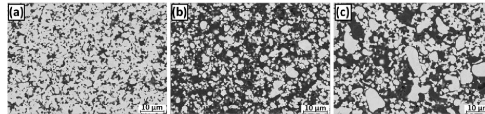
Figure 4.4: Polished cross-section of the cell supports in the fuel inlet area after SYN test (a), 2PHEN test (b), and 8PHEN test (c)
