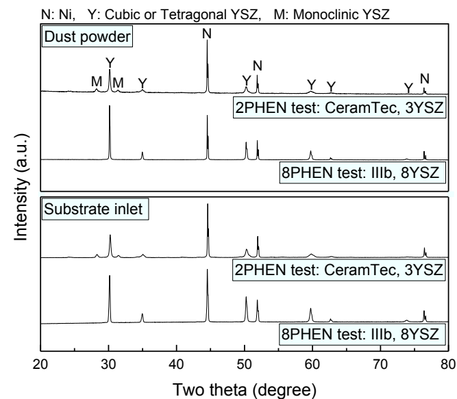
Figure 4.5: XRD results of the support in the area of the fuel inlet and the powder collected from the alumina housing after PHEN test
