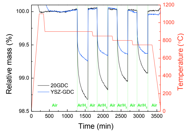
Figure 5.6: TGA analysis of the reduction in GDC (black line) and a GDC–YSZ mixed phase sintered at 1400°C (blue line); the dotted green lines indicate a change in the gas atmosphere [150]
