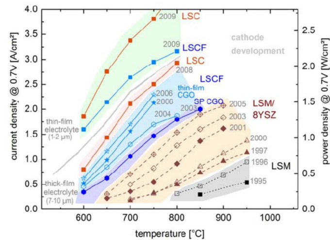
Figure 2.5: Current density as function of operating temperature for single cell tests with various cathode materials [37]
