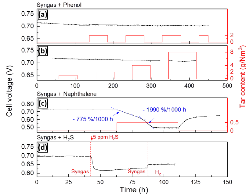
Figure 5.10: Ni/GDC anode cell single measurement result with syngas + phenol (a and b), syngas +naphthalene (c), and syngas + H 2 S (d) at 700 °C, 0.34 A/cm 2
