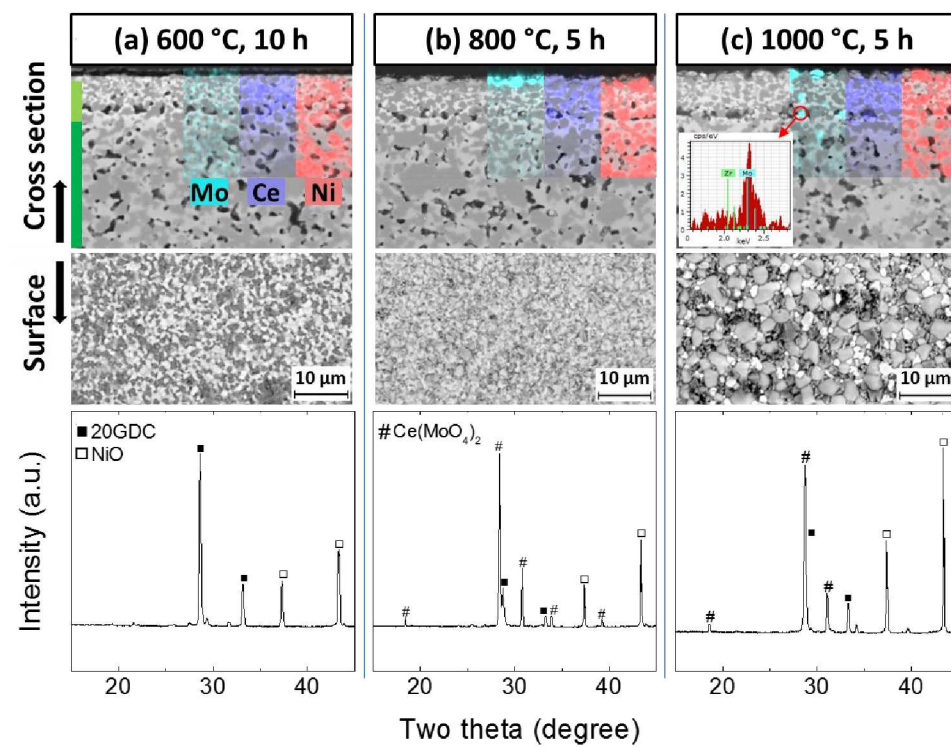
Figure 5.20: The microstructure and phase analysis result of Ni/GDC anode after \text{NiMoO}_4 treatment with different heat treatment 600 °C, 10 h (a), 800 °C, 5 h (b), and 1000 °C, 5 h (c)
