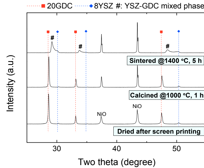
Figure 5.3: XRD result of the Ni/GDC anode layer on the Ni/GDC support
