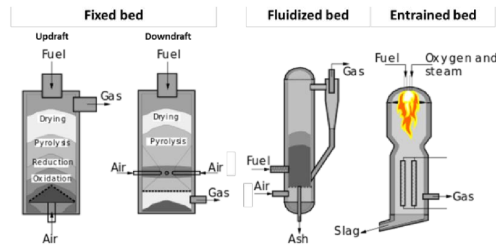
Figure 2.7: Schematic diagrams of type of gasifiers
