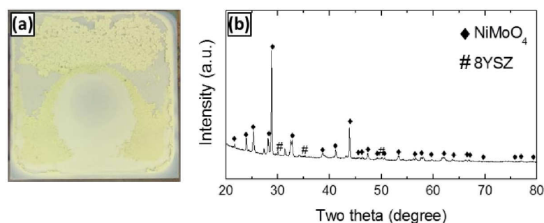
Figure 5.16: XRD result of the yellow powder on the support surface after the gas infiltration process
