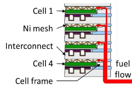
Figure 3.2: Schematic diagram of stack structure with a direction of fuel gas flow
