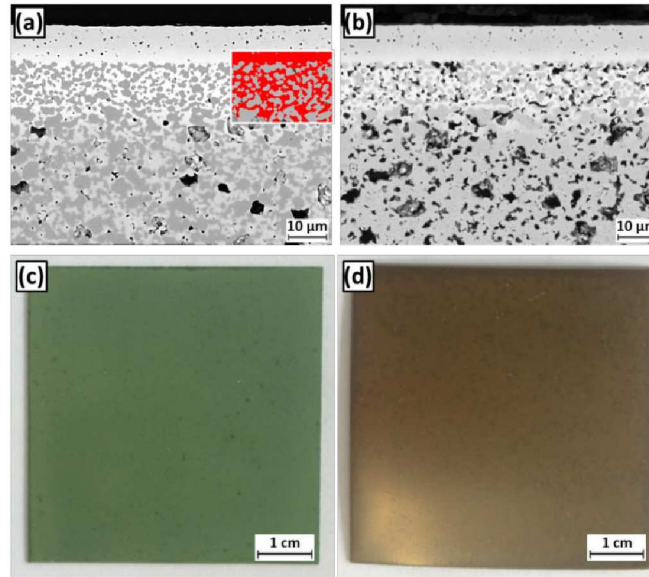
Figure 5.2: Cross-sectional SEM image of Ni/GDC anode half-cell with 50 to 50 composition (a) oxidized and (b) reduced state, and the picture of the cell (c) oxidized and (d) reduced state
