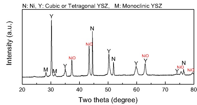
Figure 4.10: XRD result of the Ni/YSZ support surface in the outlet area after the NAPH test
