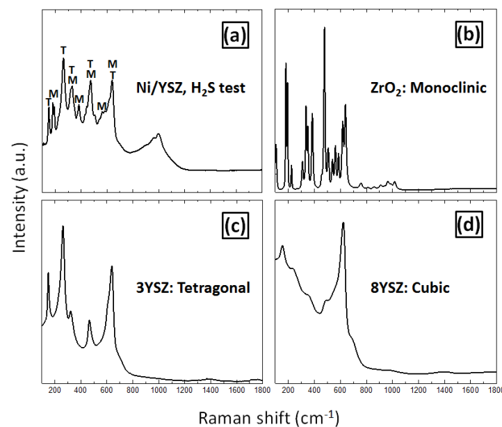
Figure 4.15: Raman spectra of the Ni/YSZ support after the H 2 S test (a), and the reference zirconia spectra of ZrO 2 (b), 3YSZ (c), and 8YSZ (d)
