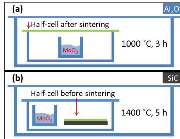
Figure 3.3: Schematic diagram of the MoO 3 gas infiltration experiment setup
