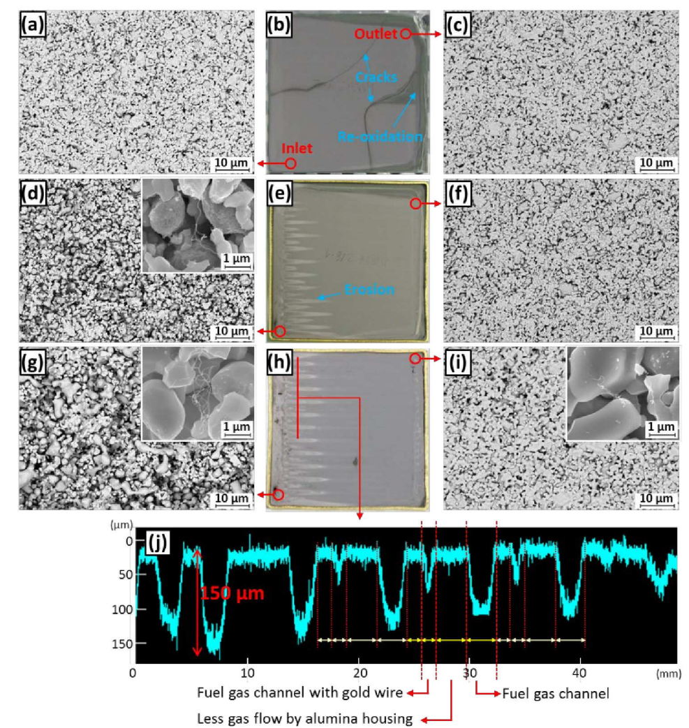
Figure 4.3: Support surface photos and SEM images after SYN test (a-c), 2PHEN test (d-f), and 8PHEN test (g-i), and a depth profile of the erosion pattern on the surface of the support after 8PHEN test (j).
