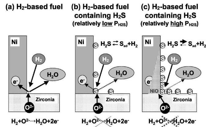
Figure 2.10: Sulfur poisoning mechanisms: (a) \text{H}_2 -based fuel containing no \text{H}_2\text{S} , (b) \text{H}_2 -based fuel with relatively low P_{\text{H}_2\text{S}} , and (c) \text{H}_2 -based fuel with relatively high P_{\text{H}_2\text{S}} [15]
