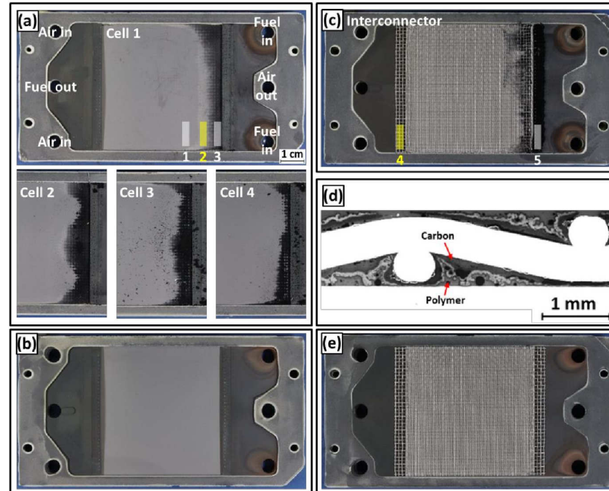
Figure 4.19: The photo of cells with frame after tar-syngas test (a), clean-syngas test (b); the photo of interconnects after tar-syngas test (c), and clean-syngas test (e); the cross-sectional optical microscope image of contacting Ni mesh (d)
