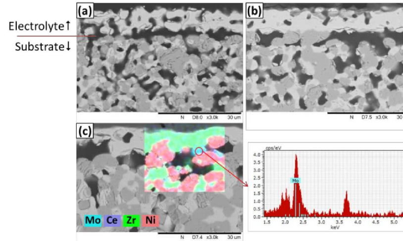
Figure 5.18: The cross-section SEM image of a sintered half-cell in \text{MoO}_3 atmosphere with different \text{MoO}_3 loading: 0.1 (a), 0.2 (b), and 0.5 (c) g
