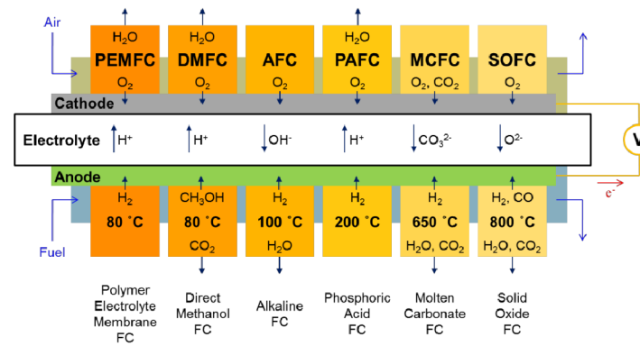
Figure 2.1: Schematic diagram of various types of fuel cells
