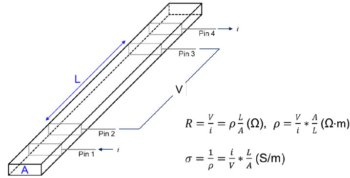
Figure 3.5: Schematic diagram of the four point-probe method
