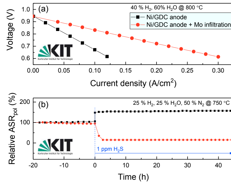
Figure 5.22: Single cell measurement results of the ESC cell with the Ni/GDC anode with and without Mo infiltration and relative ASR (Measured at KIT IAM-WET by N. Russner)
