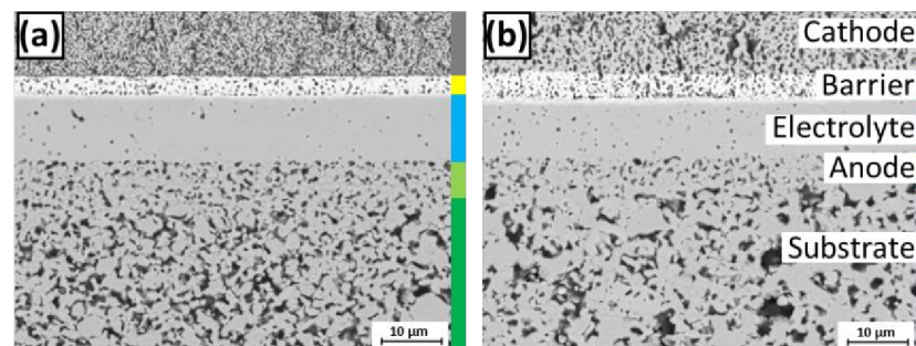
Figure 4.1: Cross-sectional SEM images of (a) CeramTec and (b) IIIb full cell structures in reduced state
