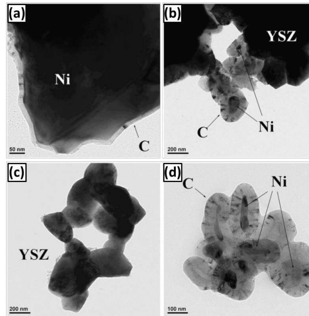
Figure 2.8: Transmission electron microscope result of the Ni/YSZ anode operated with syngas for 15 min (a) and 2 h (b-c) [64]
