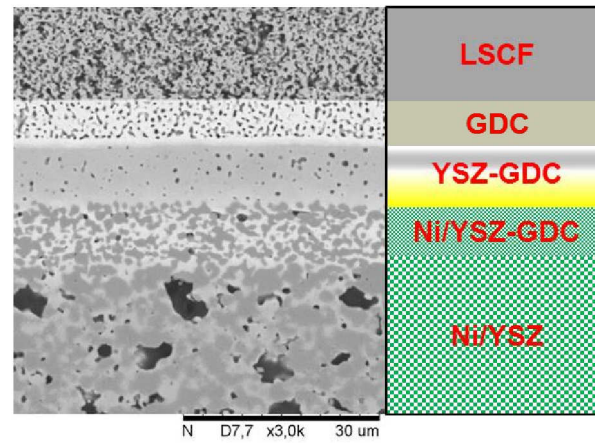
Figure 5.8: Microstructure and schematic diagram of the Ni/GDC anode full-cell
