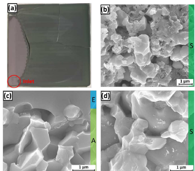
Figure 4.13: Cell photo (a) and fractured cross-sectional SEM images of the outlet support (b), inlet electrolyte and anode (c), and inlet support (d) after the H 2 S test
