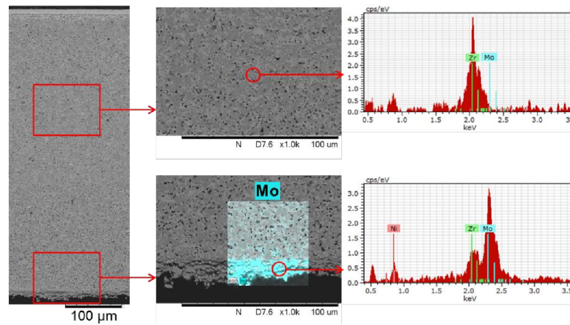
Figure 5.17: The cross-section SEM image and EDX result of the half-cell after the MoO 3 gas infiltration at 1000 °C for 3 h
