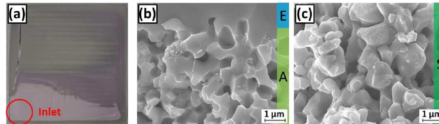
Figure 5.13: Support photo and fractured cross-section SEM images of the support inlet after the 5 ppm H 2 S test
