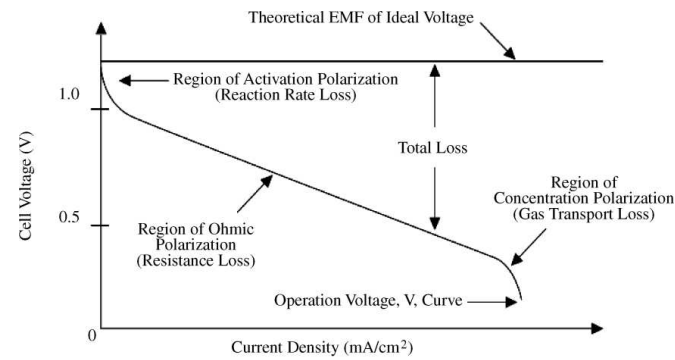
Figure 2.3: Ideal and actual performance of a fuel cell with respect to the potential current response [20]
