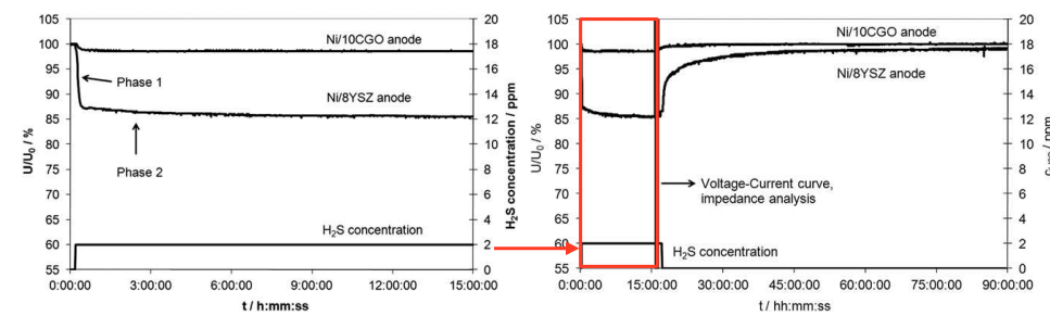
Figure 2.12: Comparison of the ratios of the contaminated stack voltages to initial voltages with respect to time with Ni/8YSZ and Ni/10CGO anodes during and after 2 ppm H_2S contamination at 850 °C [76]
