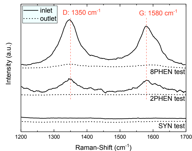
Figure 4.6: Raman spectra of cell support inlet (solid line) and outlet (dotted line) area after SYN test, 2PHEN test, and 8PHEN tests
