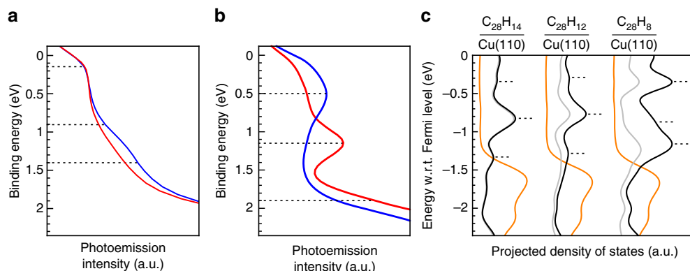
Fig. 2 Valence band of DBBA on Cu(110) before and after annealing at 250 °C. a Energy distribution curves (EDCs) of as-deposited DBBA measured along [001] (blue curve) and [110] (red curve) directions of Cu(110). b EDCs after annealing of DBBA at 250 °C measured along [001] direction of Cu(110) (blue curve) and 25° away from [110] direction (red curve). For the EDCs, the photoelectron intensity was integrated over the polar angle range of 0° to +85°. c DFT calculations of density of states (DOS) of C_{28}H_{14} , C_{28}H_{12} and C_{28}H_8 on Cu(110). The orange lines show the total DOS, while the black and grey lines display the DOS projected onto the molecule and the \pi -states of the molecule, respectively. The dotted lines mark energies corresponding to experimental and theoretical k -maps in Figs. 3 and 4
