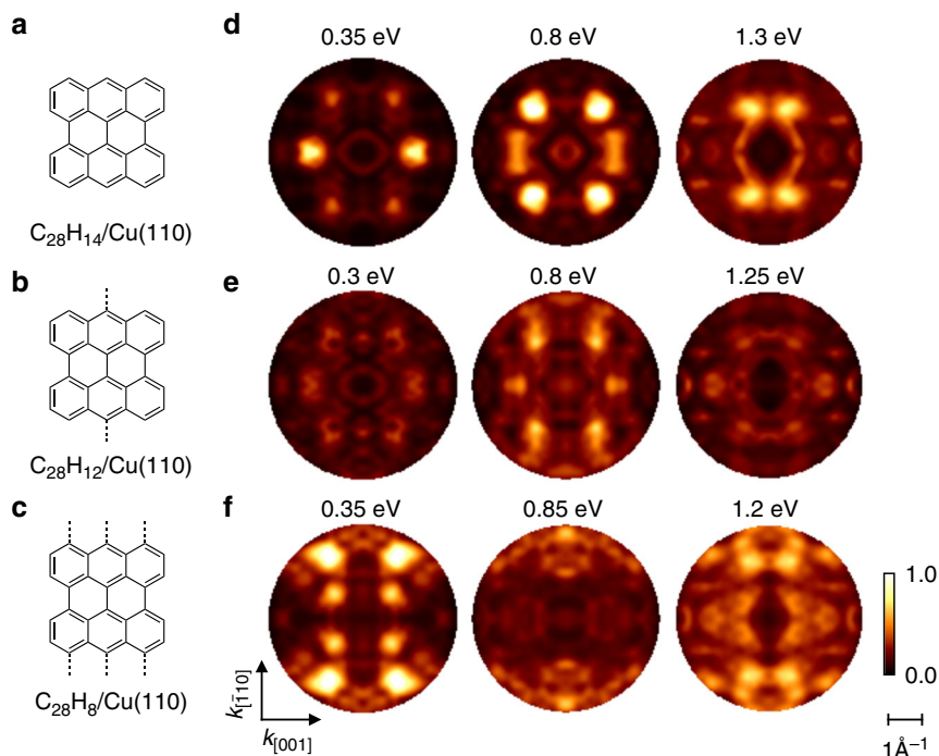
Fig. 4 Bisanthrene, C_{28}H_{12} and C_{28}H_8 on the Cu(110) surface. a–c Chemical structure and d–f simulated k-maps at three representative binding energies (compare dotted lines in Fig. 3c) for a, d bisanthrene C_{28}H_{14} and partly dehydrogenated b, e C_{28}H_{12} and c, f C_{28}H_8 . Grey dashed lines in b, c mark localised chemical bonds of dehydrogenated carbon atom with copper atoms
