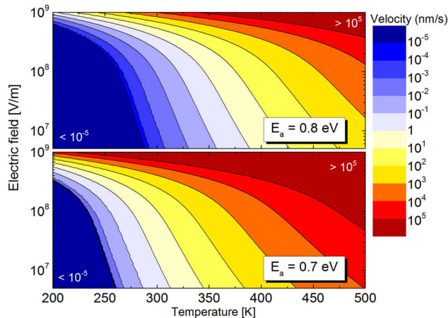
FIG. 7. 2-D contour plots of the drift velocity of oxygen vacancy according to Eq. (5) using activation energies of 0.8 and 0.7 eV for unstrained and tensile strained SrTiO 3 , respectively.
