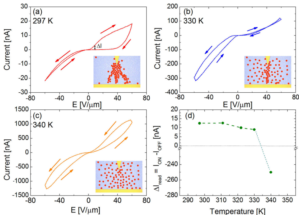
FIG. 8. (a)–(c) IVCs of an e-synapse (14° tip) on 90 nm thick SrTiO 3 film on DyScO 3 measured at different temperatures and (d) difference of the read current measured at 5 V in the ON state and OFF state. The schematics in (a)–(c) display the expected change of the distribution of oxygen vacancies for the different temperatures.
