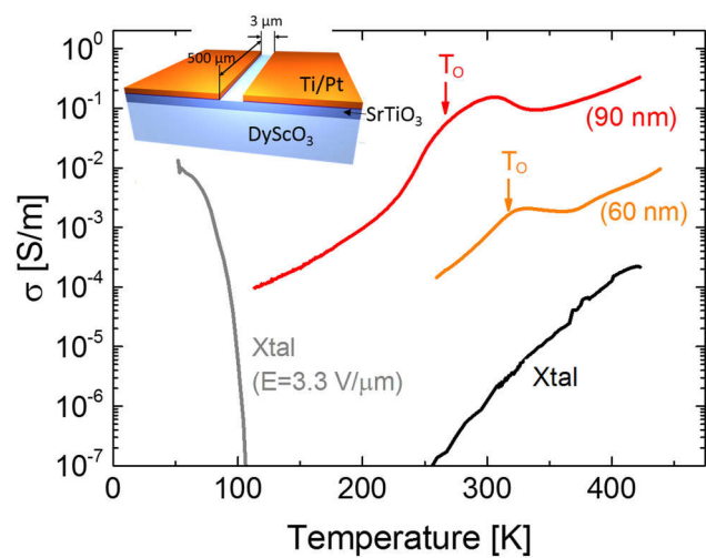
FIG. 3. Temperature dependence of the conductivity of a 90 nm and a 60 nm thick SrTiO 3 film on (110) DyScO 3 measured along the large strain ([010] SrTiO 3 ) direction and, for comparison, of unstrained SrTiO 3 (single crystal). All measurements represent the conductivity at small electric fields, i.e., in the ohmic regime, except for the low temperature data for crystalline SrTiO 3 (gray line) which was measured at elevated field (3.3 V/ \mu m) in order to obtain a measurable signal above the noise floor of \sim 5 \cdot 10^{-8} S/m. The phase transition temperature T_o for strained SrTiO 3 is marked, the inset shows a sketch of the electrode design and the arrangement of the layers.
