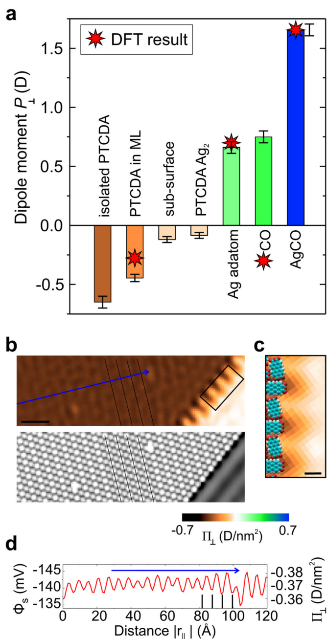
Figure 4. Surface dipoles of selected nanostructures and dipole density within a layer.
