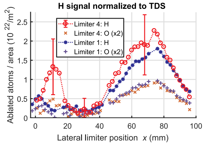
Fig. 7. Comparison of the hydrogen and oxygen content of limiter tiles 3 measured with LIA-QMS in different modules of W7-X.
