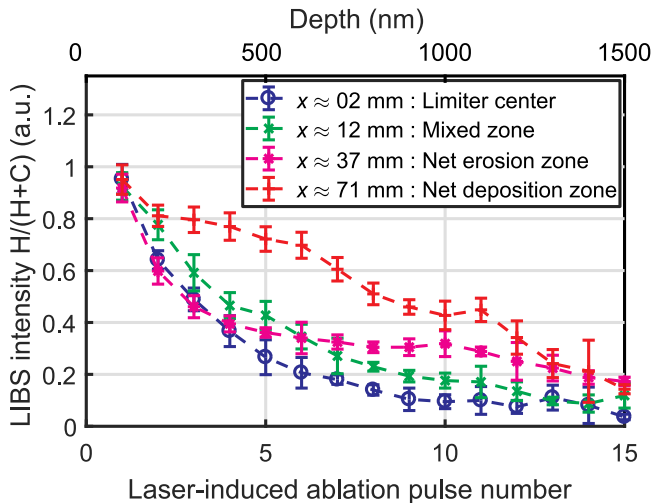
Fig. 6. Depth resolved LIBS signal on limiter 4 - tile 3.
