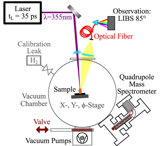
Fig. 2. Schematic overview of the setup: Single picosecond laser pulses are used to successive ablate a sample in a vacuum chamber. A combination of LIBS and QMS is used to measure the sample's composition. For a residual gas analysis and the calibration of the quadrupole mass spectrometer a valve to the vacuum pumps is closed (figure based on [16]).
