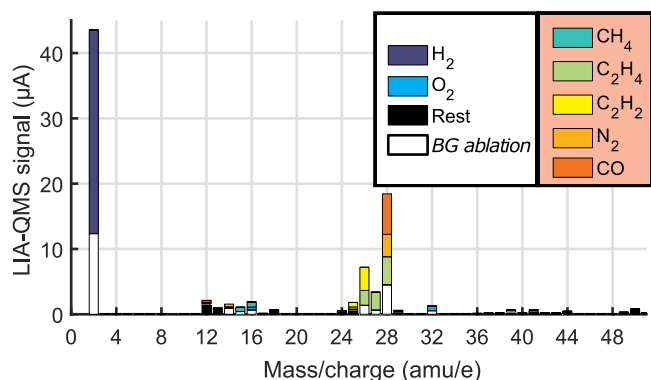
Fig. 8. Possible solution for the composition analysis of the first laser pulse in the deposition dominated zone. Pulse number 15 in white is showing the constant background ( BG ablation ) signal. (For interpretation of the references to colour in this figure legend, the reader is referred to the web version of this article.)
