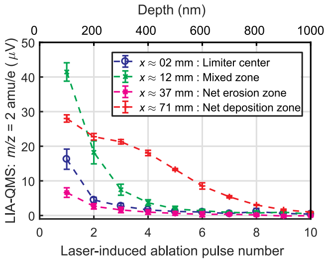
Fig. 5. Depth resolved LIA-QMS hydrogen signal for different toroidal positions x on limiter 4 - tile 3 which show zones of different plasma interaction with the surface.
