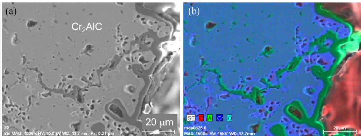
Figure 6 Polished cross-section of porous \text{Cr}_2\text{AlC} (75%) after the creep test in (a) BSEM image and (b) EDX element mapping, which show that the surface pores are closed by the scales and microcracks are healed by the scales.
