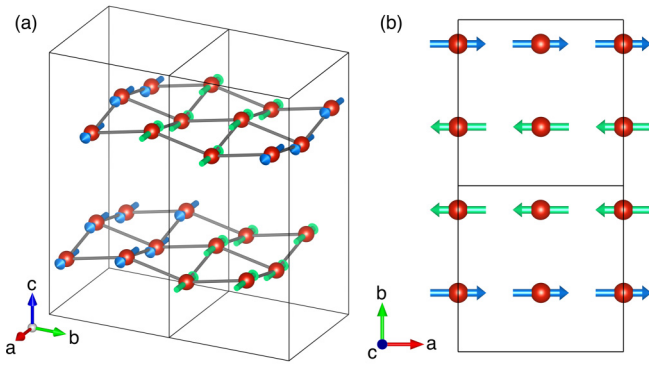
FIG. 3. Magnetic structure of \text{BaCdVO}(\text{PO}_4)_2 as determined by neutron diffraction. The \text{V}^{4+} ions form a distorted square lattice with ordered moments along the a direction. Panel (a) shows a general view and (b) the ab square-lattice plane. The different spin colors differentiate between moment directions. The structural unit cells are shown as solid-line boxes/squares.
