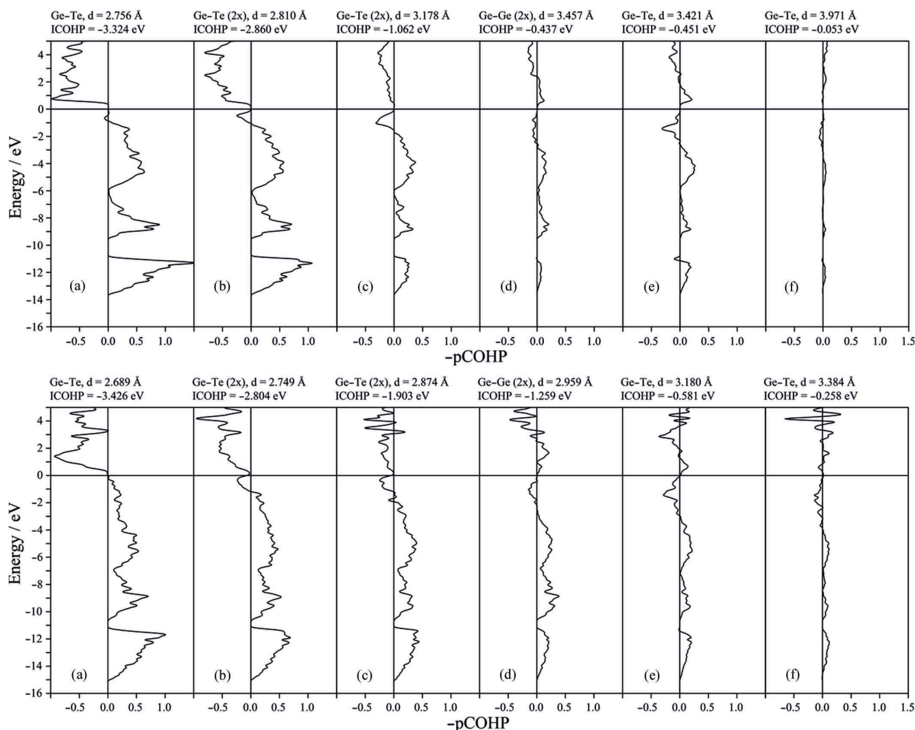
Figure 7 COHP plots of selected bonds within the GeTe-III structure at 0 GPa (top) and 15 GPa (bottom). Positive COHP values indicate bonding interactions whereas negative COHP represent antibonding states.
