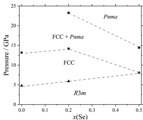
Figure 8 Tentative high-pressure phase diagram of the \text{GeSe}_x\text{Te}_{1-x} solid solution for x(\text{Se}) between 0 and 0.5.
