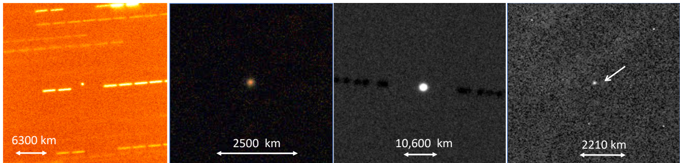
Figure 1. Montage of images of ‘Oumuamua showing its point-like unresolved appearance with no hint of detectable activity. From left to right: 0.4 hr integration through an R-band filter with the Nordic Optical Telescope on 2017 October 26 (Jewitt et al. 2017); “true color” image simulated from grizY -band images obtained on 2017 October 27 for a total integration of 1.6 hr with the Gemini South telescope (Meech et al. 2017); a deep 3.6 hr r -band composite image obtained on 2017 October 27–28 with the Gemini North telescope (Drahus et al. 2018); and an F350LP image from Hubble Space Telescope (Micheli et al. 2018).
