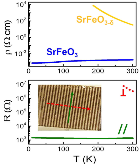
FIG. 5. Electronic resistivity as a function of temperature for monolithic insulating \text{SFO}_{3-\delta} ( \delta \approx 0.5 ) and metallic \text{SFO}_3 (top), and resistance as a function of temperature for a 200- \mu\text{m} periodicity \text{SFO}_3/\text{SFO}_{2.5} heterostructure (bottom) measured perpendicular to the stripe direction (red, dotted) and parallel to the stripe direction (green, solid), with inset visualization of current direction in a film.
