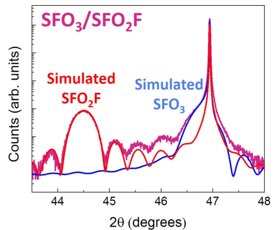
FIG. 4. X-ray diffraction of \text{SFO}_3/\text{SFO}_2\text{F} heterostructure (purple) with superimposed simulated diffraction data of \text{SFO}_3 (blue) and \text{SFO}_2\text{F} (red).
