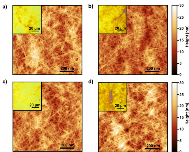
Figure 2. AFM topographic images with four different surface charges: (a) 400, (b) 800, (c) 1000, and (d) 1360 μmol/g. The insets are optical microscopy images of the corresponding films.
