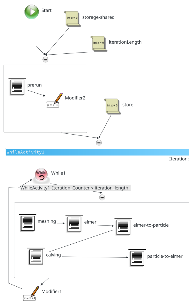
Figure 4. Workflow implementation in the URC workbench.
