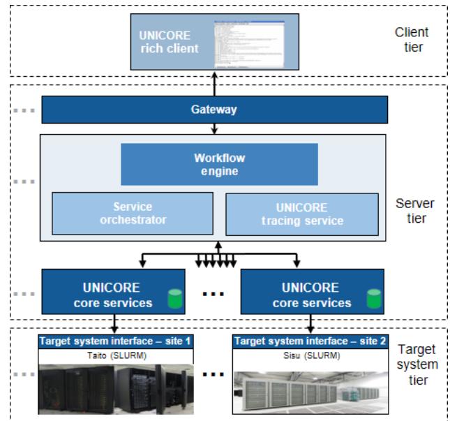
Figure 3. Multi-tiered UNICORE architecture.
