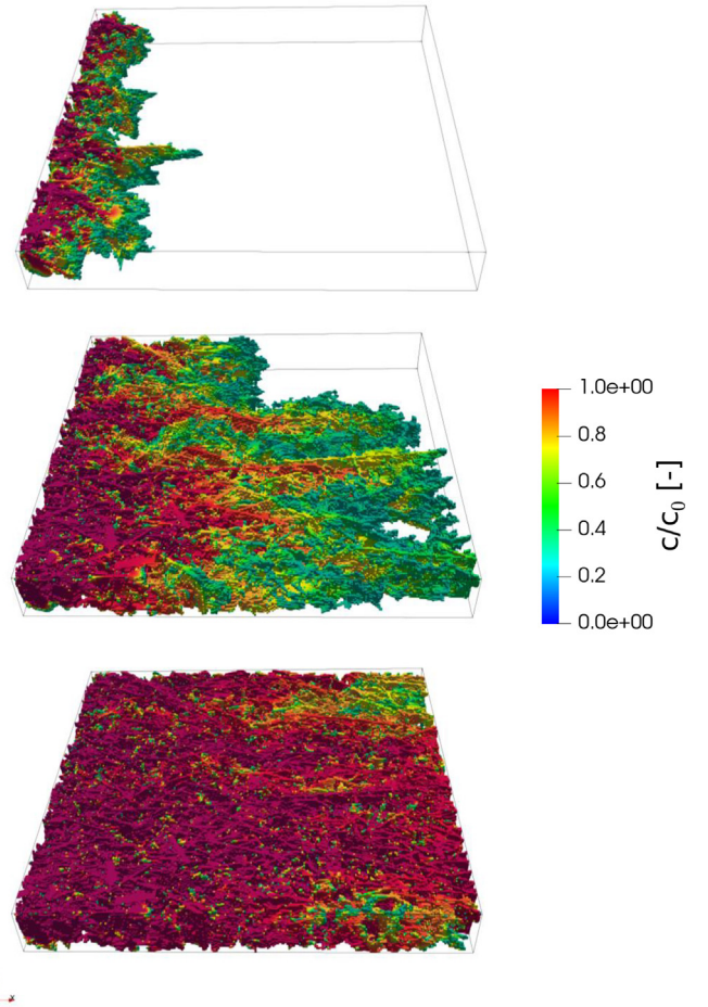
Fig. 9. TC2: concentration of the conservative tracer at time (a) 5 y, (b) 35 y and (c) 100 y. A portion of the domain is hidden in order to show a vertical cross-sections. Concentration values are normalised by the concentration in the boundary water. The cells with concentration c/c_0 < 0.2 are not shown.
