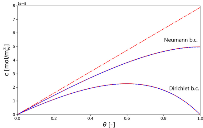
Fig. 3. ^4\text{He} concentration along the flowing fracture computed using the Dirichlet and the Neumann boundary conditions for Pe = 2.5 . The blue dashed lines are the results of the PFLOTTRAN 1D calculations while the red continuous lines are the two analytical solutions (Eqs. (11) and (12)). The dashed dotted line is the analytical solution for an infinite Peclet number (Eq. (16)). Distance is normalised by the total fracture length ( \theta = x/L ).
