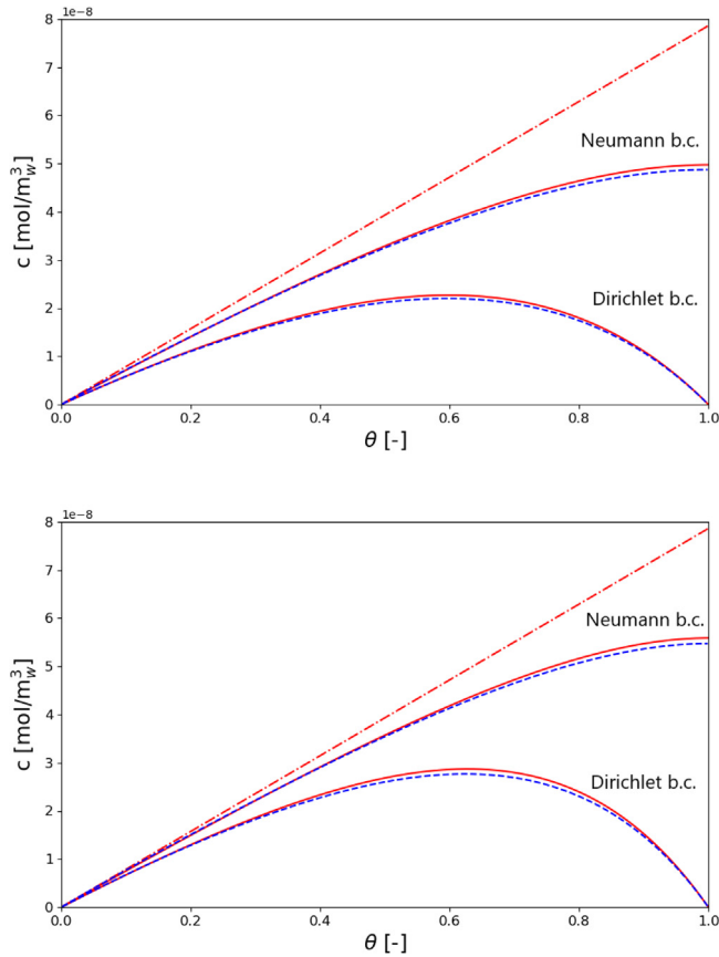
Fig. 2. ^4\text{He} concentration along the flowing fracture computed using the Dirichlet and the Neumann boundary conditions for (top) Pe = 2.5 and (bottom) Pe = 3.3 . The blue dashed lines are the results of the PFLOTTRAN simulations while the red continuous lines are the two analytical solutions (Eqs. (11) and (12)). The dashed dotted line is the analytical solution for an infinite Peclet number (Eq. (16)). Distance is normalised by the total fracture length ( \theta = x/L ).
