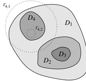
Fig. 1.1 Exemplary scatterer D with bulk D_1 that contains three inner components D_2, D_3, D_4 . For demonstration purposes, some admissible source boundary \Gamma_4 = \Gamma_{4,1} \cup \Gamma_{4,2} for D_4 is added dottedly in the component's outside and inside, respectively.
