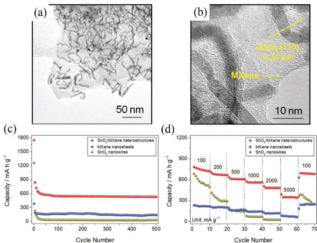
Figure 17. a) High-magnification TEM and b) HRTEM images of a SnO 2 nanowire/Ti 3 C 2 (MXene nanosheet) nanocomposite. c) Cycling performance at 1 Ag -1 and d) rate capability at different current densities of this composite, in comparison with the phase-pure counterparts. Reproduced (adapted) with permission from Ref. [94a]. Copyright 2018, Wiley-VCH.
