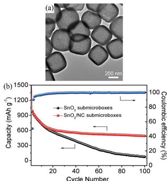
Figure 13. TEM (a) image of \text{SnO}_2/\text{NC} sub-microboxes and their cycling performance at 0.5 \text{ A g}^{-1} compared to \text{SnO}_2 sub-microboxes (b). Reproduced (adapted) with permission from Ref. [18c]. Copyright 2018, Wiley-VCH.
