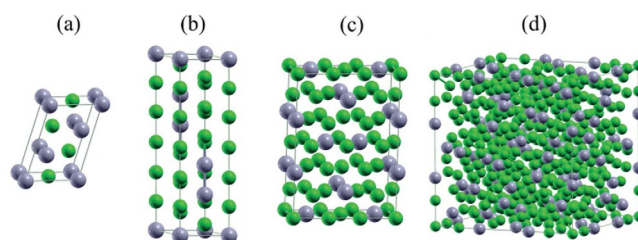
Figure 3. Schematic representation of theoretically predicted intermediate \text{Li}_x\text{Sn} alloys: a) \text{LiSn} , b) \text{Li}_{13}\text{Sn}_5 , c) \text{Li}_7\text{Sn}_2 , and d) \text{Li}_{17}\text{Sn}_4 . Green and gray spheres represent Li and Sn atoms, respectively. Reproduced (adapted) with permission from Ref. [7a]. Copyright 2015, Royal Society of Chemistry.
