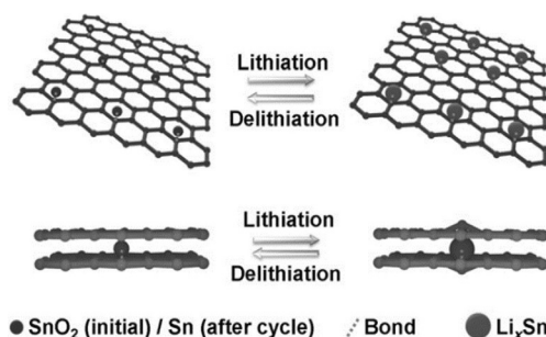
Figure 14. Schematic illustration of lithiation/delithiation processes in a \text{SnO}_2 nanocrystal/graphene composite. Reproduced (adapted) with permission from Ref. [67c]. Copyright 2014, Wiley-VCH.
