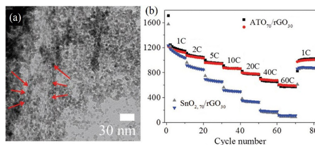
Figure 15. a) HR-TEM image of Sb:SnO 2 nanoparticles on rGO sheets. b) Specific capacity of galvanostatic charge/discharge measurements at C rates up to 60 C. Reproduced with permission from Ref. [44b]. Copyright 2018, Wiley-VCH.
