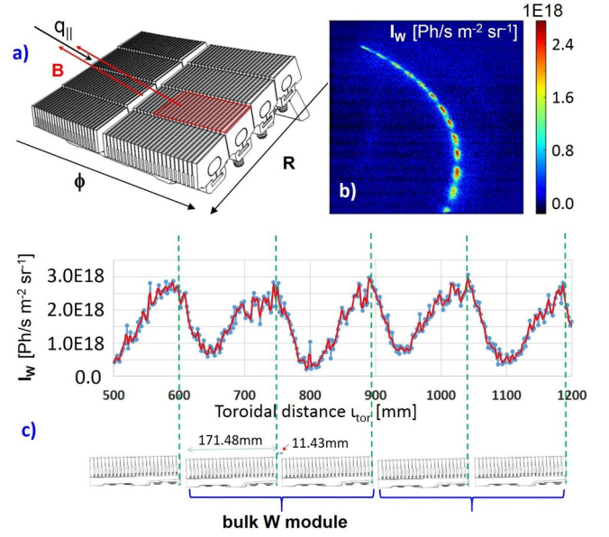
Fig. 5. Full view of a bulk W module (a) with indication of the wetted area, divertor view (b) as seen by the AVT-PIKE camera (KL11) equipped with a WI interference filter; toroidal distribution of the photon flux I_{WI} at the outer strike point measured in discharge JPN 90453 at t = 55.599 s (c).
