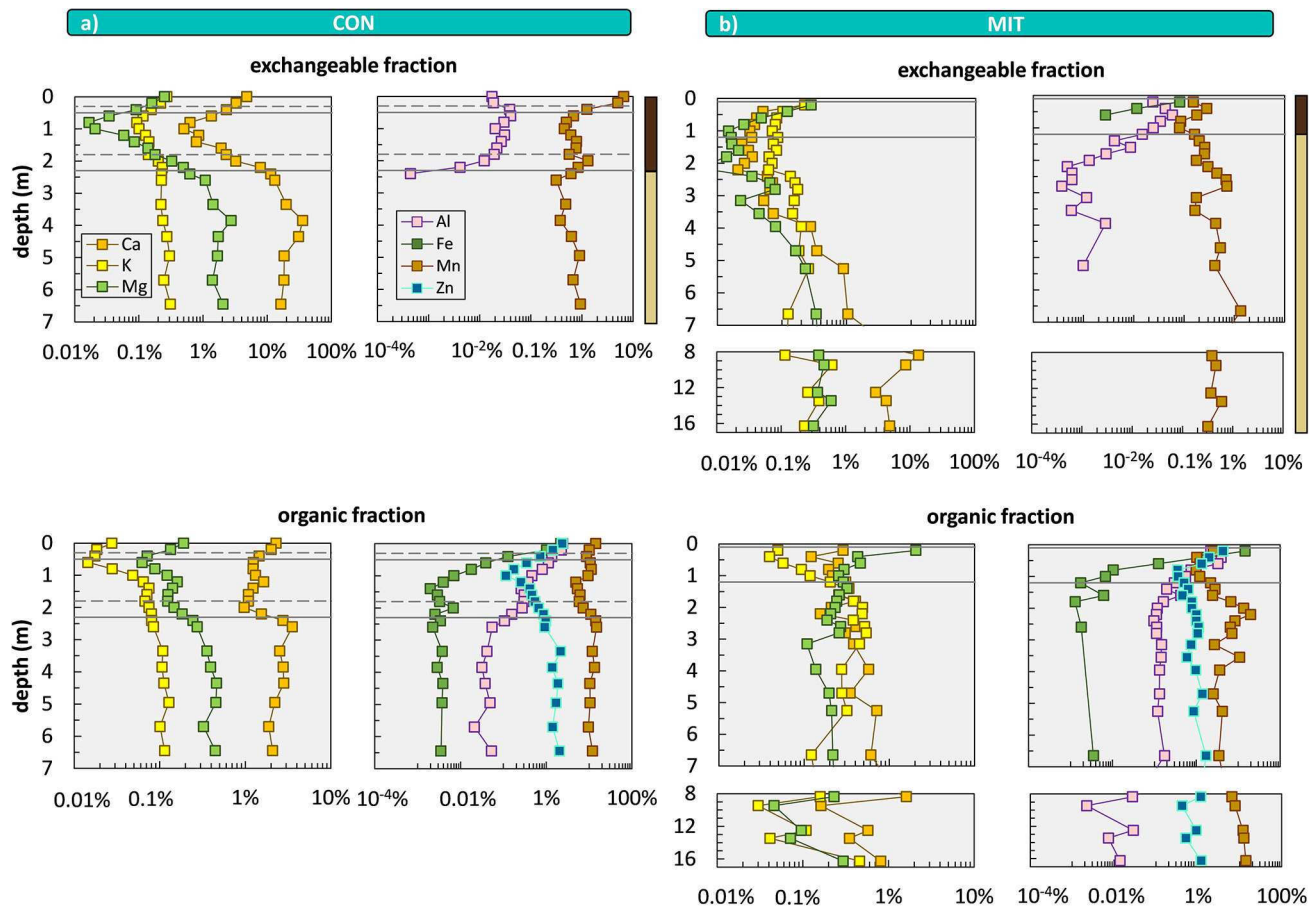
FIGURE 6 | Depth distributions of sequentially extracted fractions comprising the exchangeable fraction (1 M \text{NH}_4\text{OAc} ) and organic fraction (30% \text{H}_2\text{O}_2 in 0.01 M \text{HNO}_3 ) at CON (a) and MIT (b). Shown are total concentrations relative to bulk soil and saprolite samples. Data gaps occur when extractant was below limit of detection. Solid lines illustrate soil horizon boundaries and the interface of weathered rock to unweathered rock. Dashed lines indicate soil horizon subdivision (see Figure 2). Colored bars at the top of the panel refer to color coding of drill core sections from Figure 2. For ease of display we changed the y-axis spacing with depth, yet all data are shown continuously.
