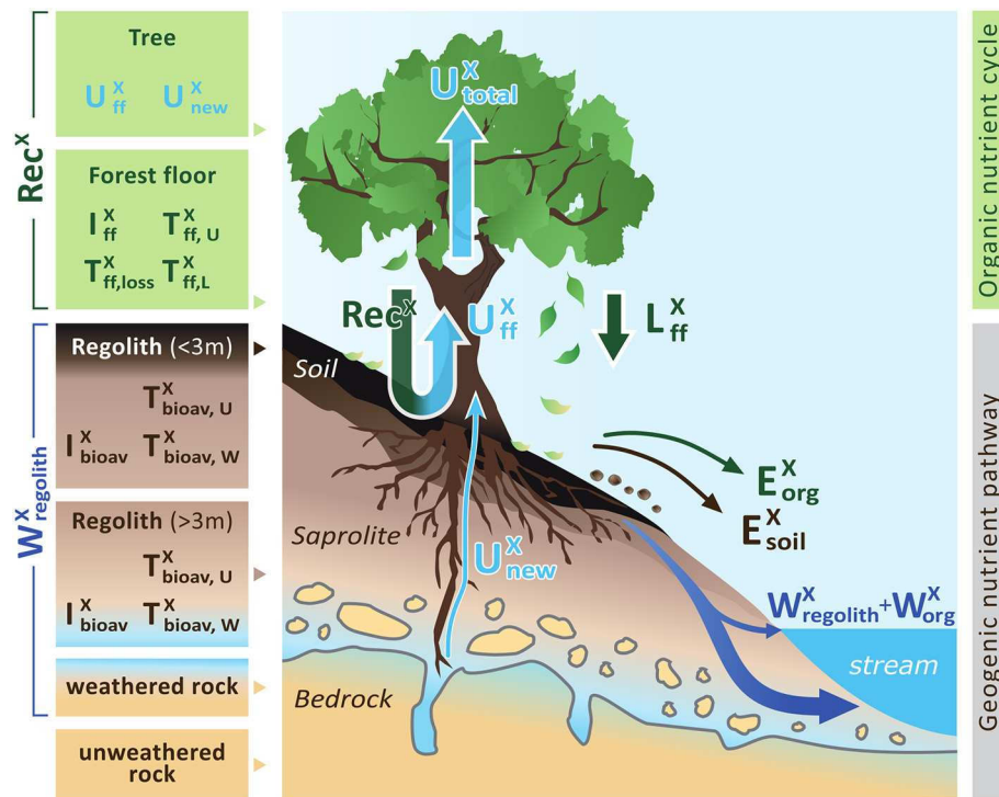
FIGURE 1 | A conceptual forest ecosystem comprising the “geogenic nutrient cycle” which is mainly effected by nutrient release through chemical weathering ( W_{regolith}^X ) and the “organic nutrient pathway” which is mainly effected by nutrient re-utilization (recycling) from organic matter ( Rec^X ). Individual compartments are presented as boxes including the metrics used to quantify their properties: nutrient inventory ( I ) and nutrient turnover time ( T ) of element X . The first subscript refers to the ecosystem compartment (“ff” denotes forest floor, “bioav” denotes the biologically available fraction and “regolith” denotes soil, saprolite and weathered rock, respectively). The second subscript refers to the flux used to calculate the respective turnover time (“U” denotes nutrient uptake, “L” denotes litterfall, “W” denotes chemical weathering). Compartments are linked by fluxes (arrows), where the thickness of the arrows indicates the relative proportions. Fluxes include nutrient uptake ( U ), chemical weathering ( W ), erosion ( E ) of soil or organic matter (org), and litterfall ( L ). “Rec” denotes nutrient recycling. Detailed information on the metrics is provided in Table 1 . Figure is not drawn to scale.
