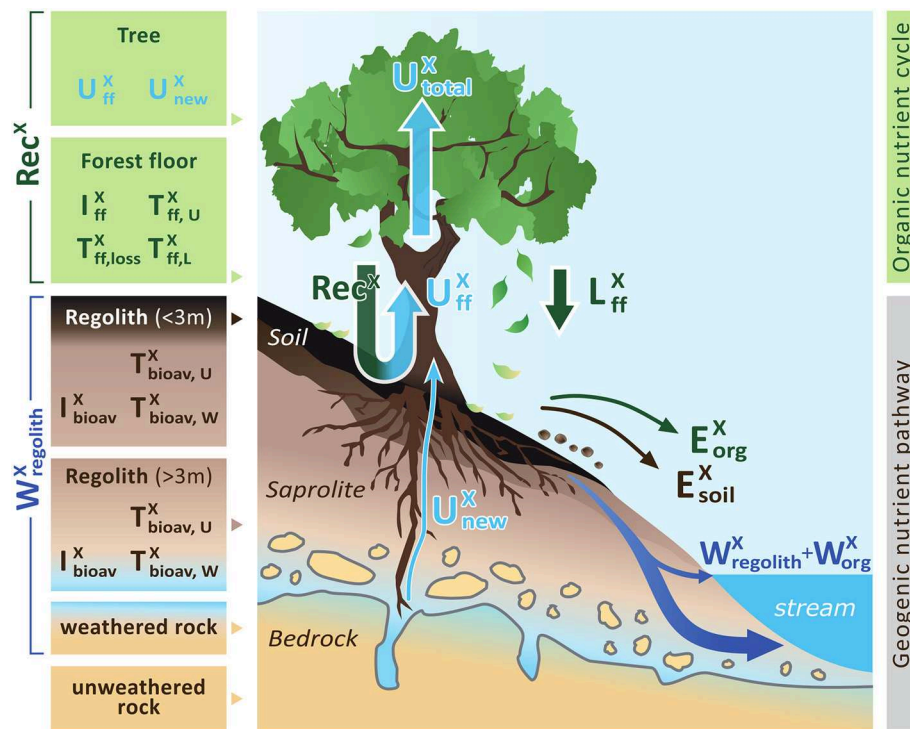
FIGURE 1 | A conceptual forest ecosystem comprising the “geogenic nutrient cycle” which is mainly effected by nutrient release through chemical weathering ( W_{regolith}^X ) and the “organic nutrient pathway” which is mainly effected by nutrient re-utilization (recycling) from organic matter ( Rec^X ). Individual compartments are presented as boxes including the metrics used to quantify their properties: nutrient inventory ( I ) and nutrient turnover time ( T ) of element X . The first subscript refers to the ecosystem compartment (“ff” denotes forest floor, “bioav” denotes the biologically available fraction and “regolith” denotes soil, saprolite and weathered rock, respectively). The second subscript refers to the flux used to calculate the respective turnover time (“U” denotes nutrient uptake, “L” denotes litterfall, “W” denotes chemical weathering). Compartments are linked by fluxes (arrows), where the thickness of the arrows indicates the relative proportions. Fluxes include nutrient uptake ( U ), chemical weathering ( W ), erosion ( E ) of soil or organic matter (org), and litterfall ( L ). “Rec” denotes nutrient recycling. Detailed information on the metrics is provided in Table 1 . Figure is not drawn to scale.
