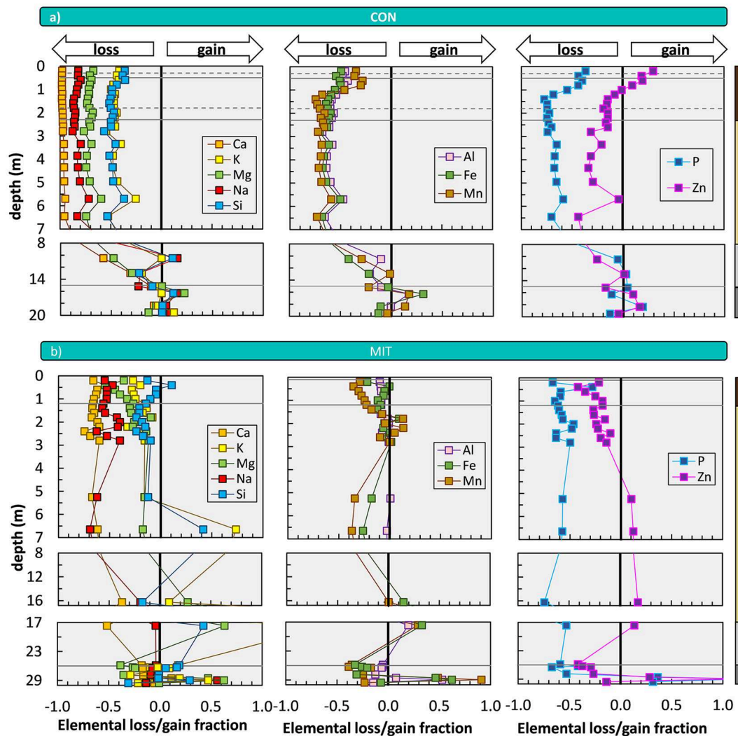
FIGURE 4 | Depth distribution of elemental loss/gain fractions (mass transfer coefficients, \tau_{Xj}^X ) at CON (a) and MIT (b). The vertical line indicates a \tau_{Xj}^X -value of zero and represents unweathered parent bedrock. Solid horizontal lines illustrate soil horizon boundaries and the interface of weathered rock to unweathered rock. Dashed horizontal lines indicate soil horizon subdivision (see Figure 2). Colored bars at the right site of panel a refer to color coding of drill core sections from Figure 2. For ease of display we changed the y-axis spacing with depth, yet all data are shown continuously. X-axis scale in panel a (not shown) is the same as in panel b. Given that some outliers were excluded from this figure, Figure 3a and from flux estimates that are based on \tau_{Xj}^X , we show the depth distribution of element concentrations in Supplementary Figure 2, and \tau_{Xj}^X in Supplementary Figure 3 and Supplementary Figure 4 [according to Fisher et al. (2017) \log_{10}(C_X/C_i) ] including the outliers.
