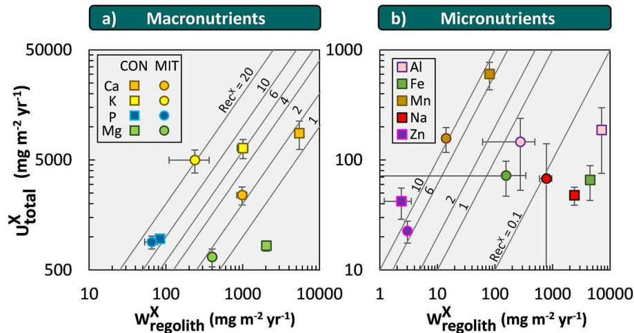
FIGURE 5 | Chemical weathering fluxes ( W_{regolith}^X ) and ecosystem nutrient uptake fluxes ( U_{total}^X ) for macronutrients (a) and micronutrients + Na (b) at CON (squares) and MIT (circles). Contour lines illustrate the nutrient recycling factor ( Rec^X ), which is the ratio of U_{total}^X to W_{regolith}^X . Uncertainty bars show one standard deviation (see section Calculation of Fluxes and Inventories in Forest Ecosystems).
