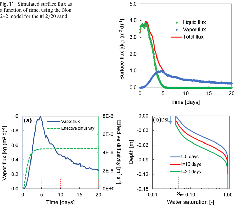
Fig. 12 a Simulated surface vapor flux and effective diffusivity by the Non 2–2 model as a function of time. Three time points (5, 10 and 20 days) are marked by the dotted red line and are the simulated times in Fig. 12b; b simulated water saturation profile at different times by the Non 2–2 model, the vertical black dotted line is where the residual water content ( S_{rw} ) located. The blue arrow indicates the increase in the dry surface layer thickness over time. All the results are of #12/20 sand
