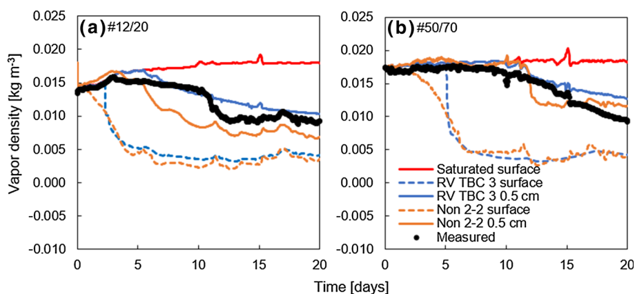
Fig. 16 Measured and simulated vapor density at the soil surface and 0.5 cm below the soil surface for the Richards vapor (RV) and Non 2–2 models. In the legend, “Saturated surface” means the calculated saturated vapor density at the surface based on measured the surface temperature (Eq. 11), “surface” means the vapor density is at the surface and “0.5 cm” means vapor density is at the 0.5 cm depth
