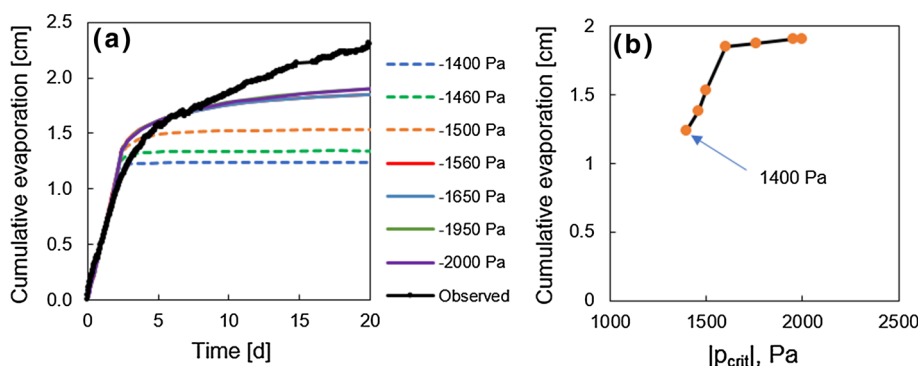
Fig. 5 a Observed and simulated cumulative evaporation as a function of time for different critical water pressures; b cumulative evaporation at t = 20 days based on the critical water pressures shown in Fig. 5a. All figures are shown for the Richards model based on the soil properties of Exp 1 (#12/20 sand)
