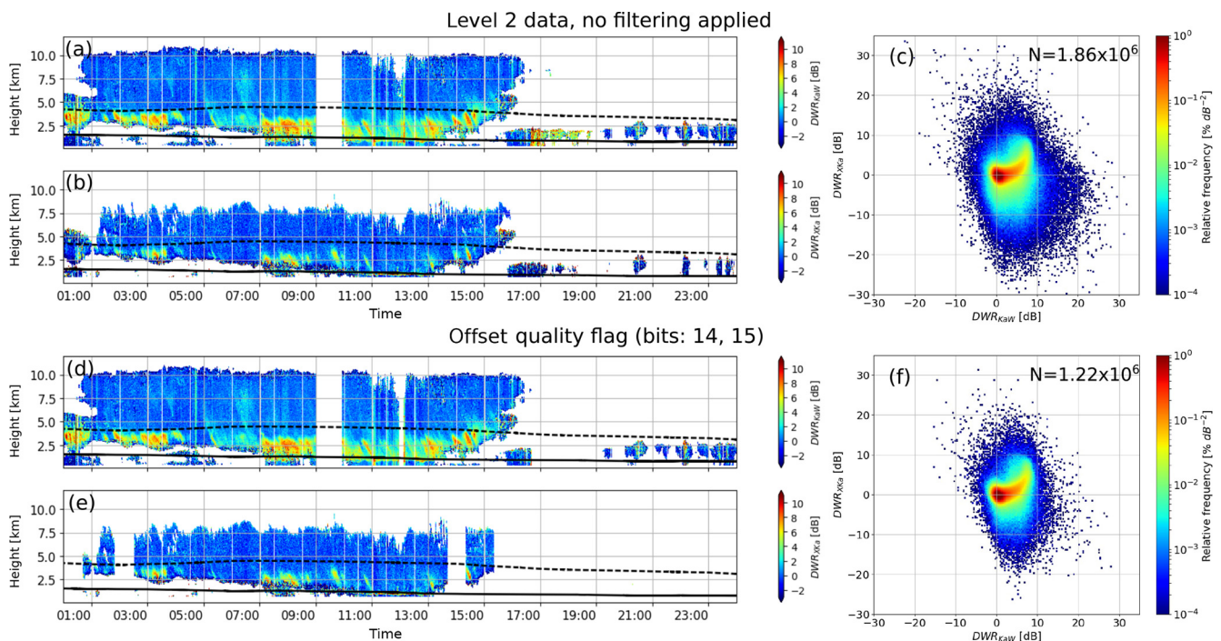
Figure 4. Time–height plots of DWR KaW (a) and DWR XKa (b) using the Level 2 data of 20 November 2015 without applying any filtering. The continuous line and dashed line are the 0 and -15^{\circ}\text{C} isotherms (provided by the CloudNet products), respectively. The triple-frequency signatures for the ice part of the clouds are shown in (c). Panels (d–f) show the remaining data after applying the offset quality flags and the restriction to data pairs with sufficient correlation. N in (c, f) indicates the respective number of data pairs in the ice part of the clouds. Note the log scale on the color bars in (c, f).
