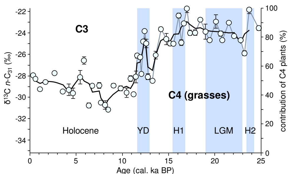
Figure 5: Reconstruction of changing proportions of C3 and C4 vegetation based on \delta^{13}\text{C}
