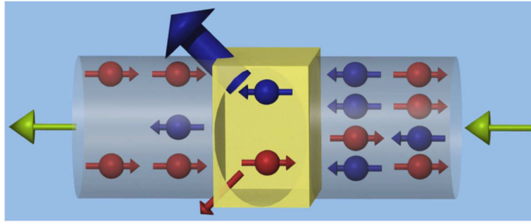
Fig. 1 Spin-filtering concept. The spin-dependence of the hadronic interaction cause a selective discard of one spin state of the stored particles
