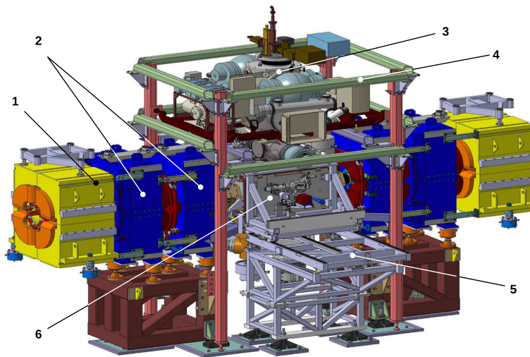
Fig. 6 View of the PAX installation at COSY from the interior of the ring (the beam comes from the left). 1: COSY quadrupole magnet; 2: two of the four PAX quadrupoles forming the low- \beta insertion by doublet focusing (DF-FD); 3: atomic beam source (ABS); 4: support system; 5: flange supporting rail system; 6: PAX target chamber housing the detector and the storage cell. The Breit-Rabi polarimeter (BRP) and the target-gas analyzer (TGA) are mounted towards the outside of the ring. (Figure taken from Ref. [12].)
