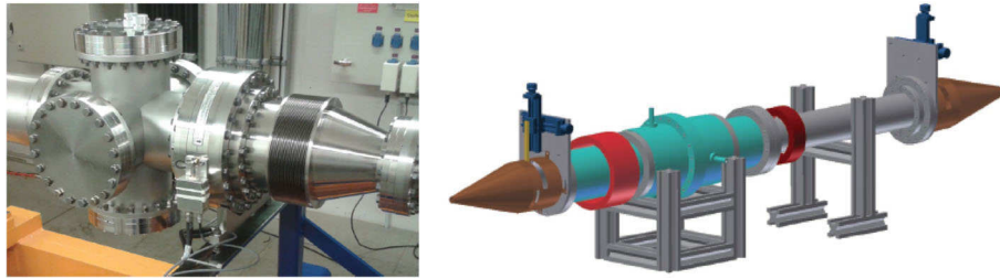
Fig. 9 Left: Fast Current Transformer from Bergoz Instrumentation installed at COSY. The FCT in the ring is equipped with a custom build preamplifier and a current source for calibration. Right: The test station for the beam current measurement devices. Different beam current sensors can be implemented into the test stand. The wire inside the tube is moved using XY tables (blue) mounted on both sides of the system. The wire tension system is covered inside the tapers (copper colored)
