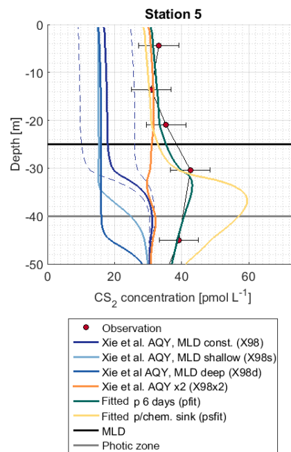
Figure 7. Observation and model sensitivity simulations at station 5. AQY: apparent quantum yield, MLD: mixed layer depth. Simulation names in brackets refer to Table 1. Dashed lines indicate the confidence interval of AQY as reported in Xie et al. (1998).
