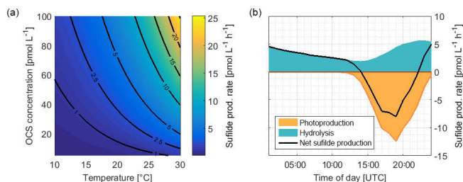
Figure 8. (a) Rate of sulfide production due to OCS hydrolysis as a function of temperature and OCS concentration, calculated with Eqs. (3) and (4). (b) Average consumption of S (organic or inorganic sulfide) by OCS photoproduction and the production of sulfide during hydrolysis from ASTRA-OMZ (average for 7–14 October).
