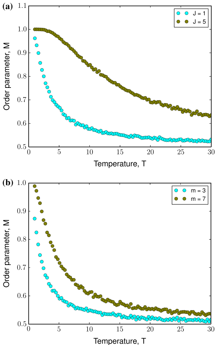
Fig. 7 Monte Carlo simulations of modified Ising model of a Barabási–Albert network of size, N = 5 \times 10^3 at h = 0 and positive coupling constant, J for n = 20 realizations of the Barabási–Albert network. (a) for coupling constants, J = 1 and J = 5 with m = 3 . (b) for different choice of preferentially attached links, m = 3 and m = 7 with J = 1 . Simulation parameters: network size, N = 5 \times 10^3 , preferentially-attached links to construct Barabási–Albert network m = 5 , magnitude of coupling constant, |J| = 1
