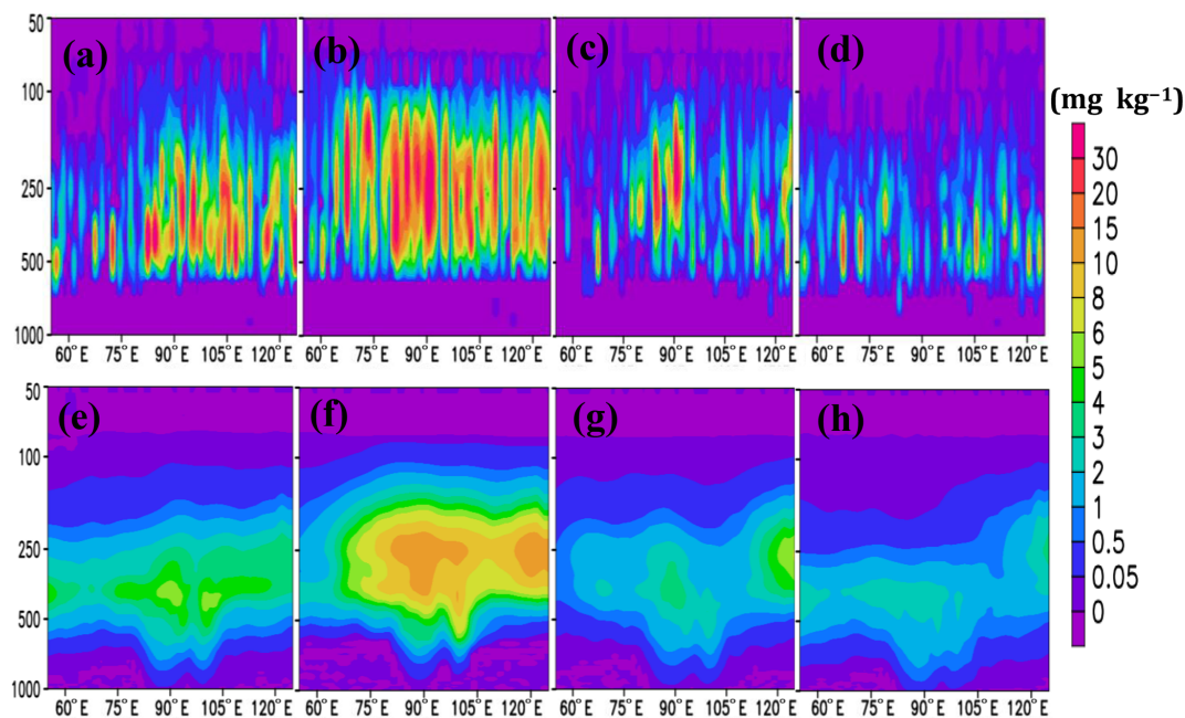
Figure 1. Seasonal mean distribution (2007–2010) of cloud ice mass mixing ratio ( \text{mg kg}^{-1} ) from CloudSat and CALIPSO combined 2C-ICE L3 averaged for 20\text{--}40^\circ\text{N} for the (a) pre-monsoon, (b) summer-monsoon, (c) post-monsoon and (d) winter seasons; (e)–(h) same as (a)–(d) but from CTRL simulations.
