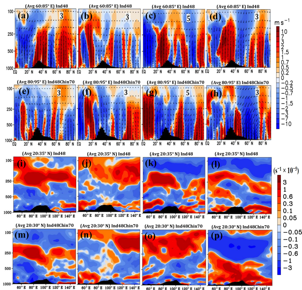
Figure 9. The distribution of anomalies in vertical velocity ( \text{m s}^{-1} ) from Ind48-CTRL for the (a) pre-monsoon, (b) summer-monsoon, (c) post-monsoon and (d) winter seasons; (e)–(h) same as (a)–(d) but for Ind48Chin70-CTRL simulations. Vertical velocity is scaled by 1000. Seasonal distribution of anomalies in the Brunt–Väisälä frequency ( \text{s}^{-1} \times 10^{-5} ) from Ind48-CTRL for the (i) pre-monsoon, (j) summer-monsoon, (k) post-monsoon and (l) winter seasons; (m)–(p) same as (i)–(l) but from Ind48Chin70-CTRL simulations. For the vertical cross section, averages obtained over latitudes or longitudes are indicated in each panel. The black vertical bars indicate topography.
