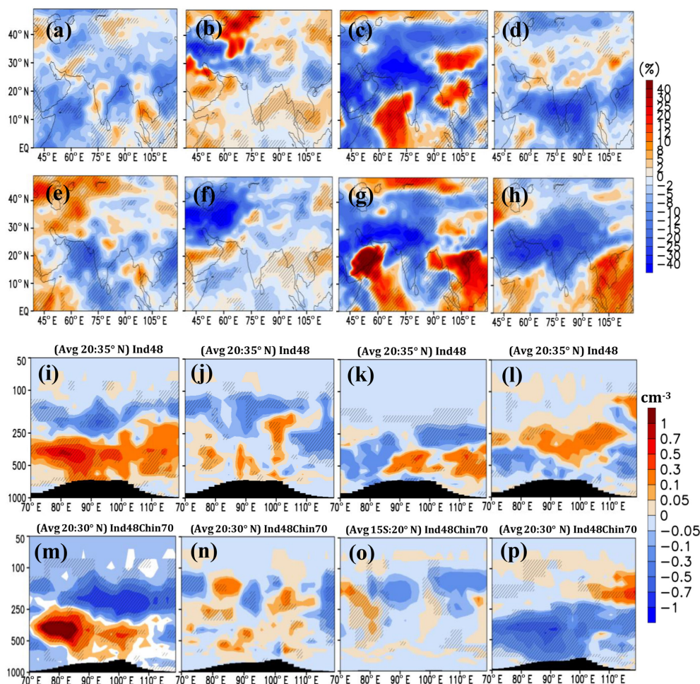
Figure 10. Seasonal distribution of anomalies in cirrus cloud (%) from Ind48-CRTL simulations for the (a) pre-monsoon, (b) summer-monsoon, (c) post-monsoon and (d) winter seasons; (e)–(h) same as (a)–(d) but for Ind48Chin70-CRTL simulations. Seasonal distribution of anomalies in ice crystal number concentration (ICNC; \text{cm}^{-3} ) from Ind48-CRTL for the (i) pre-monsoon, (j) summer-monsoon, (k) post-monsoon and (l) winter seasons; (m)–(p) same as (i)–(l) but from Ind48Chin70-CRTL simulations. For the vertical cross section, averages obtained over latitudes or longitudes are indicated in each panel. The black hatched lines indicate the 99 % significance level. The black vertical bars indicate topography.
