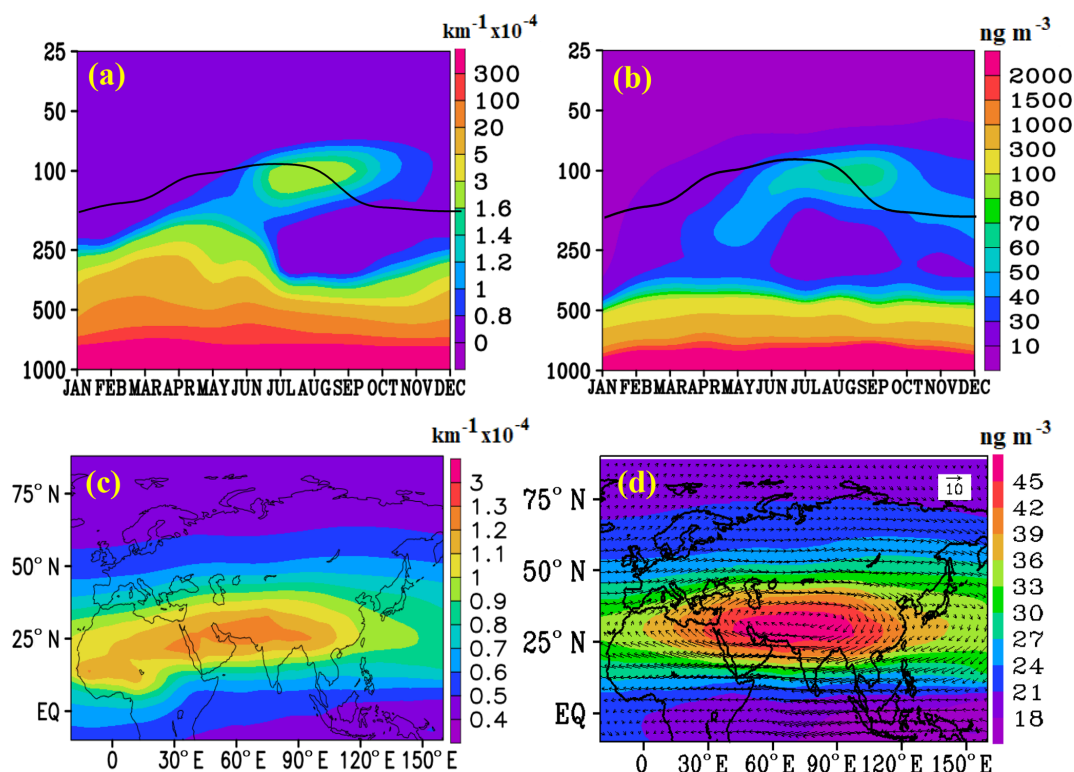
Figure 3. Monthly vertical variation in (a) extinction ( \text{km}^{-1} \times 10^{-4} ) averaged for 25–40° N, 70–120° E; (b) same as (a) but for sulfate aerosols ( \text{ng m}^{-3} ); (c) distribution aerosol extinction ( \text{km}^{-1} \times 10^{-4} ) at 100 hPa averaged for the summer-monsoon season; (d) distribution of sulfate aerosol ( \text{ng m}^{-3} ) at 100 hPa averaged for the summer-monsoon season. Wind vectors in (d) indicate the extent of the anticyclone. Panels (a)–(d) are obtained from CTRL simulations. The black line in (a) and (b) indicates the tropopause.
