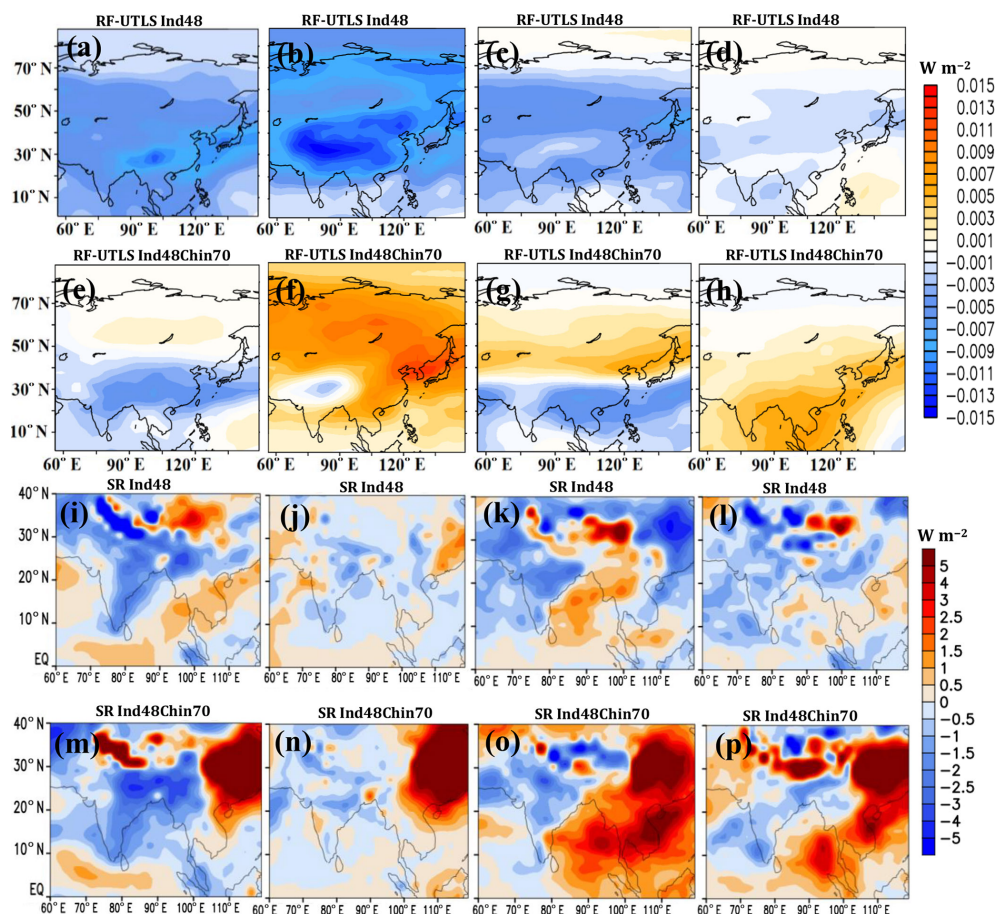
Figure 7. Simulated clear-sky direct net radiative forcing at TOA ( \text{W m}^{-2} ) using the offline model due to sulfate aerosols on the UTLS-only for the (a) pre-monsoon (b) summer-monsoon, (c) post-monsoon and (d) winter seasons for Ind48; (e)–(h) same as (a)–(d) but for Ind48Chin70 simulations. The distribution of anomalies in net solar radiation (SR) ( \text{W m}^{-2} ) at the surface from Ind48 for the (i) pre-monsoon (j) summer-monsoon, (k) post-monsoon and (l) winter seasons; (m)–(p) same as (i)–(l) but for Ind48Chin70 simulations.
