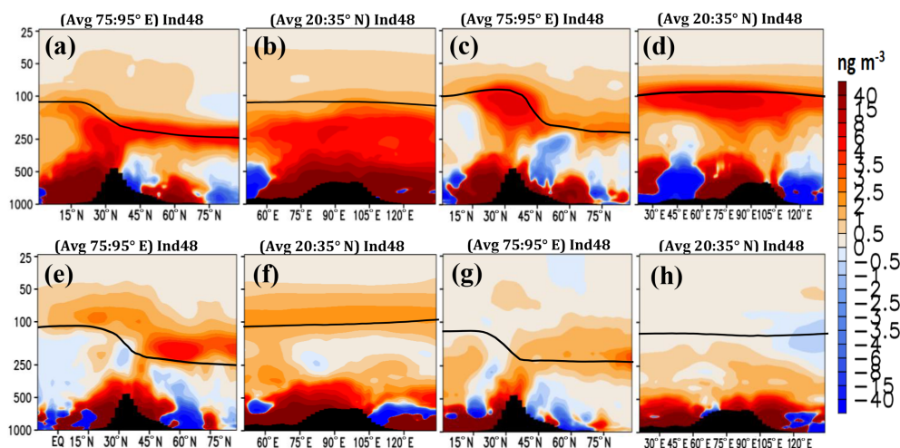
Figure 4. Vertical cross section of anomalies in sulfate aerosols ( \text{ng m}^{-3} ) from Ind48-CTRL simulations for the pre-monsoon season (a) latitude–pressure section and (b) longitude–pressure section; (c)–(d) same as (a)–(b) but for the summer-monsoon season; (e)–(f) same as (a)–(b) but for the post-monsoon season; (g)–(h) same as (a)–(b) but for the winter season. The averages obtained over latitudes or longitudes are indicated in each panel. The black vertical bars indicate topography, and a black line indicates the tropopause.
