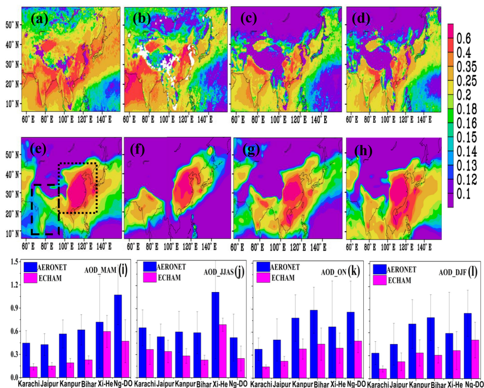
Figure 2. Seasonal mean aerosol optical depth (AOD) from MISR (2000–2016) for the (a) pre-monsoon, (b) summer-monsoon, (c) post-monsoon and (d) winter seasons; (e)–(h) same as (a)–(d) but from CTRL simulations; (i)–(l) same as (a)–(d) but from AERONET (2006–2016) at the following stations: Karachi, Jaipur, Kanpur, Bihar, Xianghe, Nghia Do. The dashed box in (e) indicates the south Asian region ( 8\text{--}35^\circ\text{N} , 70\text{--}95^\circ\text{E} ), where \text{SO}_2 emissions are enhanced by 48 %, and the dotted box indicates Chinese region, where \text{SO}_2 emissions are reduced by 70 % ( 20\text{--}45^\circ\text{N} , 95\text{--}130^\circ\text{E} ).
