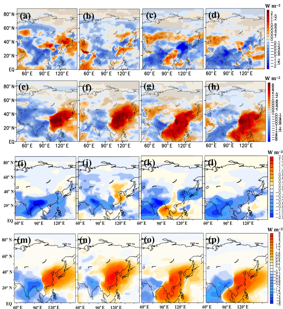
Figure 6. Seasonal distribution of anomalies in clear-sky direct net radiative forcing ( \text{W m}^{-2} ) simulated by ECHAM6-HAMMOZ at the top of the atmosphere, from Ind48-CRTL simulations for the (a) pre-monsoon (b) summer-monsoon, (c) post-monsoon and (d) winter seasons; (e)–(h) same as (a)–(d) but from Ind48Chin70-CTRL simulations; (i)–(l) same as (a)–(d) but from the offline model; (m)–(p) same as (e)–(h) but from the offline model. The black hatched lines in (a)–(h) indicate the 99 % significance level.
