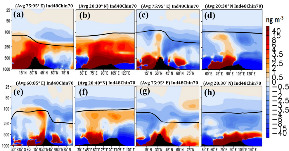
Figure 5. Vertical cross section of anomalies in sulfate aerosols ( \text{ng m}^{-3} ) from the Ind48Chin70-CTRL simulation for the pre-monsoon season (a) latitude–pressure section and (b) longitude–pressure section; (c)–(d) same as (a)–(b) but for the summer-monsoon season; (e)–(f) same as (a)–(b) but for the post-monsoon season; (g)–(h) same as (a)–(b) but for the winter season. The averages obtained over latitudes or longitudes are indicated in each panel. The black vertical bars indicate topography, and a black line indicates the tropopause.
