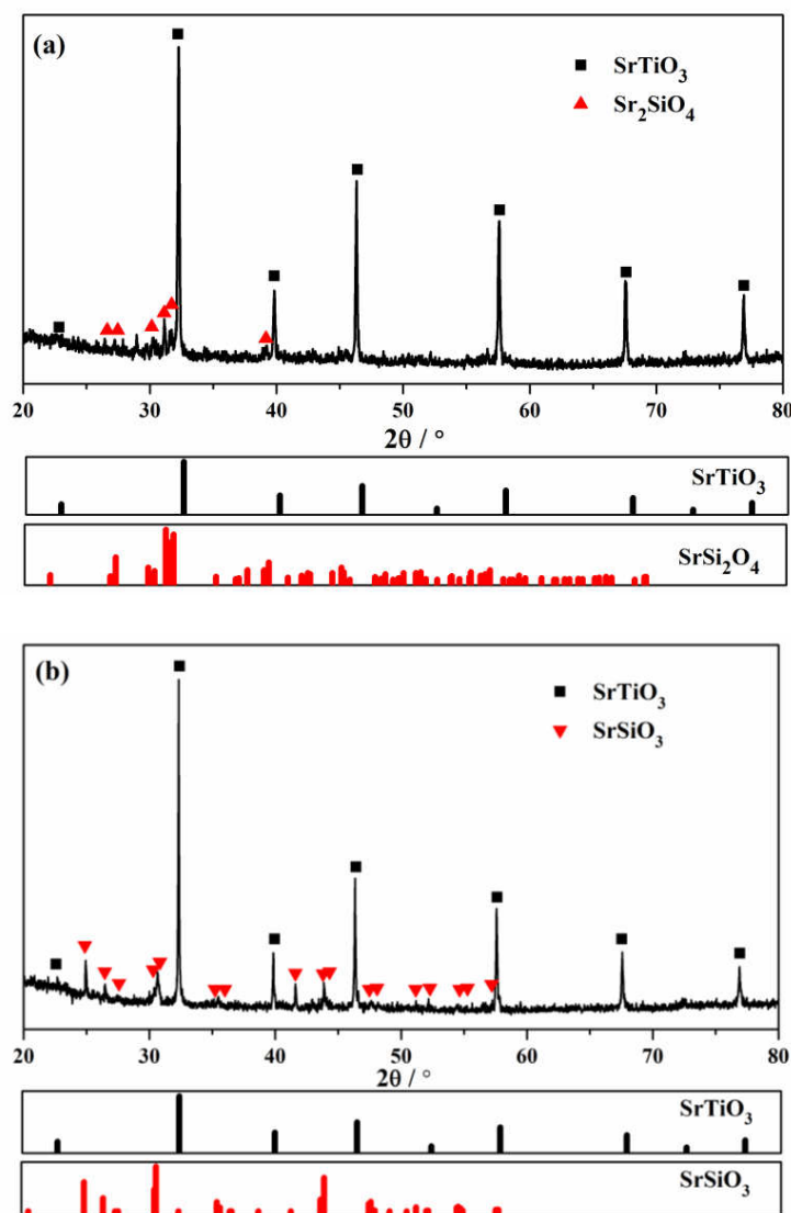
Figure S10 XRD patterns on the steam side (a) and the methane side (b) of spent SMZ-Ti membrane after coupling of water splitting and methane reforming. (Related to Figure 1a and Figure 4)
