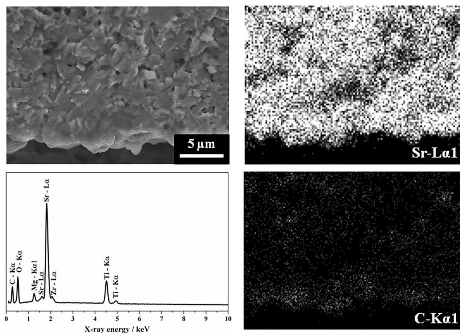
Figure S8. SEM image of the methane-carbon dioxide side of the SMZ-Ti membrane after long-term test for about 200 h, and the corresponding EDX elemental distributions of strontium and carbon. (Related to Figure 4)
