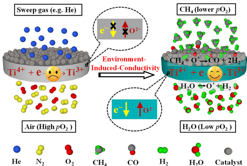
Scheme 1. The Exploitation of SMZ-Ti Mixed Conductivity Induced by Low p\text{O}_2 Environment and the Coupling of Water Splitting with Partial Oxidation of Methane Using an SMZ-Ti Membrane
