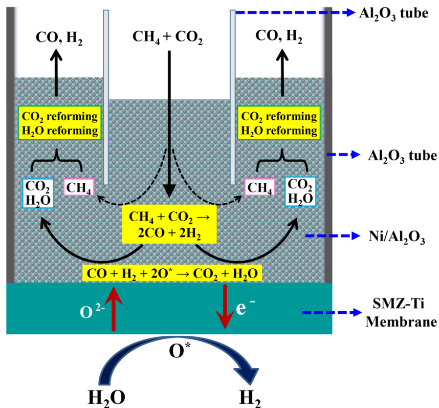
Figure S3. Scheme of catalytic reforming reactions taking place at the permeate side of SMZ-Ti membrane under Cond. IV. (Related to Figure 2)
