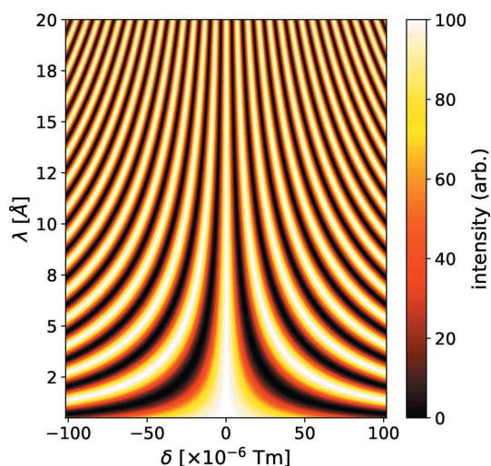
Figure 4 Computed echo oscillations (intensity coded) as function of wavelength ( \lambda in Å) and coding asymmetry \delta in T m. At the true symmetry point \delta = 0 the intensity modulation phase does not depend on \lambda .
