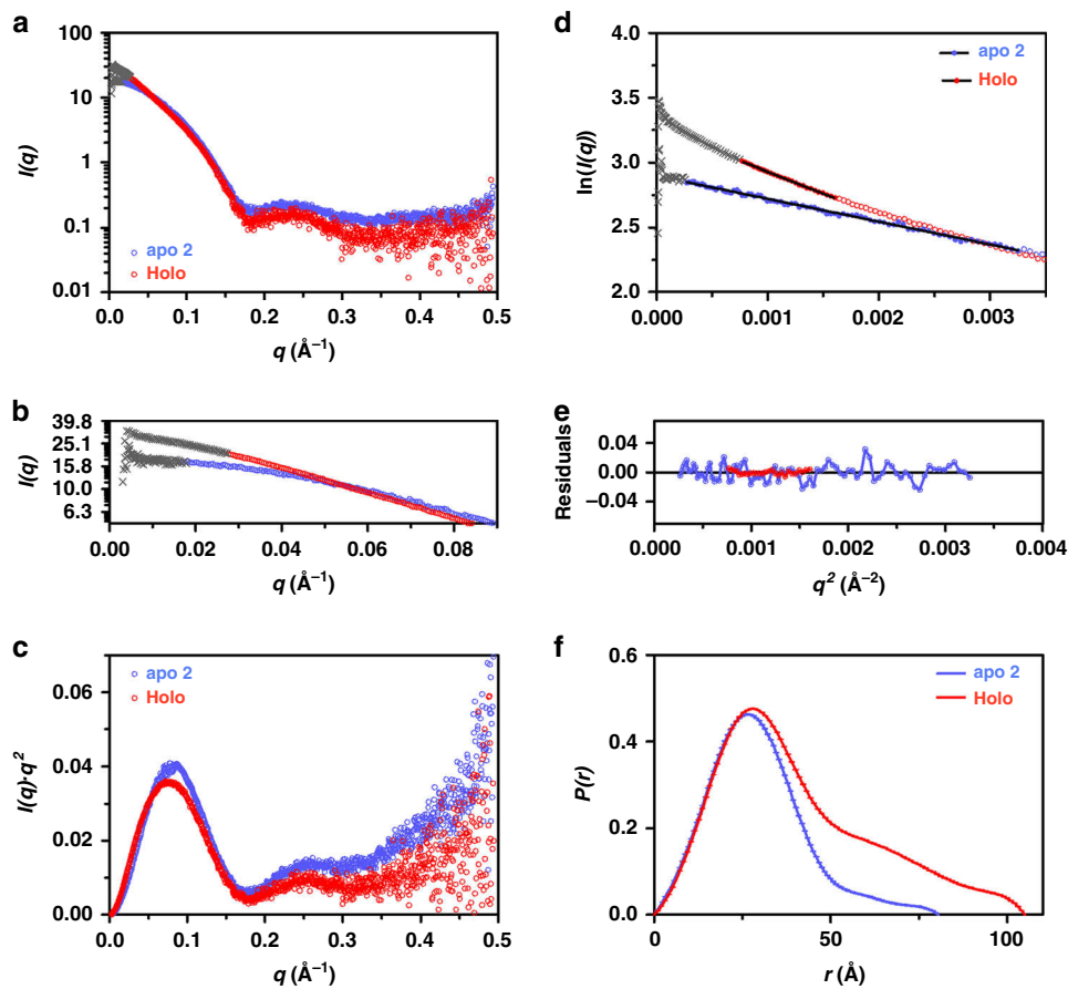
Fig. 2 Apo and holoprotein TeLPOR SAXS data. Representative SAXS data of the TeLPOR apo- (apo 2 dataset; light blue, open circles) and holoprotein (5 mg ml -1 dataset; red, open circles)(for details see: see Supplementary Discussion Section 1.3). The full datasets of the employed concentration series are shown in Supplementary Figs. 4 and 5. a SAXS scattering curve. b Scattering curve in the low q range. c Kratky plots ( I(q) \cdot q^2 versus q ). d Guinier plots ( \ln(I(q)) versus q^2 ) and e residuals for qR_g < 1.3 . Open symbols indicate data beyond the Guinier region. f Pair distribution function, P(r) . Data excluded from Guinier analysis in the low q range is shown as grey crosses in all plots
