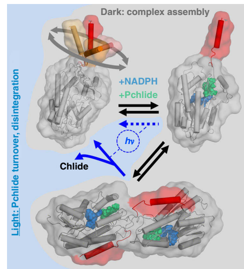
Fig. 6 Model illustrating the proposed structural changes occurring in TeLPOR due to holoprotein formation and light-dependent Pchlde turnover. For a detailed description of the model refer to the main text. Without Pchlde and NADPH, TeLPOR is monomeric, with the C-terminal \alpha -helical extension moving freely (illustrated by four different helical conformations extracted from the corresponding MD trajectory; orange to red cartoon). Assembly of the holoprotein complex in the dark might result in rigidification of the protein, which in turn allows for dimerization, mediated by the C-terminal extension, the Q-axis interface and the active site surface patch. Light-dependent conversion of Pchlde to Chlide, followed by product release would then trigger the dissociation of the dimer. The dashed blue arrow indicates the possibility that also the monomeric holoprotein shows light-dependent activity, as inferred by MWA-AUC. Pchlde and NADPH are shown as green and blue spheres, respectively. The molecular surface of the models are shown as transparent grey surface
