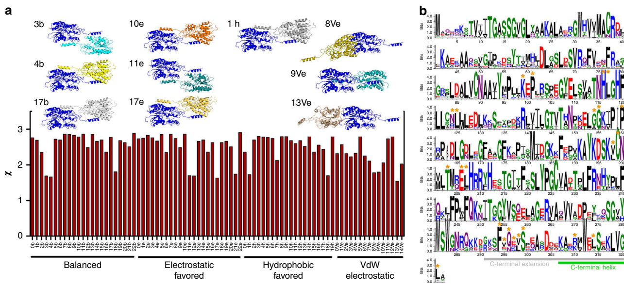
Fig. 4 SAXS-guided modelling of the TeLPOR holoprotein dimer and LPOR residue conservation. a Evaluation of the ClusPro-derived TeLPOR-C helix -based dimer models with regard to \chi for the fit against the experimental scattering data of the holoprotein using the program OLIGOMER 55 . The ten best ClusPro-derived dimer models are shown above the plot (Supplementary Table 3). b Weblogo 374 generated sequence logo, illustrating the conservation of residues within the LPOR family. Residues, which contribute to dimerization are marked by an orange asterisk
