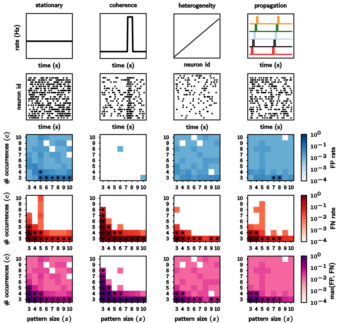
Fig. 4. Performance of 3d-SPADE in terms of FN and FP rates for four types of artificial data sets. Top row: rate models for the background activity. From left to right: stationary constant firing rate (25 Hz) for all neurons, coherent rate changes of all neurons, rate heterogeneity across neurons, and rate jump propagation across successive groups of neurons. Second row: corresponding raster plots. Third and fourth row: FP and FN rates, respectively, obtained by injecting 50 ms-long patterns of fixed size z (horizontal axis) and number of occurrences c (vertical axis) into the background data. Bottom: maximum of FP and FN rate per signature. Black circles indicate entries in the matrices where the FP or FN rate is over 0.05 (arbitrary threshold). The code to reproduce this figure can be found at https://github.com/INM-6/SPADE_applications/tree/master/validation_FPFN/code . To run the complete analysis (from generation of the artificial data, performing the SPADE analysis up to plotting this figure) execute the Snakefile contained therein.
