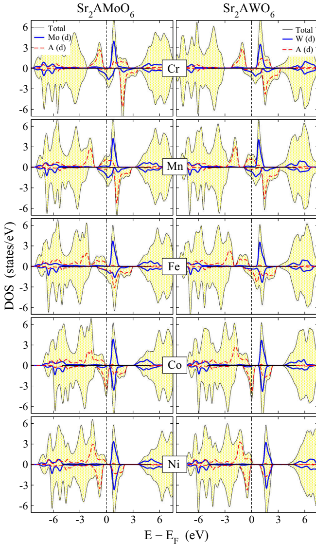
FIG. 4. Spin-polarized density of states (DOS) calculated by DFT-GGA for the double-perovskite series. Each panel shows the total DOS (black lines), the DOS projected onto the A-site cation (dashed red lines), and the DOS projected onto Mo or W (thick blue lines). The Fermi energy is set to zero.
