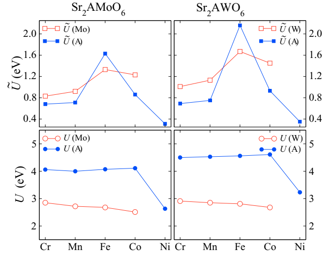
FIG. 5. RPA and cRPA results for the double-perovskite series. The values of the partially screened interaction U (bottom) and the fully screened interaction \tilde{U} (top) for both the A and B sites are presented.
