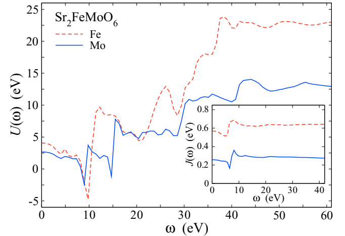
FIG. 6. Frequency dependence of U and J (inset) for Fe 3d and Mo t_{2g} electrons in paramagnetic \text{Sr}_2\text{FeMoO}_6 .
