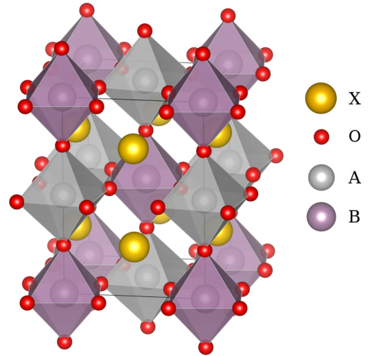
FIG. 1. Cubic double-perovskite structure for the general formula X_2\text{ABO}_6 used in this work.
