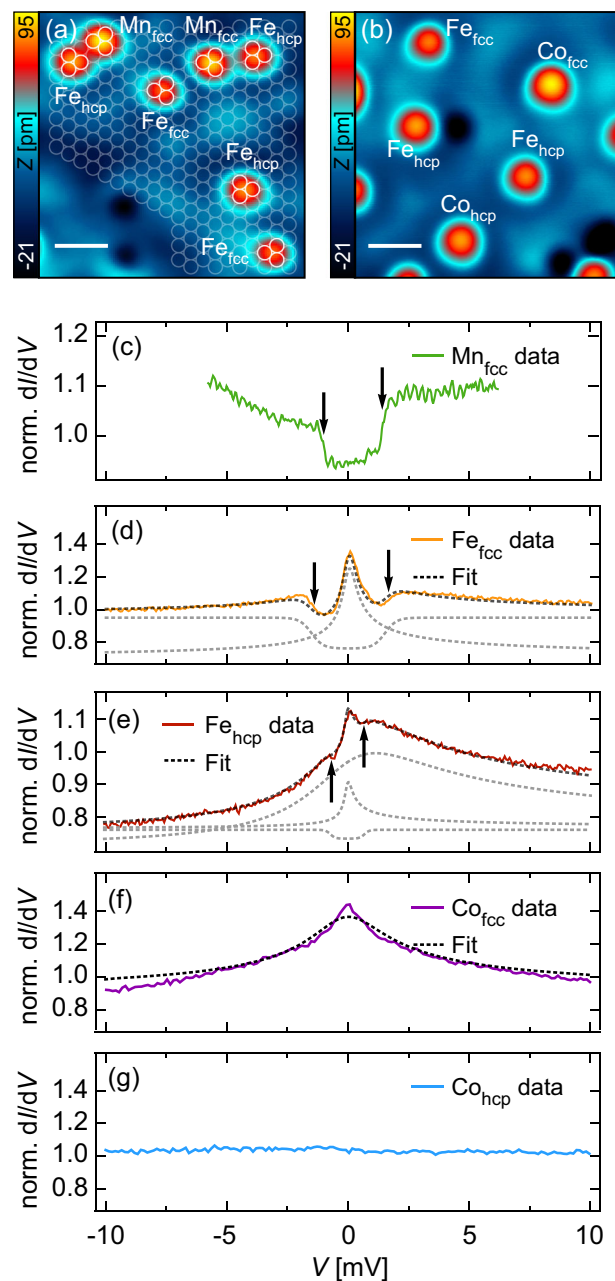
Fig. 1 Topographic and spectroscopic signatures of the 3d transition metal atoms. a Constant-current STM image of Mn and Fe atoms on different adsorption sites as indicated. The lattice of surface Re atoms determined from atom-manipulation images is overlaid (white circles). b Constant-current STM image of Co and Fe atoms on different adsorption sites as indicated (Scale bars in a , b have a length of 1 nm, V = 6 mV, I = 200 pA). c–g Tunnel spectra taken in the normal metal state of the substrate ( B_z = 50 mT). Normalized tunnel spectra taken on (c) \text{Mn}_{\text{fcc}} ( V_{\text{stab}} = -6 mV, I_{\text{stab}} = 3 nA, V_{\text{mod}} = 100 \mu V), (d) \text{Fe}_{\text{fcc}} , (e) \text{Fe}_{\text{hcp}} , (f) \text{Co}_{\text{fcc}} and (g) \text{Co}_{\text{hcp}} ( V_{\text{stab}} = 20 mV, I_{\text{stab}} = 3 nA, V_{\text{mod}} = 40 \mu V). For Fe, the black dashed lines are fits to the sum of Frota functions, and broadened step functions at the positions indicated by the black arrows (see the different contributions indicated by gray dashed lines shifted vertically for clarity). For \text{Co}_{\text{fcc}} , the black dashed line is a fit to a Frota function
