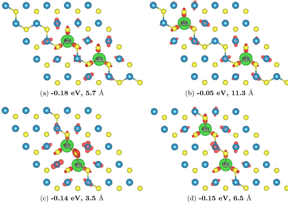
FIG. 3. Spin density isosurface distributions for 8%-Mn-doped \text{MoS}_2 in 5 \times 5 \times 1 supercells. The upper supercells contain each two Mn atoms in two armchair positions while the lower supercells contain each two Mn atoms in two zigzag positions. The energy differences between the AFM and FM coupling states ( \Delta E ) and Mn-Mn distances are listed for each configuration. The green and red isosurfaces represent positive and negative spin density, respectively. The iso-surface value is 0.015 \text{ e}\text{\AA}^{-3} .
