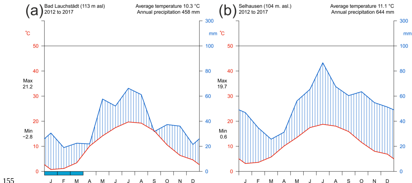
Figure 1: Climate diagrams according to Walter and Lieth (1967) for Bad Lauchstädt (a), and Selhausen (b) for 2012 to 2017. Data were obtained from the SOILCan weather stations at Selhausen and a climate station at Bad Lauchstädt above sea level (asl.). The blue bars at the bottom of subplot a) indicate months where frost is likely to occur.
