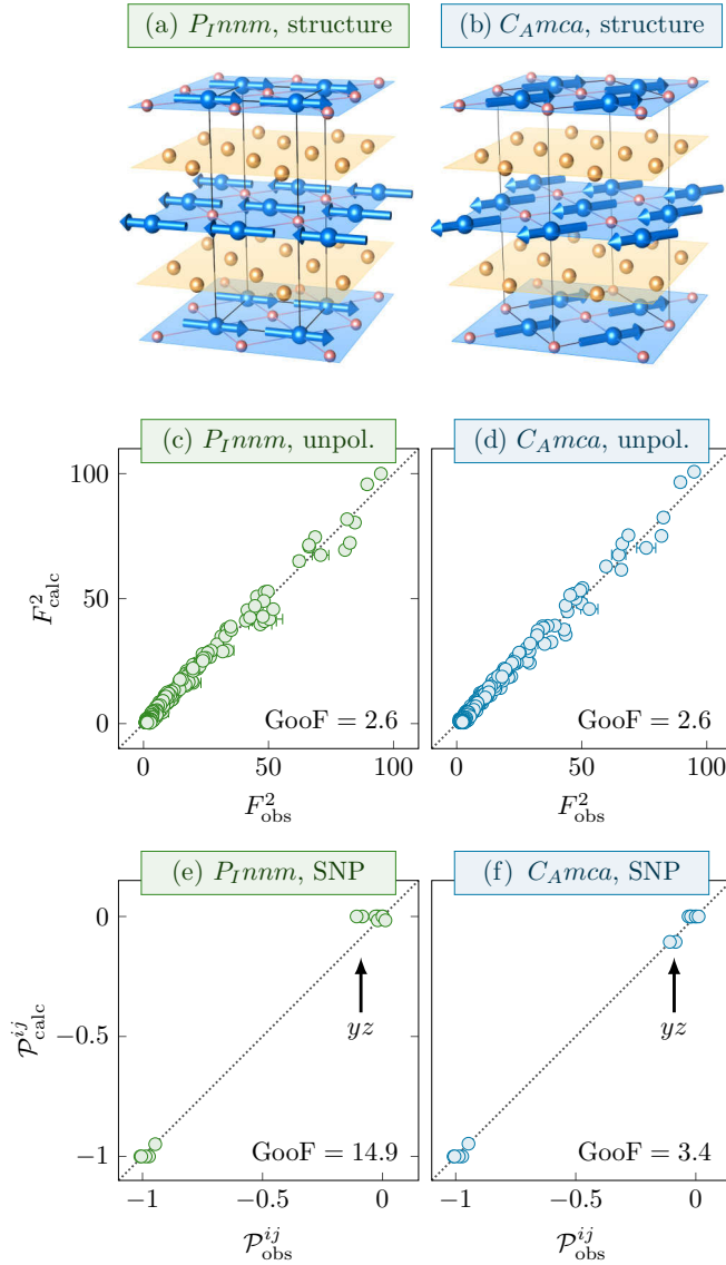
FIG. 5. Magnetic structure of \text{HoNi}_2\text{B}_2\text{C} in (a) MSG P_{1nnm} and (b) MSG C_{Amca} . Boron atoms are not shown for simplicity. Quality of the unpolarized neutron diffraction data refinement at 2.4 K in (c) MSG P_{1nnm} and (d) MSG C_{Amca} . The experimental structure factors squared F_{\text{obs}}^2 are plotted against the calculated ones F_{\text{calc}}^2 . The quality of the spherical neutron polarimetry data refinement at 3.9 K is shown in (e) MSG P_{1nnm} and (f) MSG C_{Amca} . The experimental polarization matrix elements \mathcal{P}_{\text{obs}}^{ij} are plotted against the calculated ones \mathcal{P}_{\text{calc}}^{ij} .
