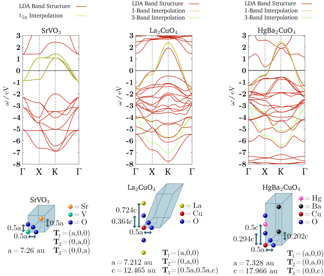
FIG. 13. LDA Band structures ( \mu at 0) and crystal structure data of \text{SrVO}_3 , LCO, and HBCO. \Gamma = (0, 0, 0) , X = (\pi/a, 0, 0) , and K = (\pi/a, \pi/a, 0) .
