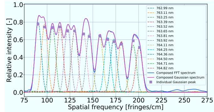
(a) Gaussian fitted spectrum with dense components
