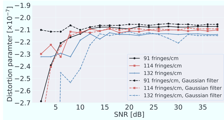
Figure 3.5: Parameter estimation results for interferograms with different spatial frequencies with respect to SNR (dB). The dashed lines represent the results with Gaussian filter for noise reduction before edge detection.
