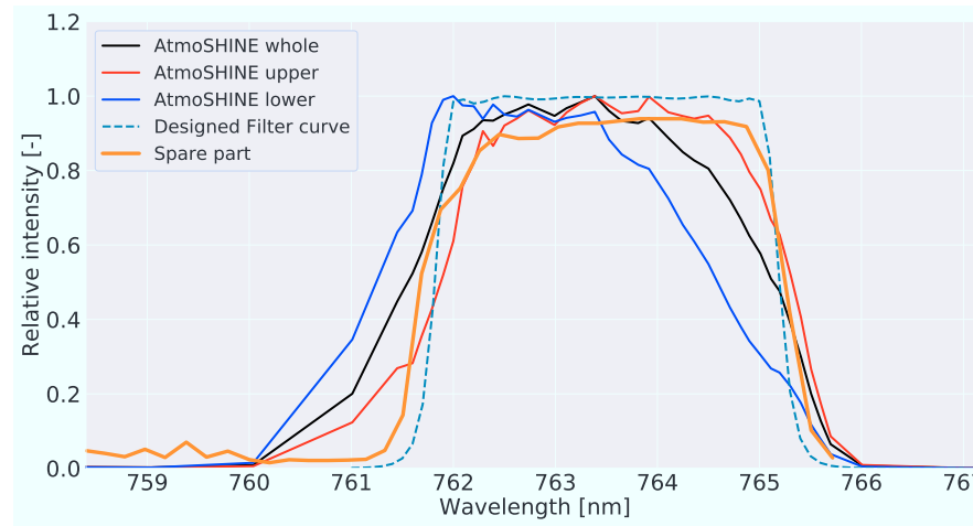
Figure A.3: Filter response functions characterized using different regions of the interferograms for AtmoSHINE instrument. Response curve marked with “AtmoSHINE whole” uses 840 \times 840 pixels in the interferogram center region. “AtmoSHINE upper” and “AtmoSHINE lower” takes 100 \times 100 pixels with the same readout column in “AtmoSHINE whole” while starting from row 200 and row 600, respectively. The curve labeled with “spare part” shows the response curve of another filter sample manufactured in the same batch process. A theory curve provided by the manufacturer is also plotted in the dashed curve.
