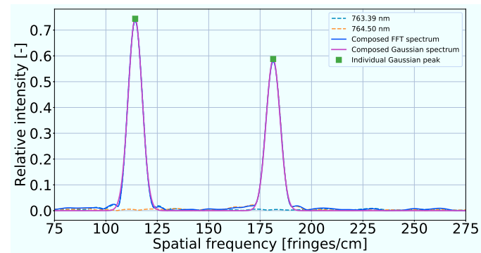
(c) Gaussian fitted spectrum with two components
