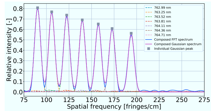
(b) Gaussian fitted spectrum with sparse components
