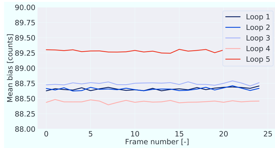
(a) Mean value of detector fixed pattern
