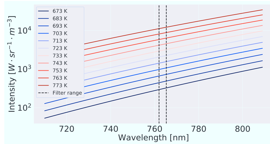
Figure 5.1: Spectral radiance estimated from an ideal blackbody at different temperatures, the dashed lines represent the optical filter range.
