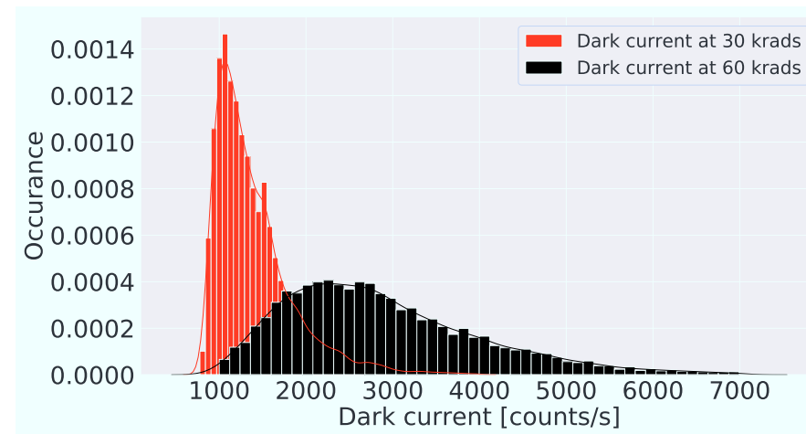
Figure 2.10: Detector dark current histograms measured under manual calibration mode with 30 krad and 60 krad radiation. An image area of 600x600 pixels are chosen starting from row 200 and column 200.
