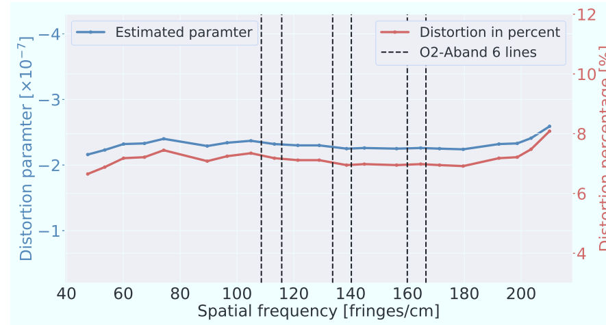
Figure 5.7: Estimated distortion parameters from the interferograms generated between 762.29 nm and 765.01 nm. Dashed lines represent the corresponding spatial frequency of 6 O 2 A-band emission lines for the temperature retrieval.
