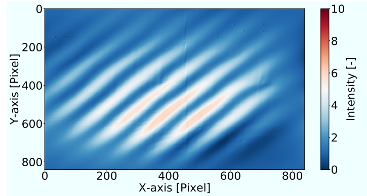
(b) Interferogram after ghost removal
