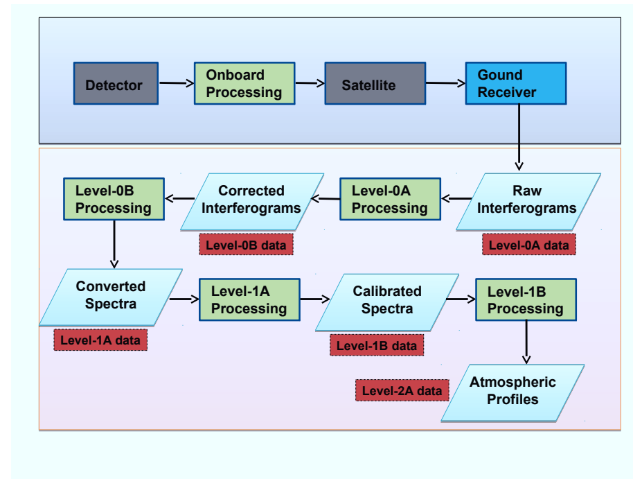
Figure 1.7: AtmoSHINE data processing chain from Level-0 to Level-2. Upper colored region indicates the processing on the satellite part, lower colored region includes the processing on ground.
