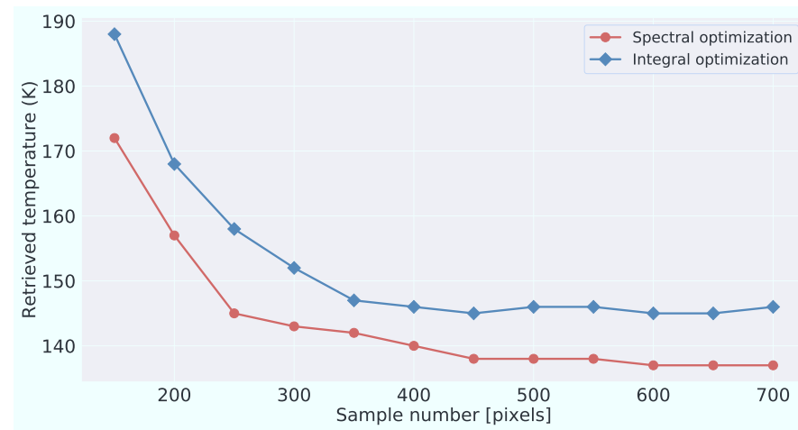
Figure 6.13: Temperature retrieval results with different number of samples for the Fourier analysis. The sampled pixels are picked around the image center.
