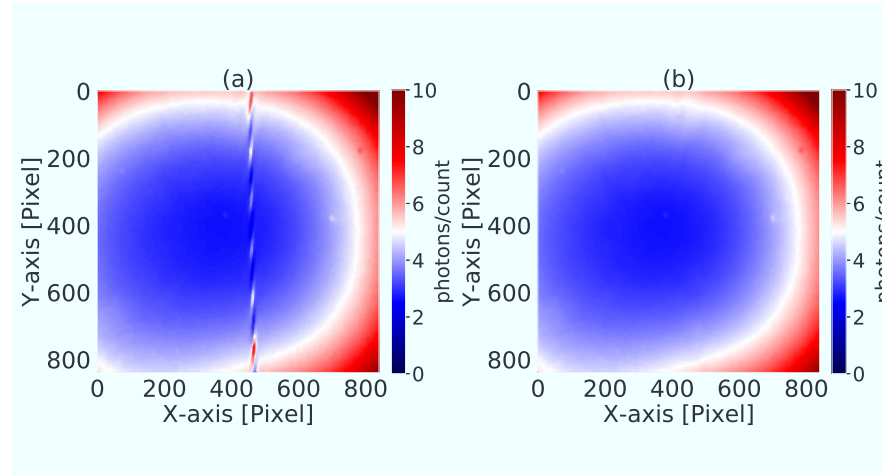
Figure 6.6: (a): Radiometric measurement from the Blackbody emission characterized on ground. (b): Corrected radiometric response matrix, the zero-order interference regions are replaced by a series of interpolated points with polynomial approximation for each row.
