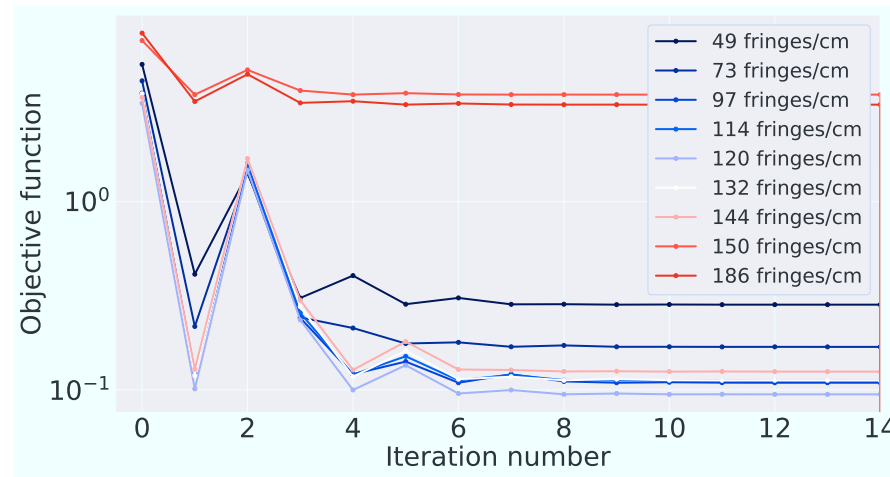
Figure 3.6: The convergence rates of the optimization algorithms using Golden section search method. Interferograms with wavelengths between 762.6 nm (49 fringes/cm) and 764.9 nm (186 fringes/cm) are used for the estimation.
