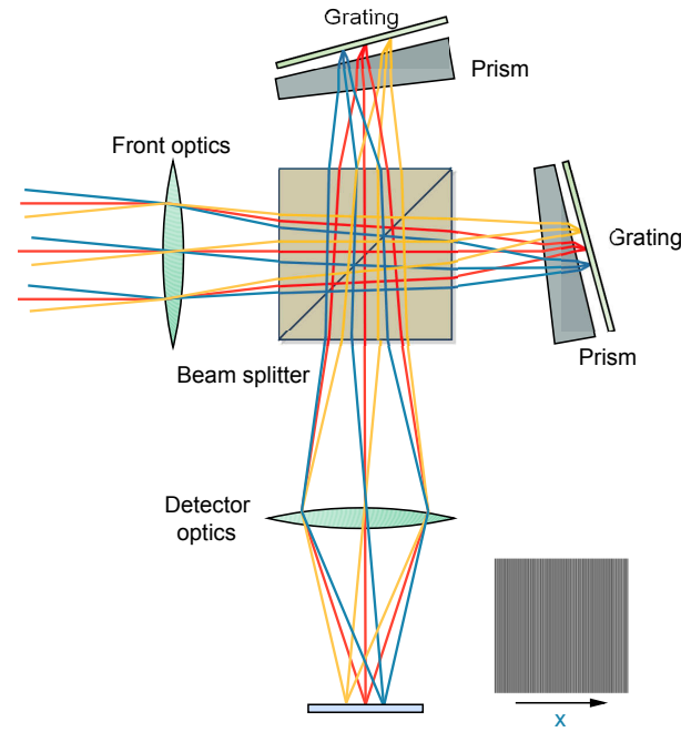
Figure 1.6: Schematic of a field-widened SHS concept in focused configuration.
