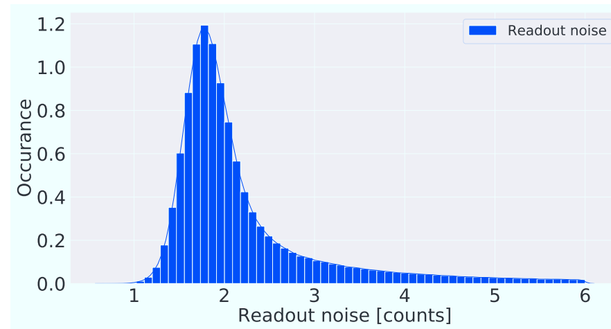
Figure 2.5: Detector readout noise estimation based on multiple frames readout under 1ms integration time. The detector was cooled down to -20^{\circ}\text{C} in the thermal chamber.
