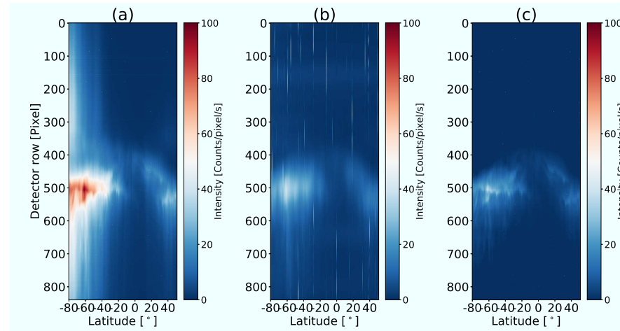
Figure A.1: Row-wise emission intensity measured at different satellite latitudes. The detector offsets are removed. Negative/positive latitude values correspond to the south/north hemisphere. Detector row 0 represents the upper altitude region, row 800 represents the lower altitude region. (a): Total emission intensity. (b): Emissions between 762.2 nm and 765.0 nm. (c): Emissions from other side of the Littrow wavelength ( <761.2 nm).
