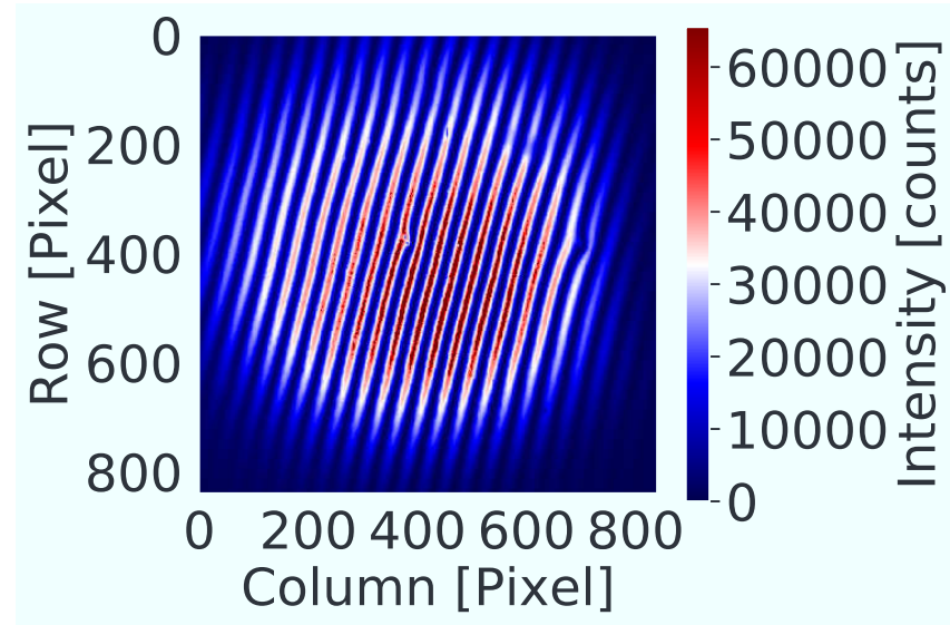
Figure 5.6: Raw interferogram containing 840x840 pixels at 762.39 nm.
