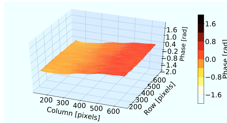
(b) Phase map with image correction
