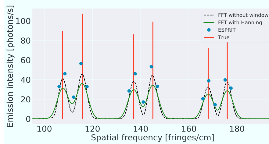
Figure 4.10: Converted spectra with one wavenumber broadening interferogram containing 800 pixels at SNR=20. The spectrum (green line) obtained from the Hanning windowed interferogram does not contain the correction using the corresponding scaling factor. For the subspace method (blue dots), 15 emission lines are assumed as the a prior information.
