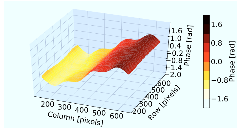
(a) Phase map without image correction
