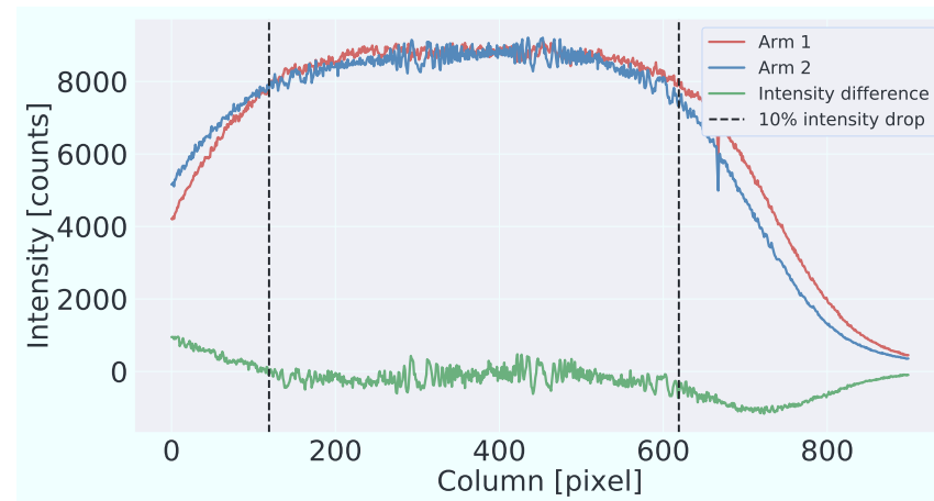
Figure 5.5: Intensity of two arms at row 450. Dashed lines indicate the edges where the intensity drop to 90% of the highest value. The relative intensity is about 51% and 49% for two arms within the dashed region. Green curve indicates the intensity difference between two arms.
