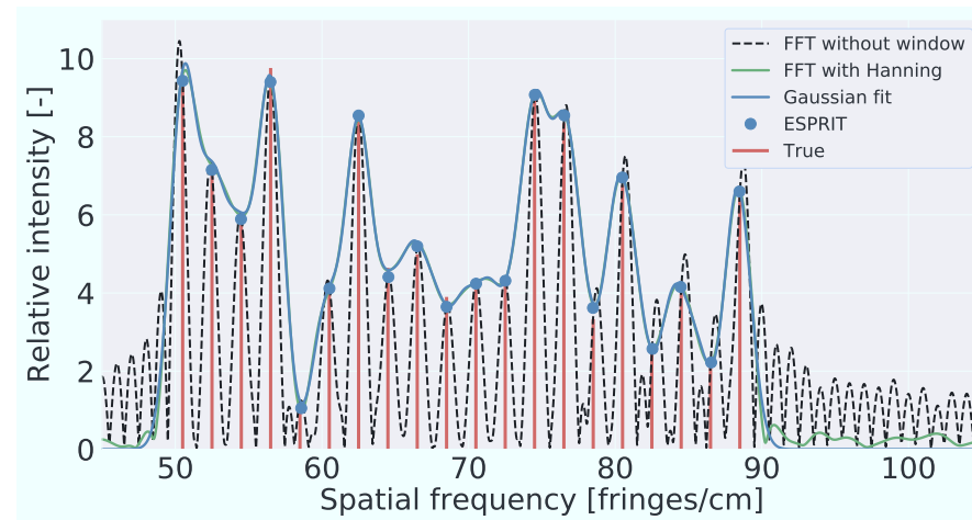
Figure 4.7: Reconstructed spectra using different methods in comparison with the input spectral intensity containing 20 well spaced components. The amplitude of each signal component is randomly generated between 1 and 10. The SNR in spatial domain is 100 and the sampling length is 500 pixels. Blue lines indicate a fitted spectrum using Gaussian mixture method with determined frequency information. Blue dots represent the amplitudes estimated from the ESPRIT method.
