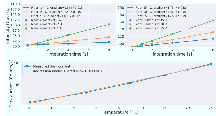
Figure 2.3: Upper plots: measured signal intensity between -14^{\circ}\text{C} and 25^{\circ}\text{C} under different integration time. Lower plot: temperature dependency of the detector dark current and the corresponding exponential fit, based on the gradients obtained in upper subplots.
