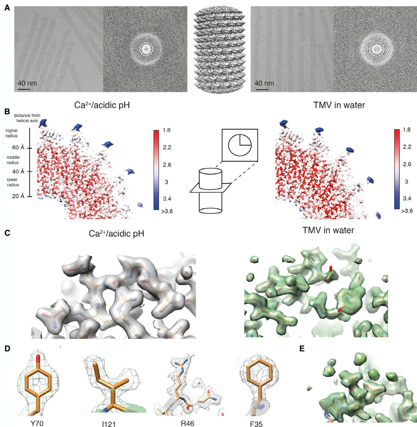
Figure 1. High-resolution cryo-EM structures of tobacco mosaic virus (TMV) in conditions of \text{Ca}^{2+} /acidic pH (gray, left) and water (green, right).
